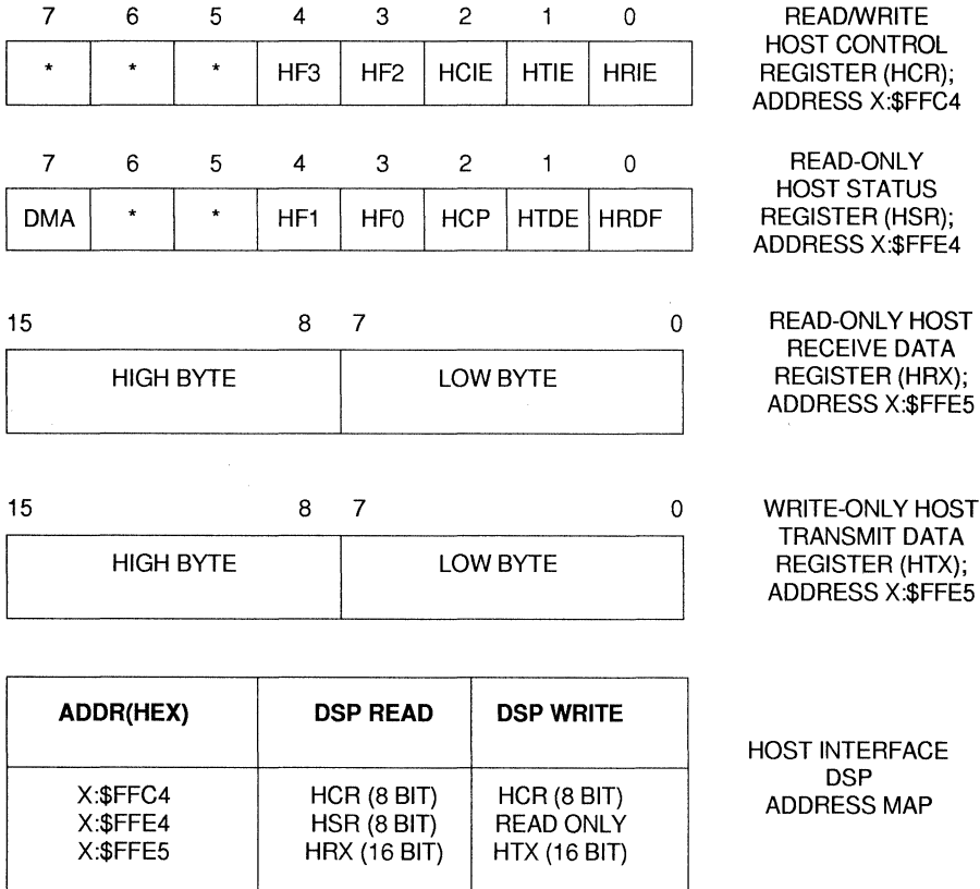
Figure 5-2 Host Interface — DSP Programming Model
