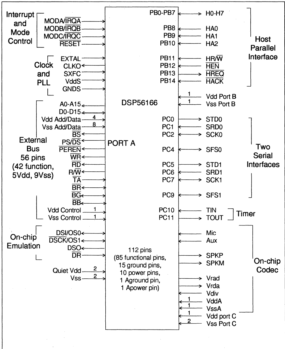
Figure 2-1. DSP56166 Pinout
