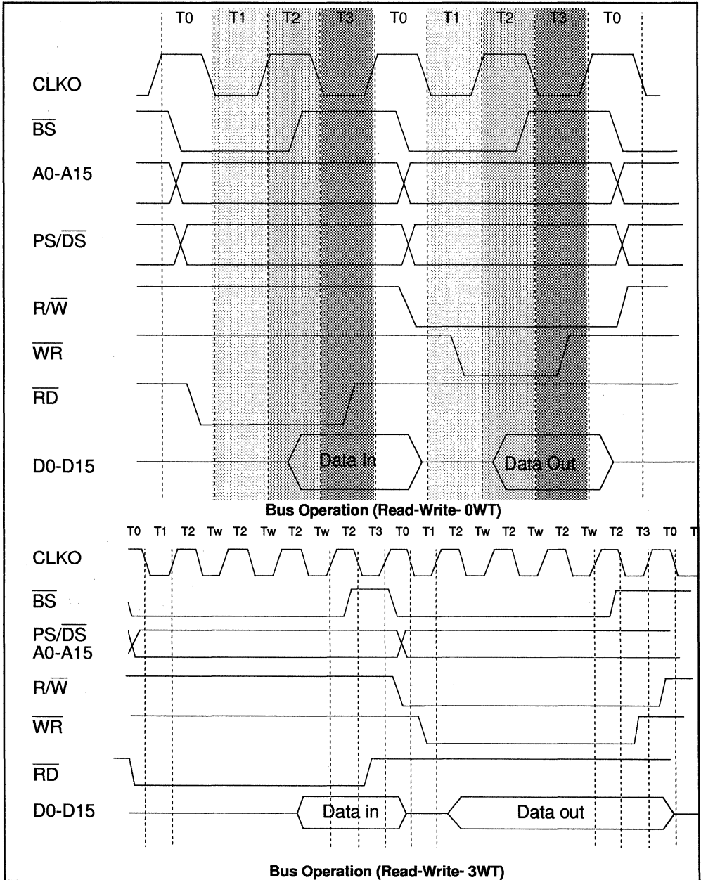
Figure 2-2 Bus Operations
