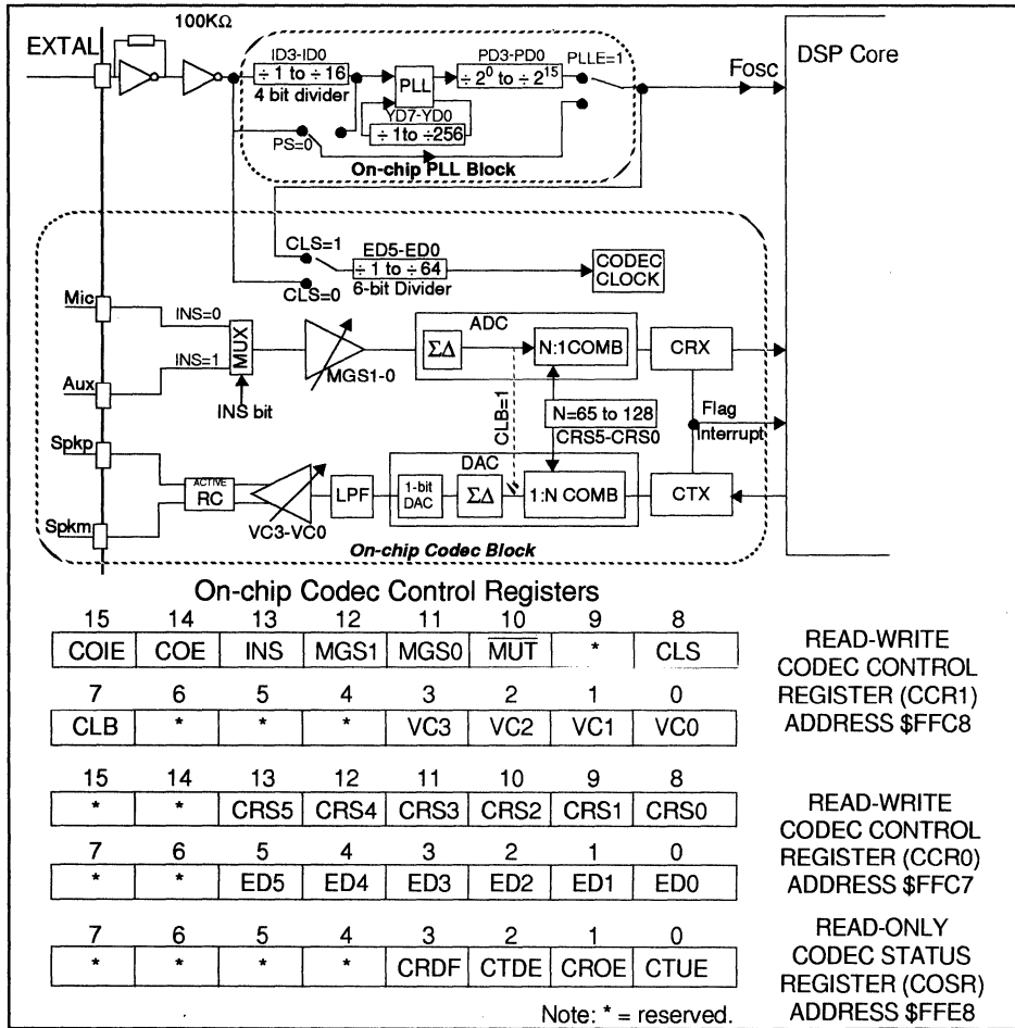
Figure 6-2 DSP56166 Codec General Block Diagram
