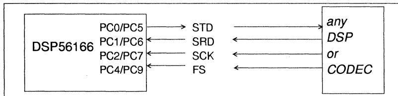
Figure 8-2 RSSI External Continuous Clock
