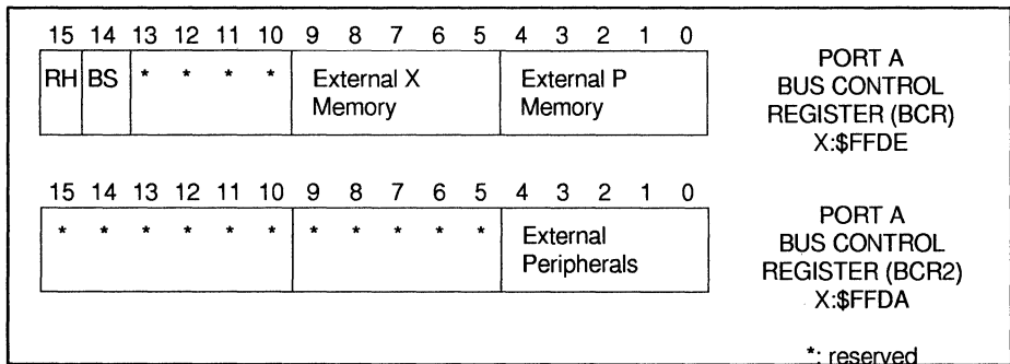
Figure 3-1 External Peripheral Bus Control Register (BCR2)
