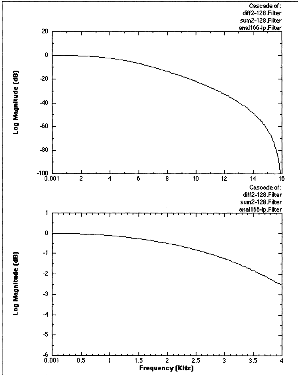
Figure 6-16 Log Magnitude Frequency Response of the D/A Section for F=2.048 MHz and D=128
