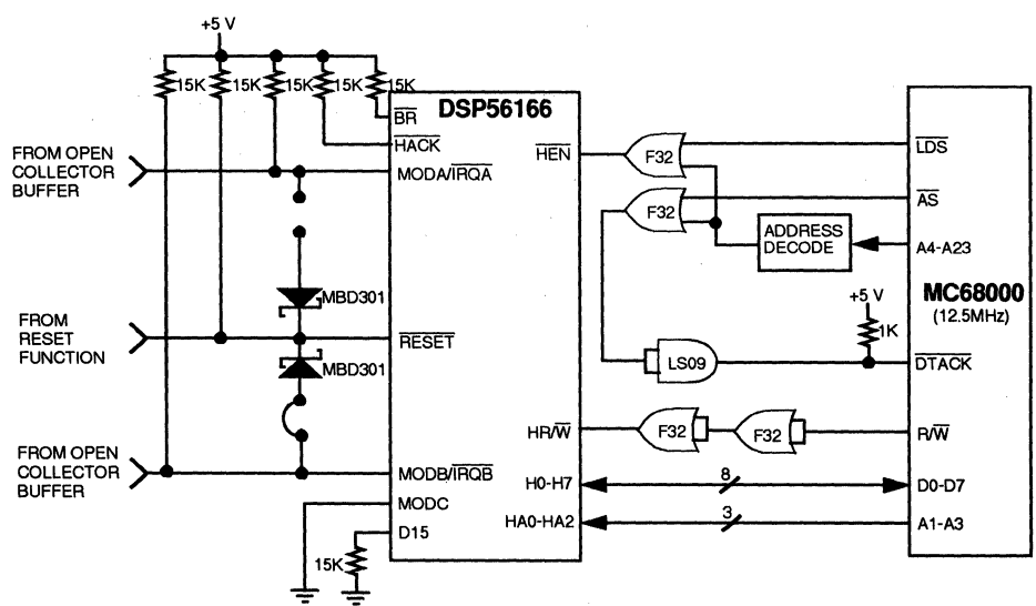
Figure B-2 DSP56166 Host Bootstrap Example — Mode 1
