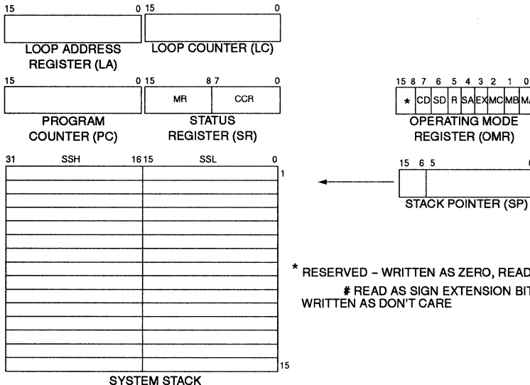
Figure 1-8 Programing Model
