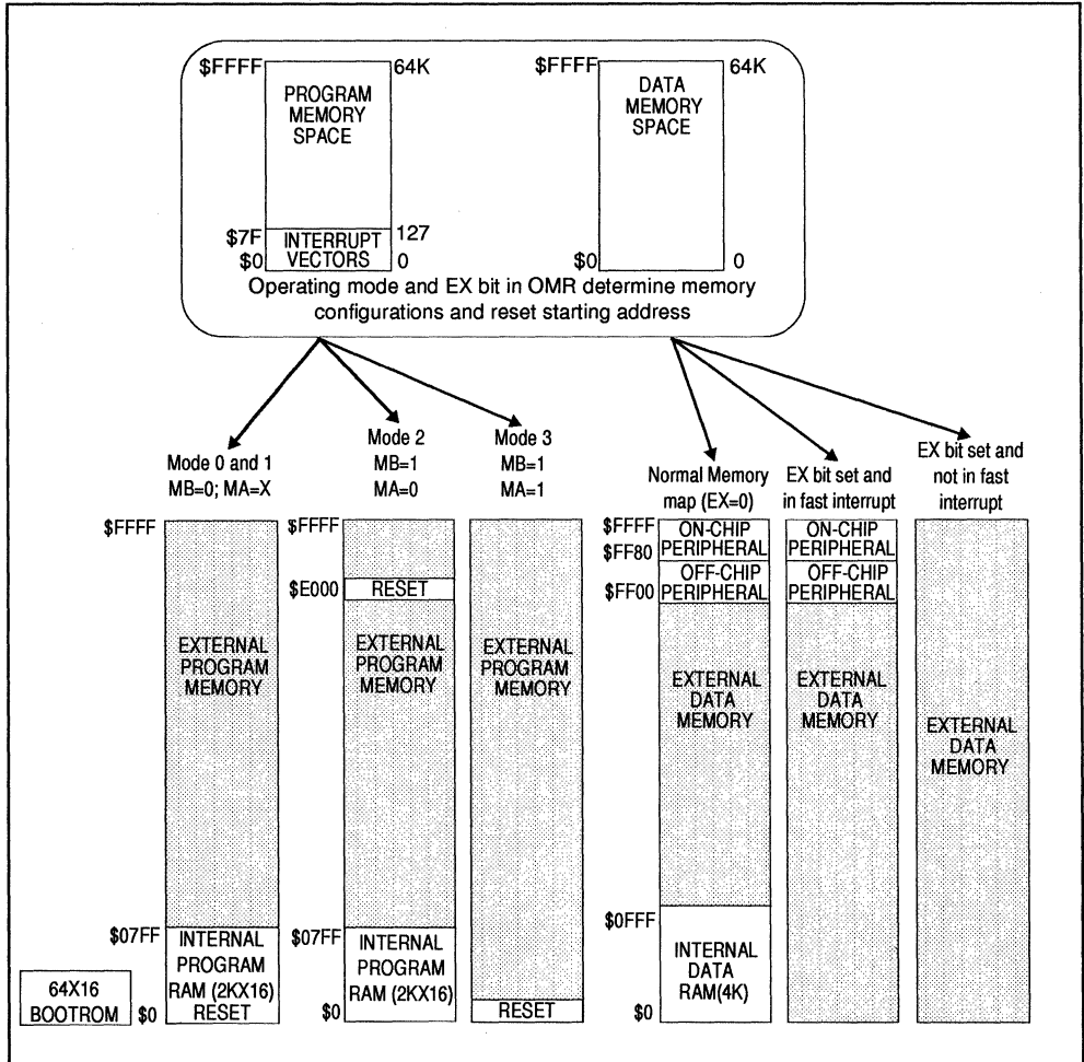
Figure 3-2 DSP56166 RAM based Memory Map
