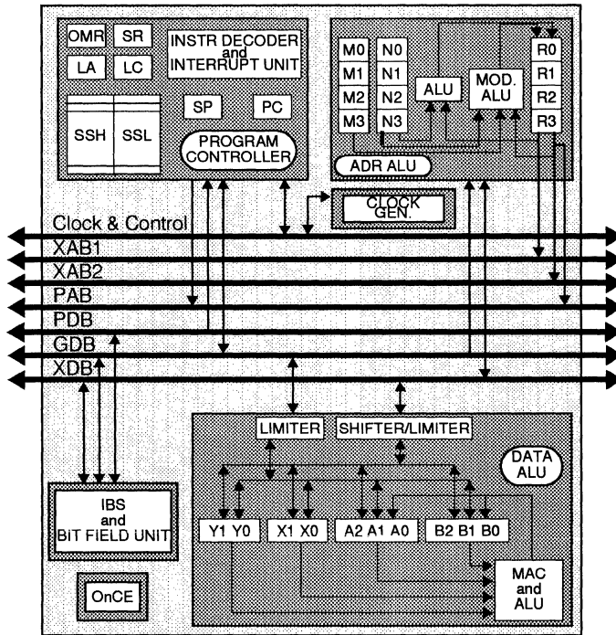
Figure 1-4 DSP5616 Core Block Diagram
