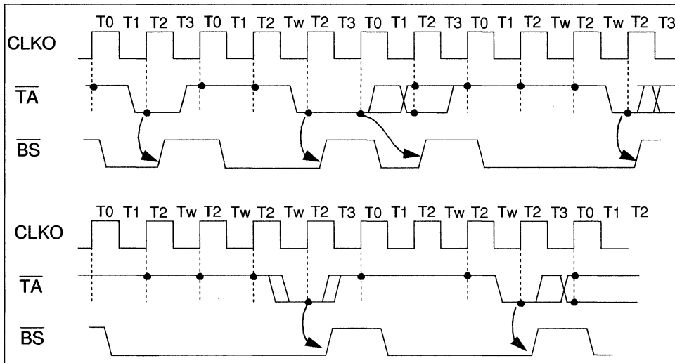
Figure 2-3 \overline{TA} Controlled Accesses
