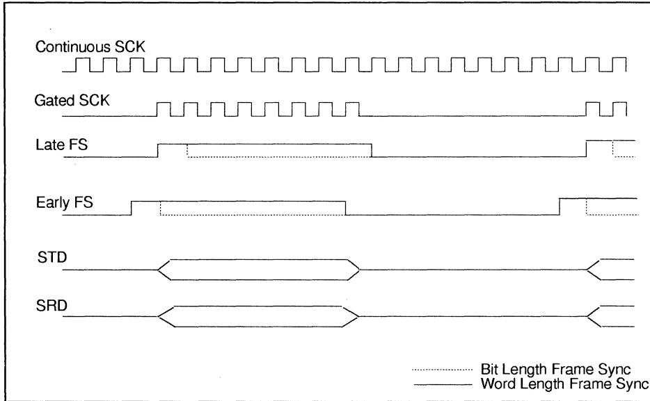
Figure 8-7 Serial Clock and Frame Sync Timing
