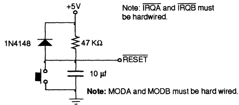
Figure B-4 Reset Circuit
