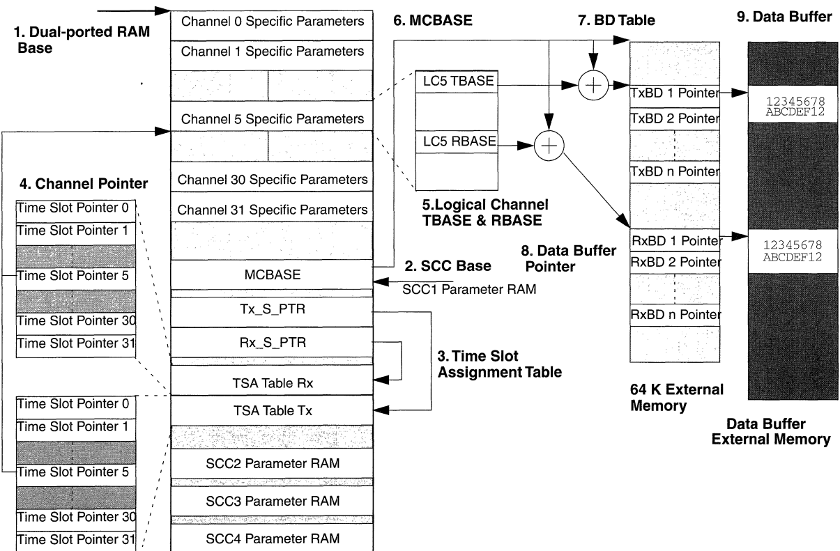
Figure 2-2. QMC Memory Structure
