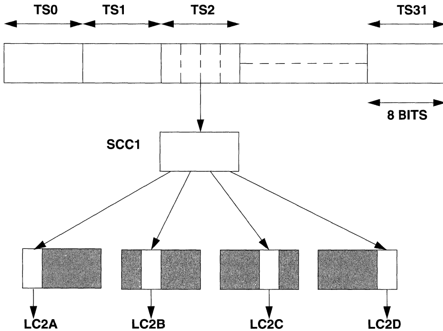
Figure 9-2. Two-Bit Subchannel Implementation with MSC Microcode
