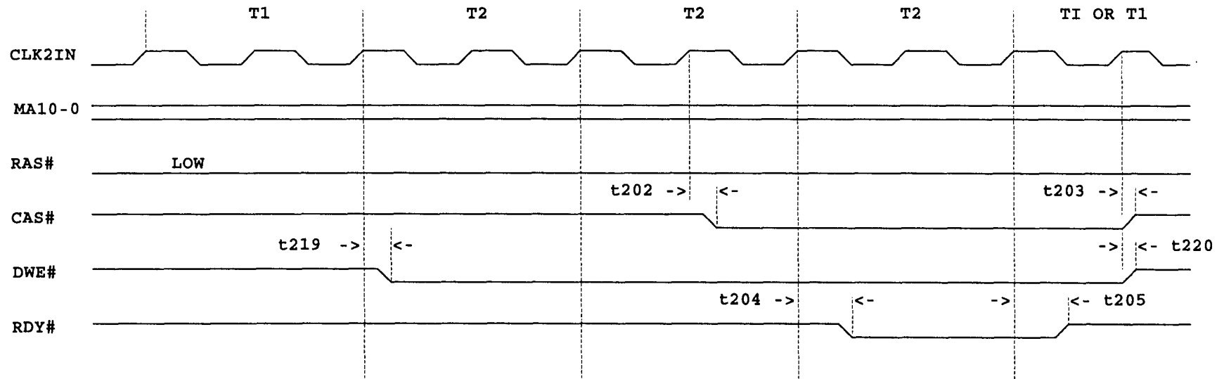
WRITE CYCLE, PAGE HIT, 2 WAIT STATES
