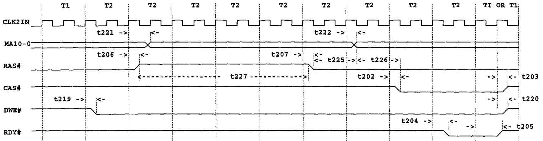
WRITE = 2 WS, PAGE MISS (WITH READ = 4-3-3-3)
