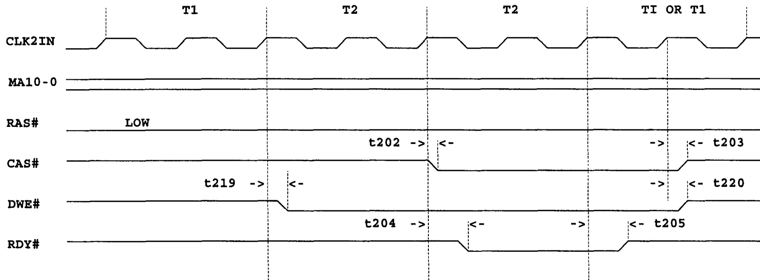
WRITE CYCLE, PAGE HIT, 1 WAIT STATE (OR READ = 4-3-3-3, WRITE = 1WS)
