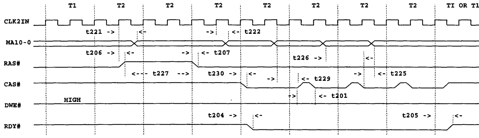
BURST READ 3-1-1-1, PAGE MISS, RAS# ACTIVE IN PREVIOUS CYCLE
