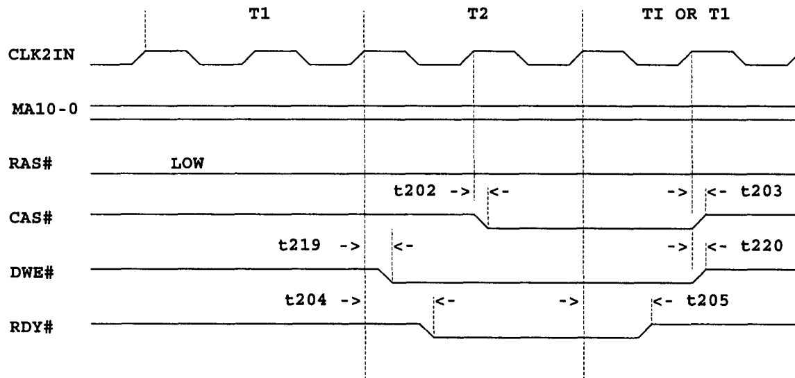
WRITE CYCLE, PAGE HIT, 0 WAIT STATE
