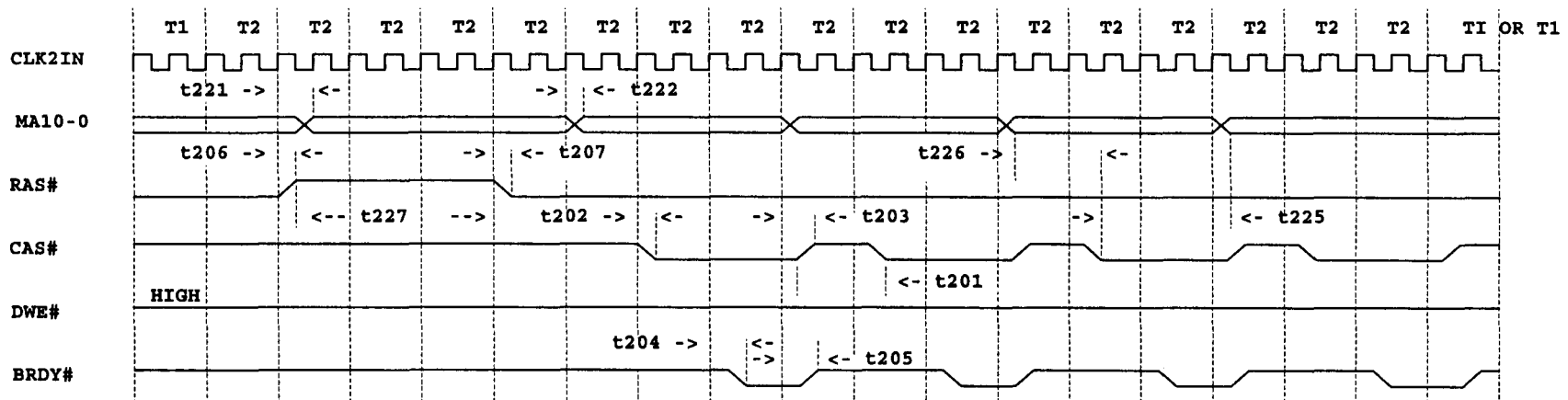
BURST READ 4-3-3-3, PAGE MISS, RAS# ACTIVE IN PREVIOUS CYCLE
