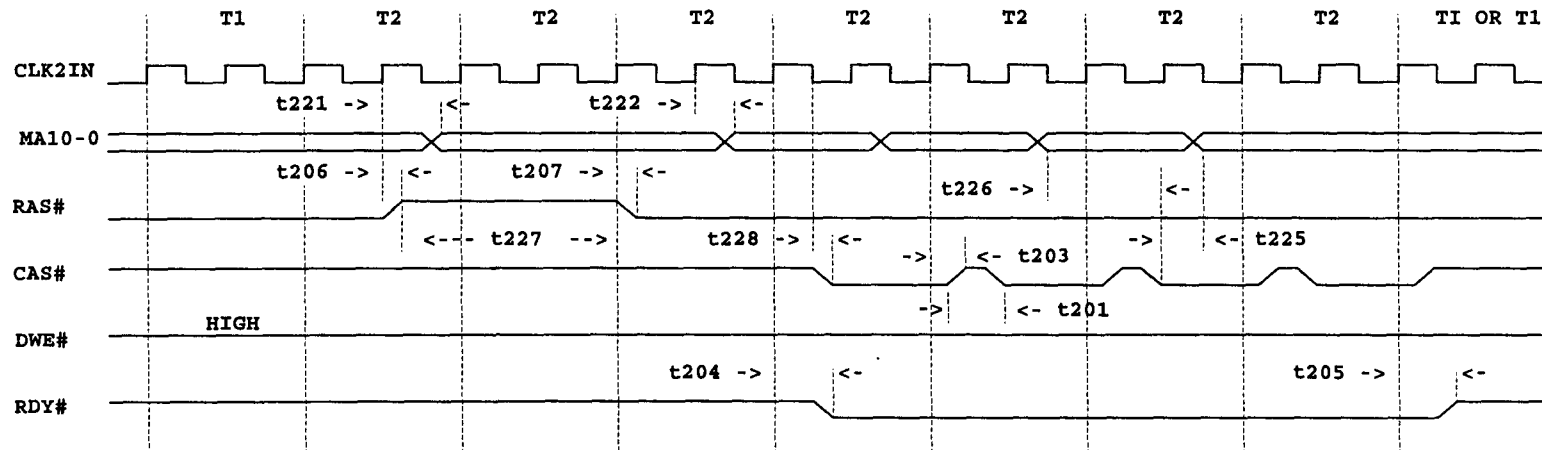
BURST READ 2-1-1-1, PAGE MISS, RAS# ACTIVE IN PREVIOUS CYCLE
