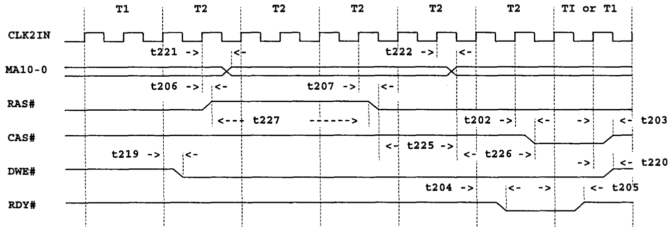
WRITE = 0 OR 1 WS, PAGE MISS (WITH READ = 3-2-2-2)
