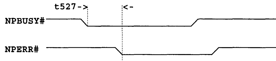
NPBUSY, FERR# TIMING
