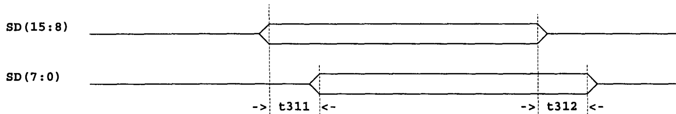
DATA VALID AND INVALID DELAY BETWEEN SD(15:8) AND SD(7:0) SWAPPING
