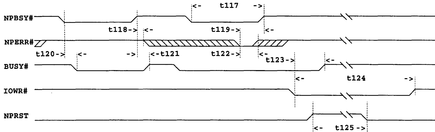
387 NUMERICAL PROCESSOR RESET TIMING
