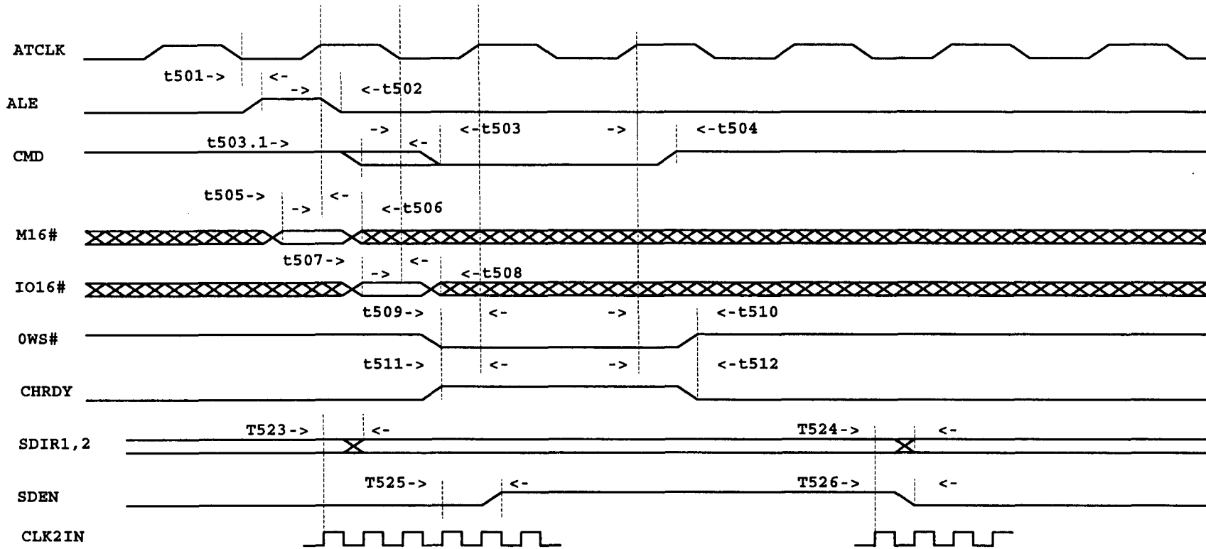
ATBUS TIMINGS
