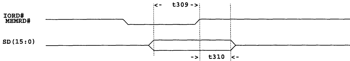
DATA SETUP AND HOLD TIME FOR IORD# AND MEMRD#
