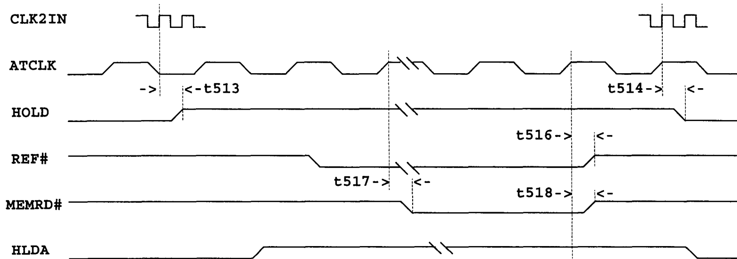
ATBUS HOLD TIMING
