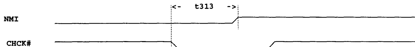
NMI VALID DELAY RELATED TO CHCK#
