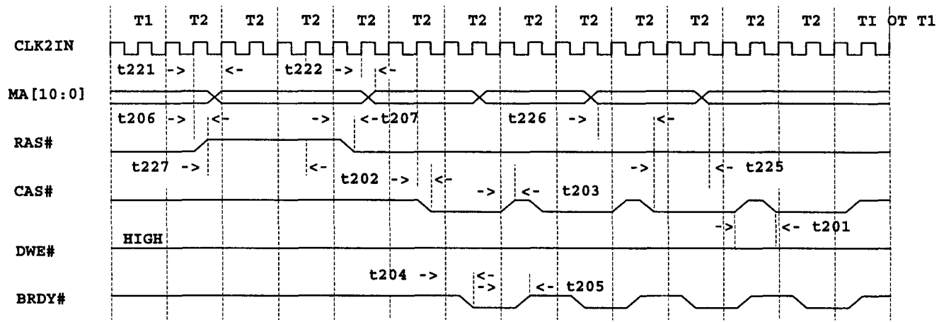
BURST READ 3-2-2-2, PAGE MISS, RAS# ACTIVE IN PREVIOUS CYCLE
