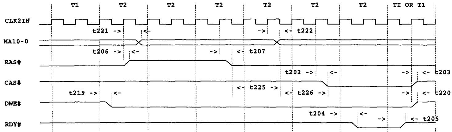
WRITE = 2 WS, PAGE MISS (WITH READ = 3-2-2-2)
