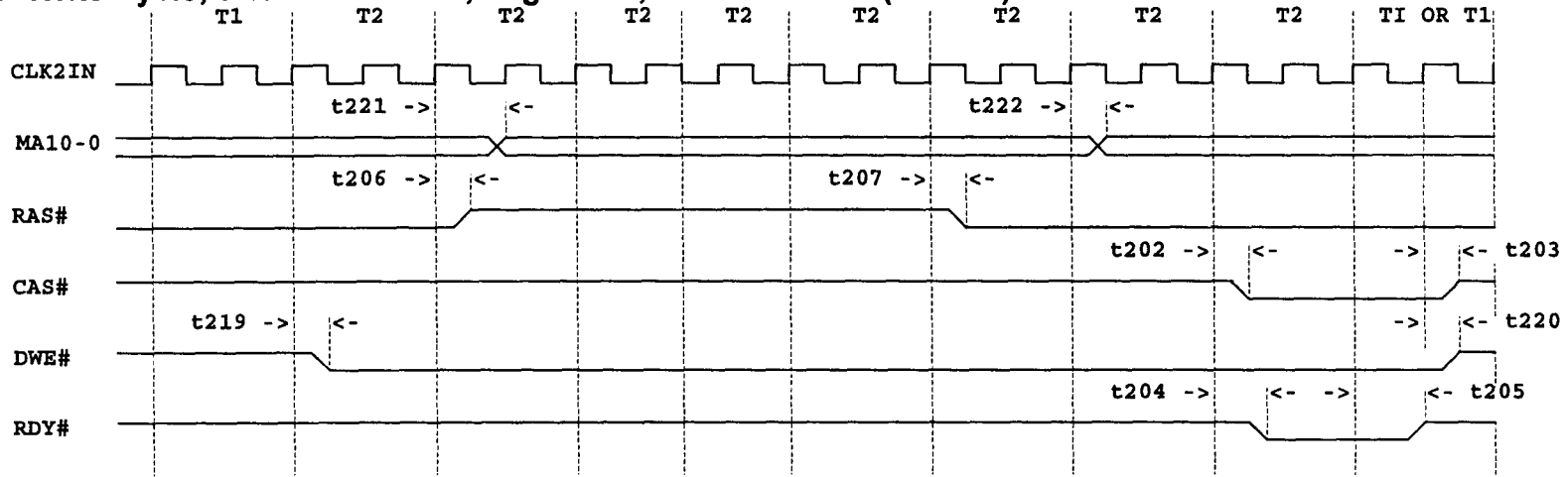
WRITE = 0 OR 1 WS, PAGE MISS (WITH READ = 4-3-3-3)
