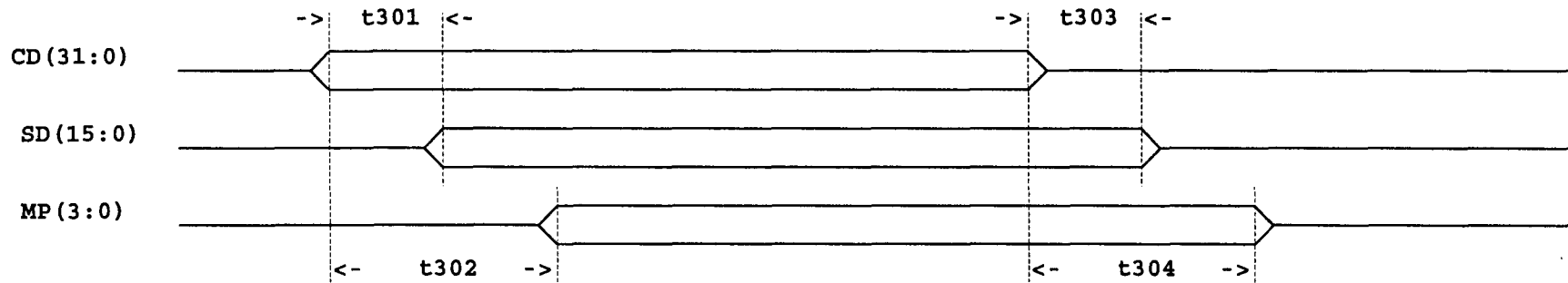
CD(31:0) TO SD(15:0) & MP(3:0) VALID AND INVALID DELAY
