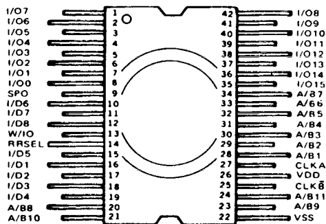
A17XX ROM/RAM/IO Pin Configurations
