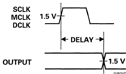
Figure 4-3. Output Timing
