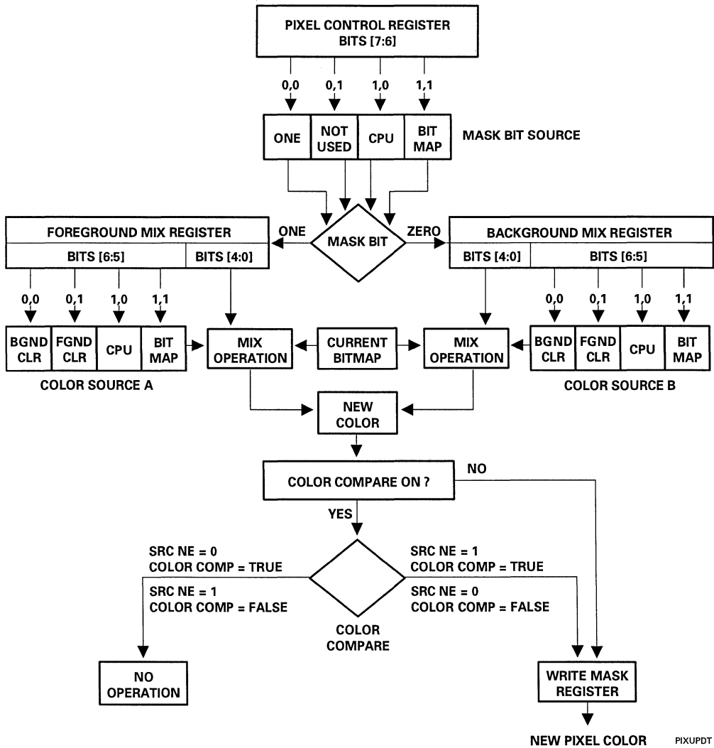
Figure 5-1. Pixel Update Flowchart
