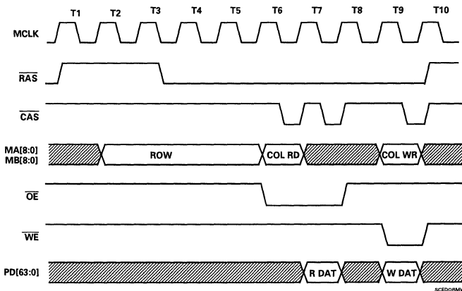
Figure 3-6. 1 Cycle EDO Read/Modify/Write Timing
