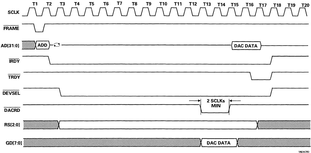
Figure 3-1. RAMDAC PCI Read Timing
