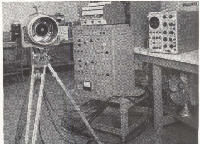
INFRARED CAMERA (left) showing adjustments (but not electronic circuits) and light sensitive camera back. Radiometer and electronic circuits (right) with recorder
