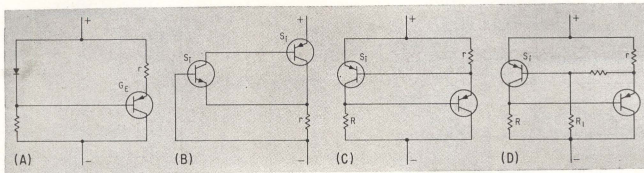
CIRCUIT OPERATES over narrow voltage range (A); ideal circuit using complementary transistors is impracticable (B); adaption of ideal circuits uses pnp transistors (C) and improved version has cancellation components added (D) —Fig. 1
