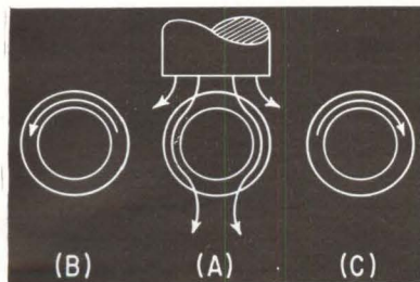
FLUX PATTERN in magnetically biased core—Fig. 1
