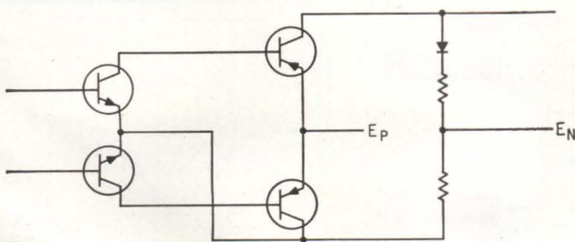
Single-ended amplifier, a simple variation of the circuit on p 38—Fig. 2
