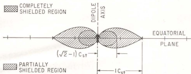
MAGNETIC DIPOLE field shielding regions
