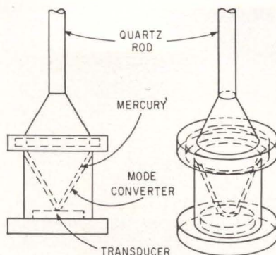
QUARTZ MODE converter is used to obtain Rayleigh waves—Fig. 3
