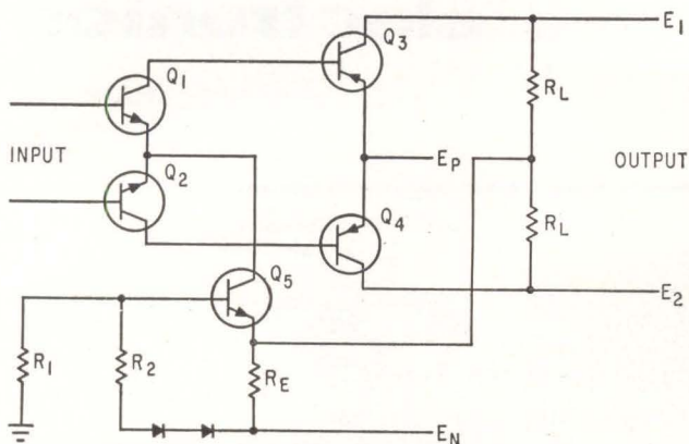
GENERAL PURPOSE amplifier. Circuit design, amplifier characteristics, and differential characteristics are analyzed for block production—Fig. 1
