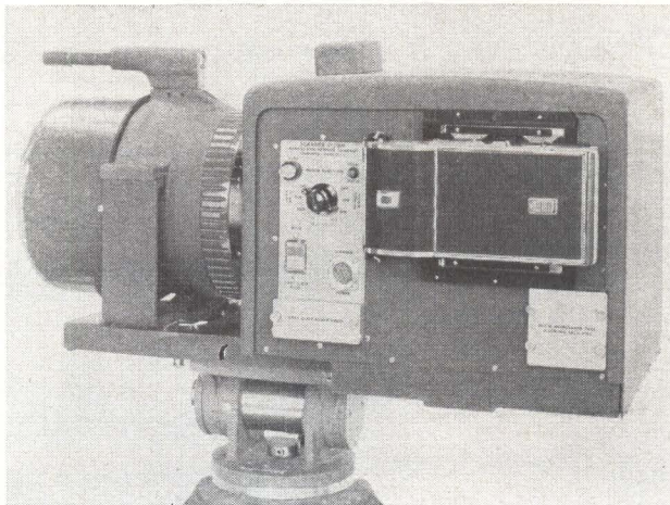
INFRARED CAMERA (left) showing adjustments (but not electronic circuits) and light sensitive camera back. Radiometer and electronic circuits (right) with recorder
