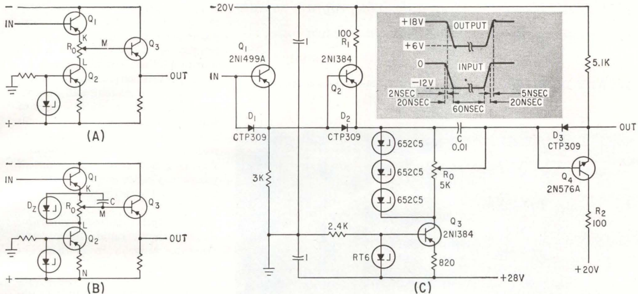
BASIC CONVERTER (A) is improved in (B) to reduce loss and improve h-f response. Final circuit (C) uses 5-percent tolerance resistors—Fig. 1
