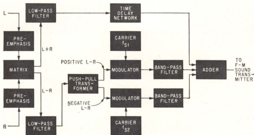
STEREO TV SOUND system employs three information channels. L+R signal can be received on unmodified sets
