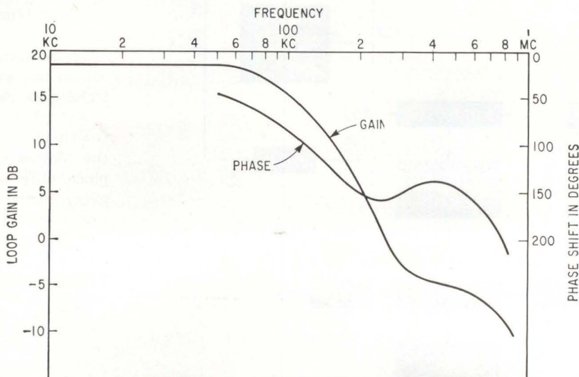
GAIN and phase response of the FMFB loop in terms of loop gain and frequency—Fig. 4
