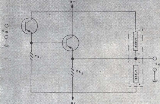
BOOTSTRAPPED EMITTER FOLLOWER WITH DUAL ISOPLY
