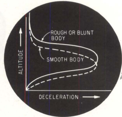
DECELERATION CURVES of re-entry bodies help identify decoys. First bend predicts rest of curve
