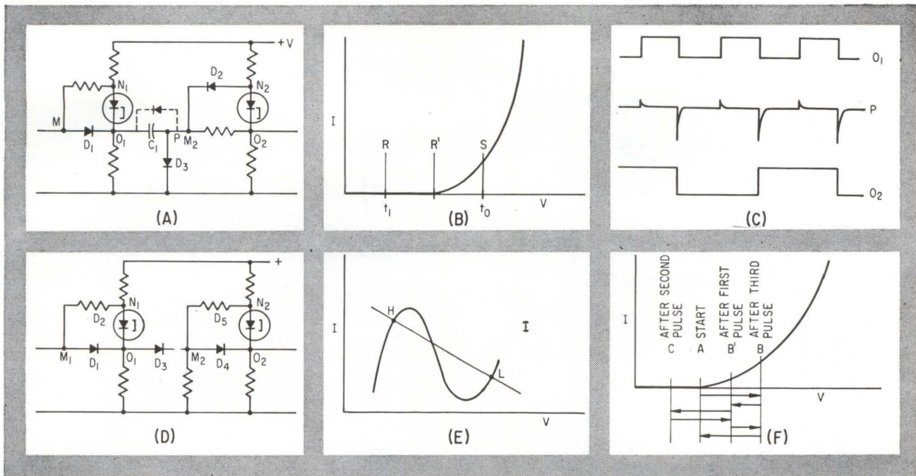
POSITIVE and negative-pulse-driven flip-flop (A) with diode curve (B) and internal waveshapes (C). A simpler coupling (D) with tunnel-diode curve (E) and diode curve (F)—Fig. 2
