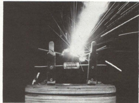
Here's a dramatic test of resistor reliability under extreme overload conditions. The effect of 120 volts on the molded unit is catastrophic in seconds; TI's hard-glass resistor can withstand it for days without damage.
