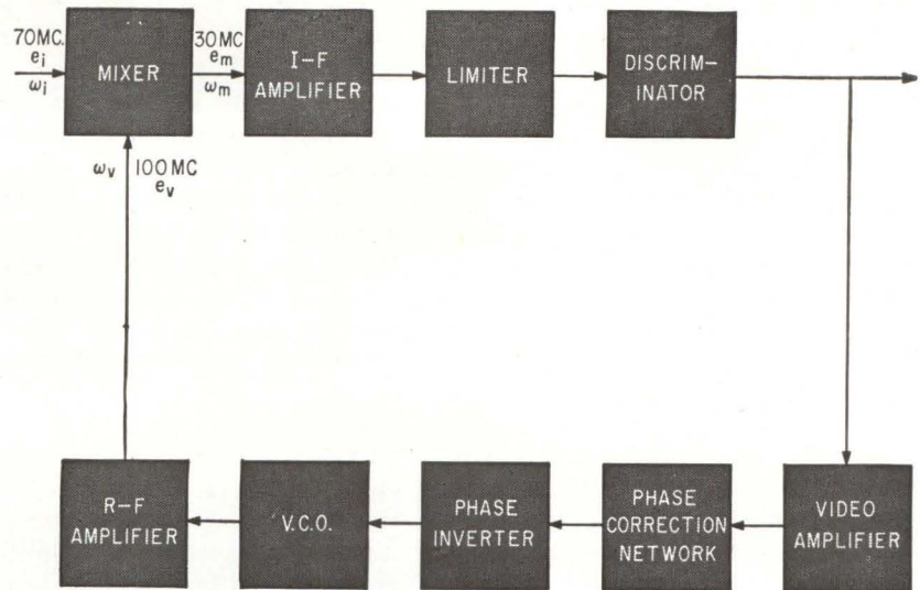
RECEIVER includes a voltage-controlled oscillator and phase-correction network — Fig. 1
