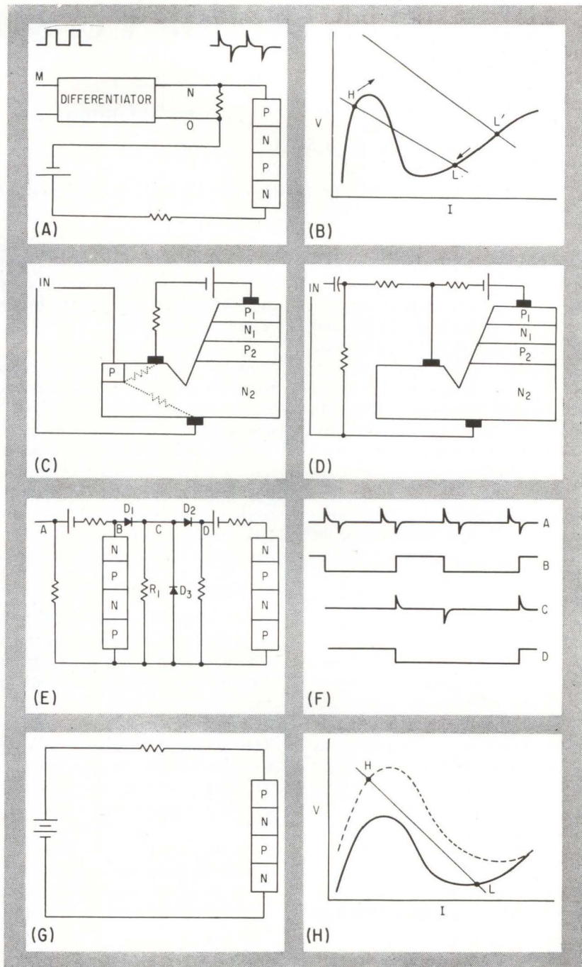
FOUR-LAYER diode basic flip-flop (A) with characteristic curve (B). Typical four-layer structure (C) can be part of circuit (D). Coupling pnpn diodes (E) use two differentiating circuits and produce waveshapes shown in (F). A low-frequency astable multivibrator (G) with its associated waveshapes (H)—Fig. 6
