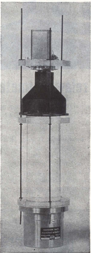
SPECTROMETER, showing scintillation detector that uses a single NaI crystal, with electronics mounted on top—Fig. 1
