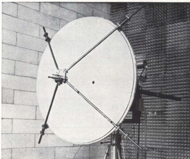
TESTS at 39 Kmc (left) showed no measurable signal losses or distortions during daylight hours due to surface inaccuracy of aluminum-spun reflector insulated by plastic-foam sandwich core. During fabrication, reflector surface is checked with a conforming template (right)
