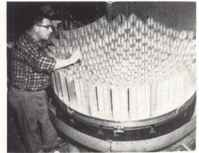
RIBS of egg-crate reflector are epoxy-bonded to each other and base plate—Fig. 3
