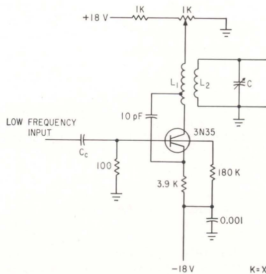
VOLTAGE-controlled oscillator uses a silicon tetrode transistor and operates at a frequency of 100 Mc—Fig. 3
