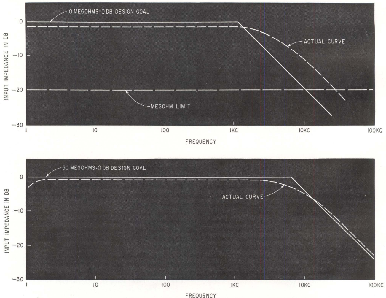
NORMALIZED theoretical and actual input impedances versus frequency for circuit of Fig. 2D (top) and Fig. 2E (bottom)—Fig. 3
