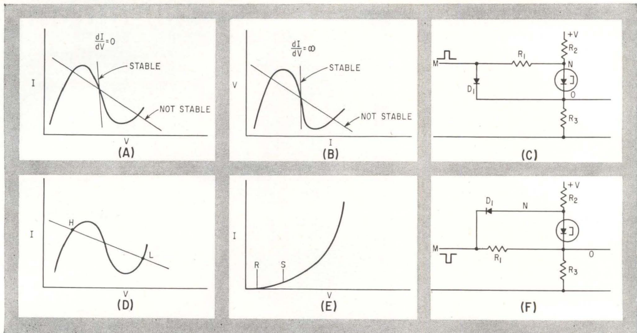
STABLE and unstable load lines (A and B). Positive-pulse-triggered tunnel diode flip-flop (C) with V-I characteristics (D) and diode characteristics (E). Negative-pulse-triggered tunnel diode flip-flop shown at (F)—Fig. 1
