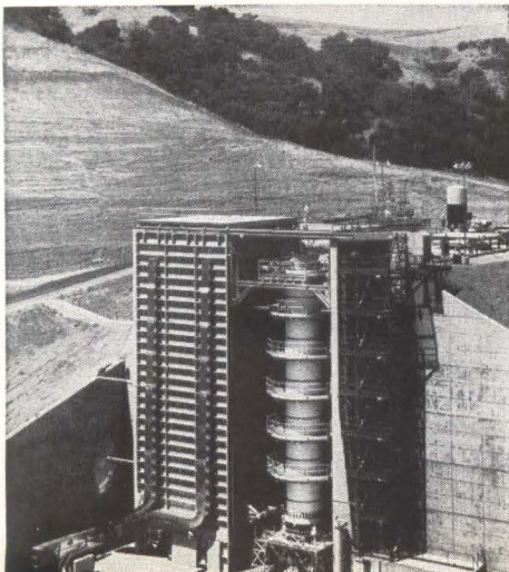
VERTICAL TEST bay—the biggest of its kind in the nation—was used in the static test-firing
