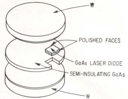
CLOSEUP of the Engeler-Garfinkel junction laser that achieved high power output, (A); and an exploded view, (B)
