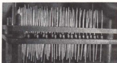
TOP PLATE positioned over the units insures that all leads are perfectly concentric—Fig. 4
