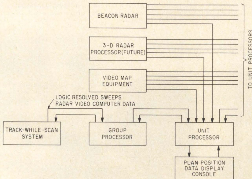
SYSTEM INPUTS are combined in each unit processor. As many additional display consoles as necessary may be added—Fig. 1
