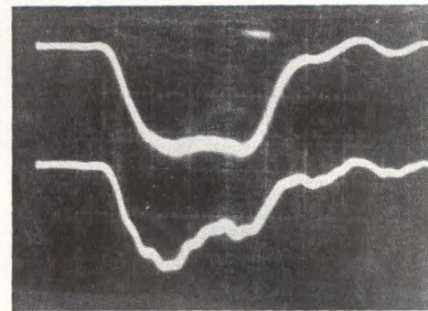
PHOTOMULTIPLIER output, taken through monochromator, shows quenching: upper trace shows current pulse applied to one laser only, lower trace shows quenching effect of second current pulse applied to quenched laser 50 nanosec later—Fig. 2
