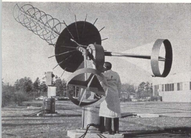
HELICAL ANTENNA is 14 ft long and 27 inches in diameter with a ground plane 72 inches in diameter. It can rotate 720 degrees in azimuth and 180 degrees in elevation
