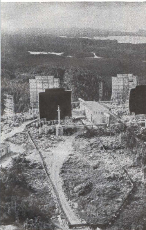
TRUTCH ISLAND relay station. High-gain, 60-ft-square, 70-ton antennas are built to withstand the weight of an inch of ice and 120-mile winds
