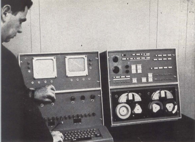
INFORMATION typed on keyboard and displayed on scope is simultaneously stored in central memory. From there it may be transferred to magnetic tape
