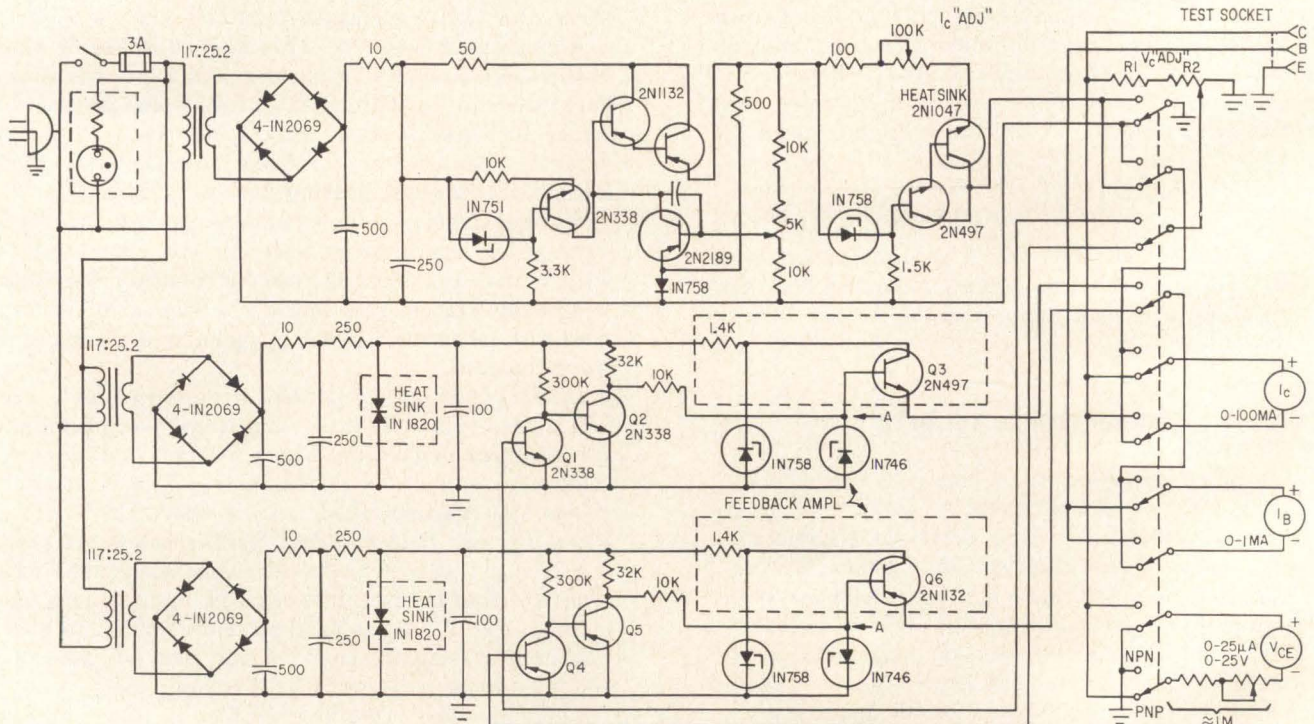
WIDE RANGE, active, common-emitter beta test set uses two feedback amplifiers, measures both npn and pnnp transistors to 1 to 7 percent error—Fig. 4
