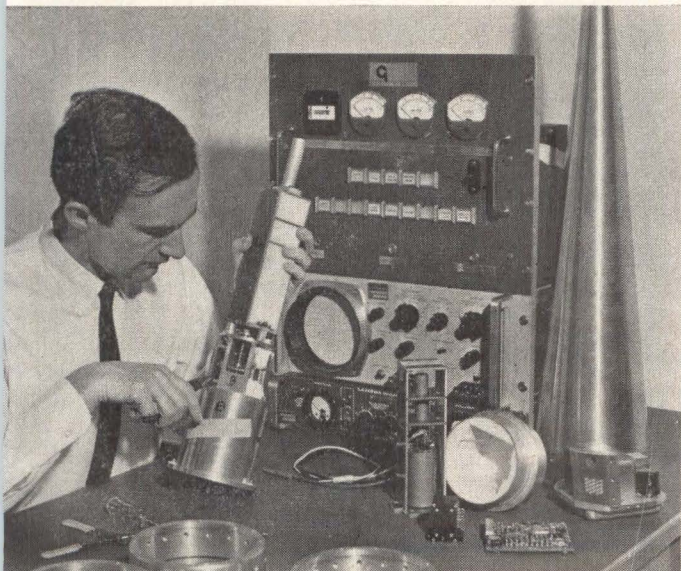
INSTRUMENT PACKAGE for Nike-Apache solar eclipse rocket is adjusted by Leslie G. Smith, project director. Blockhouse control panel is shown in rear
