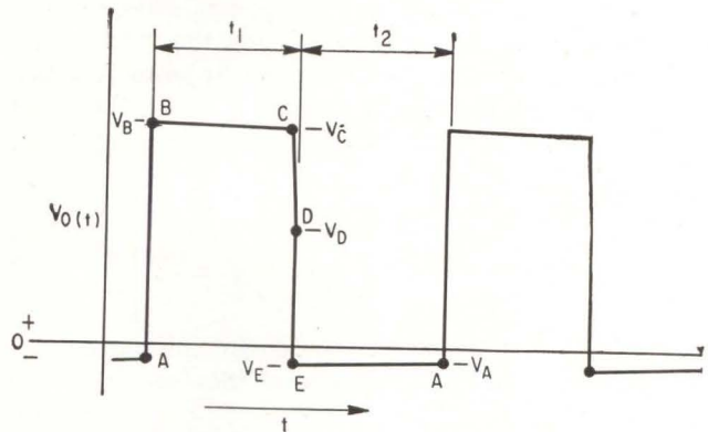
OUTPUT WAVEFORM for astable multivibrator of Fig 1A—Fig. 2
