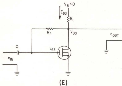
SECTIONAL view of p-MOST (A), suggested symbol and terminal notation (B), drain current vs drain voltage with gate voltage a parameter (C), drain current vs drain voltage with gate tied to drain with gate threshold voltage -8 v (D), automatically biased a-c amplifier stage (E), graphical operating point determination (F)—Fig. 1
