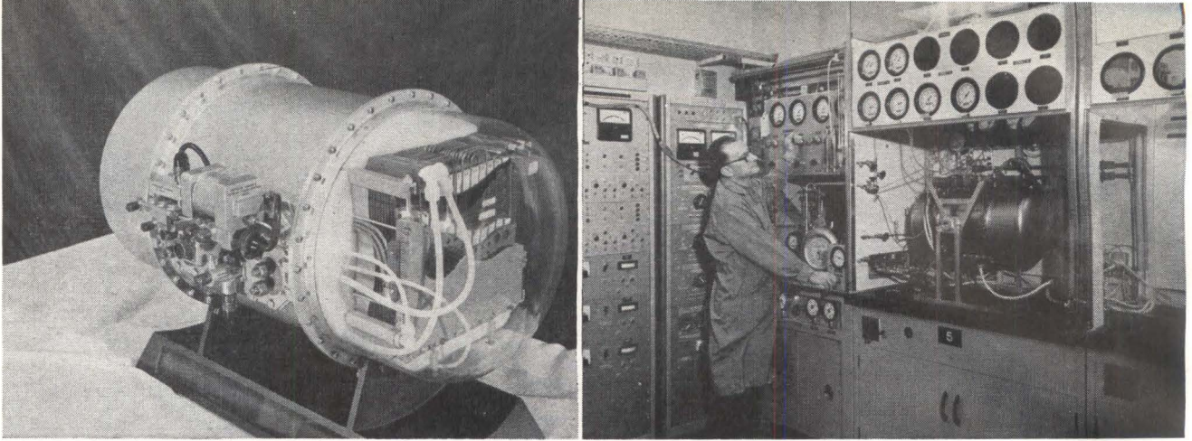
MOCKUP of Gemini fuel cell built by GE (left); fuel cell section on test (right). Load control center behind operator simulates spacecraft load demands—Fig. 2
