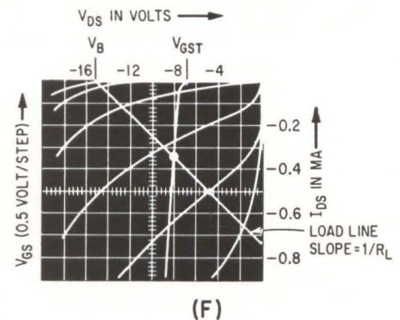
SECTIONAL view of p-MOST (A), suggested symbol and terminal notation (B), drain current vs drain voltage with gate voltage a parameter (C), drain current vs drain voltage with gate tied to drain with gate threshold voltage -8 v (D), automatically biased a-c amplifier stage (E), graphical operating point determination (F)—Fig. 1
