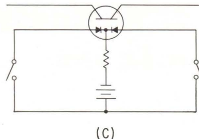
TYPICAL amplifier circuit (A). Load resistance R_L is kept to a minimum to increase operating speed. Applications include simple relay (B) and OR relay (C), Fig. 2
