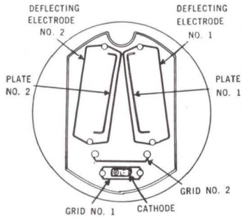
CROSS-SECTIONAL VIEW OF MAIN ELEMENTS OF RCA-7360
