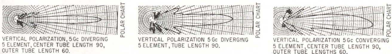
INFLUENCE of element separation and angle \alpha on pattern shape—Fig. 3
