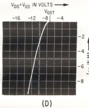
SECTIONAL view of p-MOST (A), suggested symbol and terminal notation (B), drain current vs drain voltage with gate voltage a parameter (C), drain current vs drain voltage with gate tied to drain with gate threshold voltage -8 v (D), automatically biased a-c amplifier stage (E), graphical operating point determination (F)—Fig. 1
