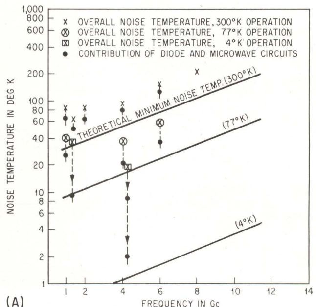
THEORETICAL minimum excess noise temperatures of par-amps at 300, 77 and 4 deg K, and experimental results of seven amplifiers (A). Excess noise from the circulator and following states is shown by dotted lines, excess noise temperature of diode and mount alone, by dots. Cross-section view of traveling-wave light modulators (B) —Fig. 3
