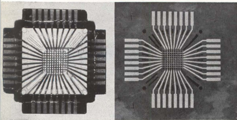
DEVICE with 0.030-inch core diameter prior to deposition of magnetic material (A) and one set of printed wires used in the 0.030-inch form (B)—Fig. 2
