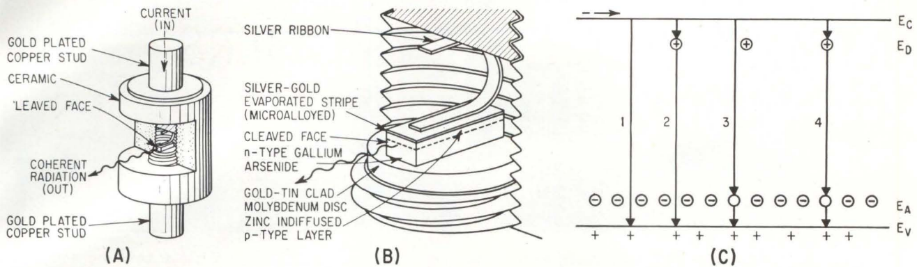
HIGH-PULSE-POWER laser package (A), with window cut in ceramic spacer for the coherent output radiation; diode laser detail (B). Four mechanisms (C) for radioactive transitions: (1) conduction to valence band; (2) donor to valence band; (3) conduction band to acceptor; (4) donor to acceptor—Fig. 1
