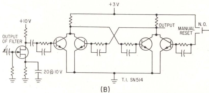
FLIP-FLOP and gate circuit (A) for opening and closing transistor switches; flip-flop (B) changes state when critical frequency is applied to filter—Fig. 4
