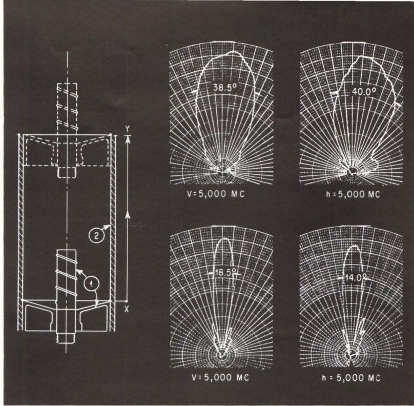
LINEAR radiation patterns for two extreme positions of the helix coupler within the glass-fiber tube—Fig. 2
