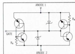
Silicon Bilateral Switch Equivalent Circuit
