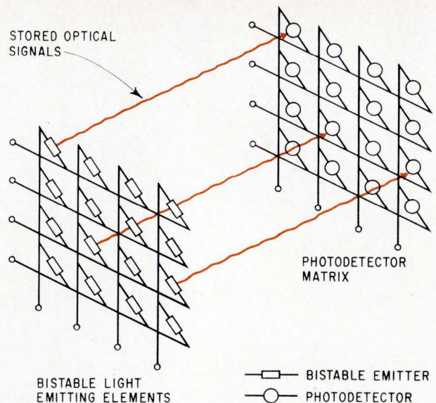
Memory matrix is built with bistable optoelectronic elements. The bistable elements are in matrix at left; the right-hand matrix is an array of detectors that determine the states of the bistable elements on command. Colored lines show light paths from emitter to detector.
