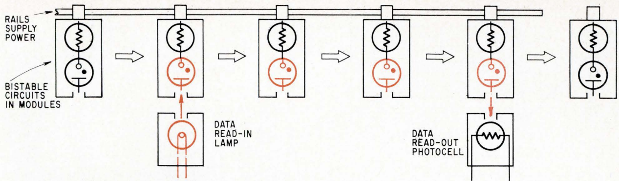
Assembly line uses bistable optoelectronic element. Each module travels along the line with a unit being assembled. Light bulbs beside the line indicate conditions at each assembly station. When a module passes a glowing light bulb, its bistable circuit turns on and its neon bulb glows. Later the module passes a photocell beside the line, which "sees" the glowing neon and produces a signal for the nearest assembly station. Modules are turned off when they run off the end of the rail at the end of the assembly line.
