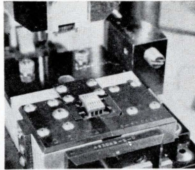
Crimping machine, simultaneously squeezes 14 barrel-shaped contacts around a flatpack's 14 leads. The process takes less time than is required to solder or weld flatpack leads.
