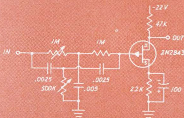
60 CPS Bandstop Amplifier
