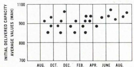
Control chart of test averages of delivered capacity over a year's time. Data represents sample groups taken from a run of 22,000 cells. (Minimum acceptable capacity—800 MAH)
