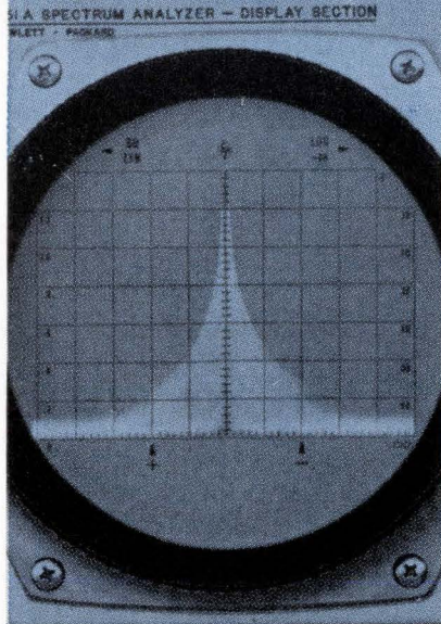
Spectrum signature of L-Band radar (horizontal 3 mc/cm, vertical 10 db/cm); 851B/8551A wide display dynamic range allows viewing of magnetron moding and transients 40-50 db below pulse main lobe.
