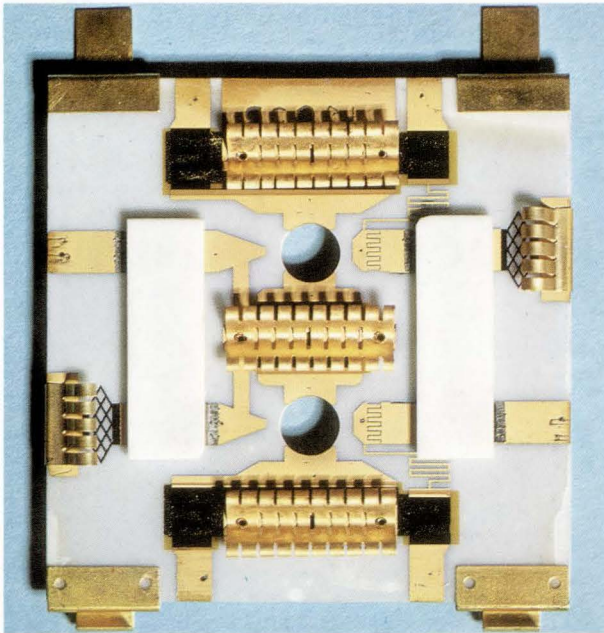
Evolution of Bell Telephone Laboratories' 3.5- to 4.5-Gc amplifier begins (upper right) with a plan ceramic substrate that is built up, step by step, from left to right, with components. The finished IC—except for transistors which are missing in this picture—(above) becomes one of the four IC's that make the completed amplifier (lower right).
