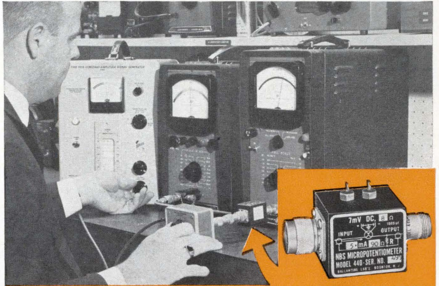
Model 440 Micropotentiometer being used to calibrate voltmeter on right
