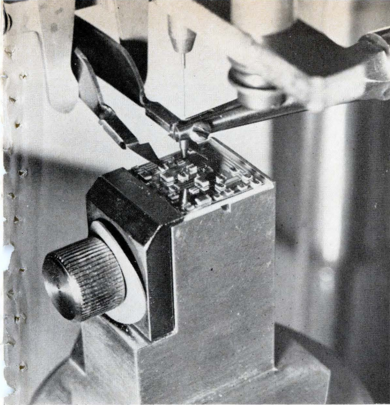
Ultrasonic bonder attaches gold leads to chip mounts and to thin-film conductors on the hybrid-circuit substrate. The close-up photograph at the left shows the bonding tip poised above a transistor mounted on a ceramic channel.
