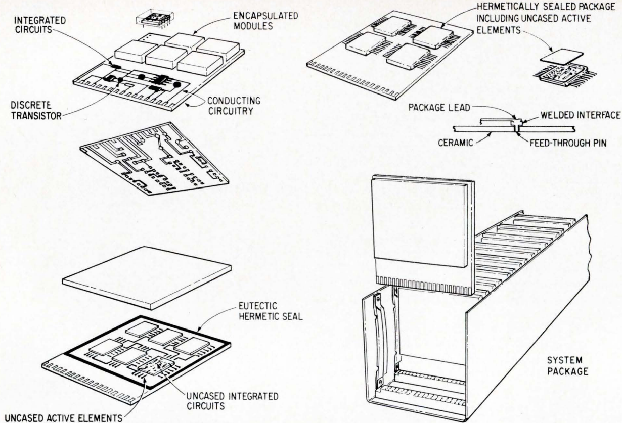
Alternate methods of making hybrid-circuit arrays are to plug sealed packages into a ceramic base (upper left), seal the circuits under one cover (lower left), or weld ribbon leads to feedthrough pins (upper right). The respective power ratings per square inch are 4 watts, 50 watts and 10 watts. Each type can fit into the system package shown.
