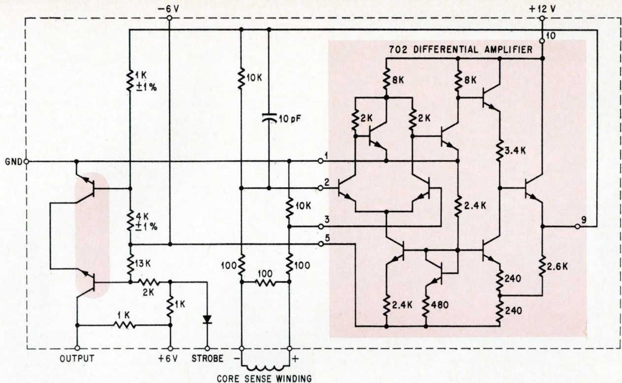
Sense amplifier is built with a monolithic circuit and a transistor, both in flatpacks (colored areas), that are attached to a passive network made by the thick-film process. The hybrid-circuit assembly is shown at the top of page 106.
