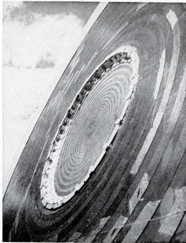
Monopulse feed , consisting of two spiral antenna—one inside the other—operates over a 4-to-1 frequency band with a sharp gain in boresight accuracy. The antenna was developed by Radiation Systems, Inc.
