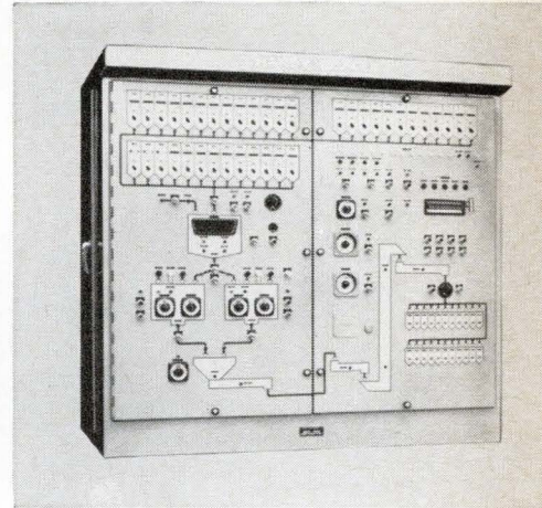
Standard punched cards, read by A-MP Card Reader, operate this batch mixing equipment.
