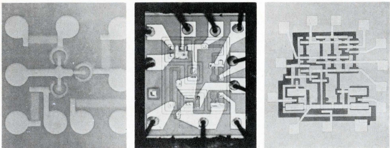
Three forms of monolithic circuits (left to right): a compatible circuit which has four film resistors (the faint bars) atop the silicon crystal in which the active devices are grown; a conventional IC with bipolar transistors and resistors diffused into the silicon; a metal-oxide-semiconductor circuit built primarily of field effect transistors.
