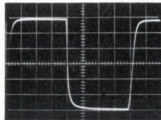
60 cps square wave drive showing maximum efficiency.
