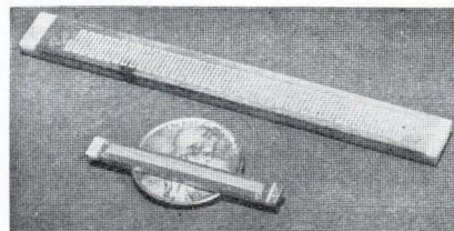
Photoetched slow-wave structures are formed by etching away some of the copper bonded to the beryllia substrate.
