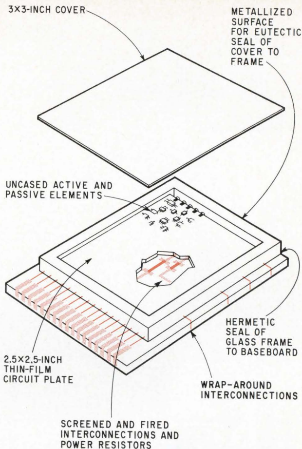
Package planned for large subsystems. Although nine times as large as the inch-square packages already developed, this package can be made the same way. Honeywell hopes to put 60 analog circuits into it.
