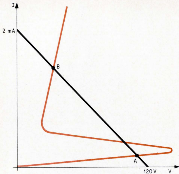
Characteristic curve and load line for a bistable optoelectronic memory element containing a photocell and neon, as shown on page 85. The straight line joins the points of zero current and zero voltage, and intersects the curve at its stable points.
