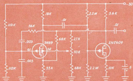
Wien Bridge Oscillator
