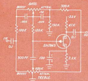
Hi-Fi Tone Control
