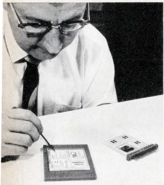
Modular hybrid-circuit array is built by sealing four ceramic frames to a ceramic base, putting thin-film circuits into the frames and then sealing the frames with ceramic covers. A base-frame assembly and an almost-completed array are seen in the photo. The circuits are interconnected with conductors (color, in drawing) that are screen-printed on the base along with power resistors and package leads.
