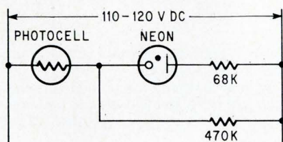
Assembly line uses bistable optoelectronic element. Each module travels along the line with a unit being assembled. Light bulbs beside the line indicate conditions at each assembly station. When a module passes a glowing light bulb, its bistable circuit turns on and its neon bulb glows. Later the module passes a photocell beside the line, which "sees" the glowing neon and produces a signal for the nearest assembly station. Modules are turned off when they run off the end of the rail at the end of the assembly line.
