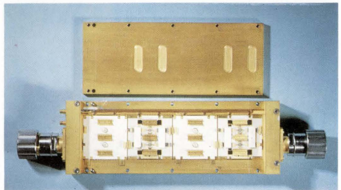
Evolution of Bell Telephone Laboratories' 3.5- to 4.5-Gc amplifier begins (upper right) with a plan ceramic substrate that is built up, step by step, from left to right, with components. The finished IC—except for transistors which are missing in this picture—(above) becomes one of the four IC's that make the completed amplifier (lower right).
