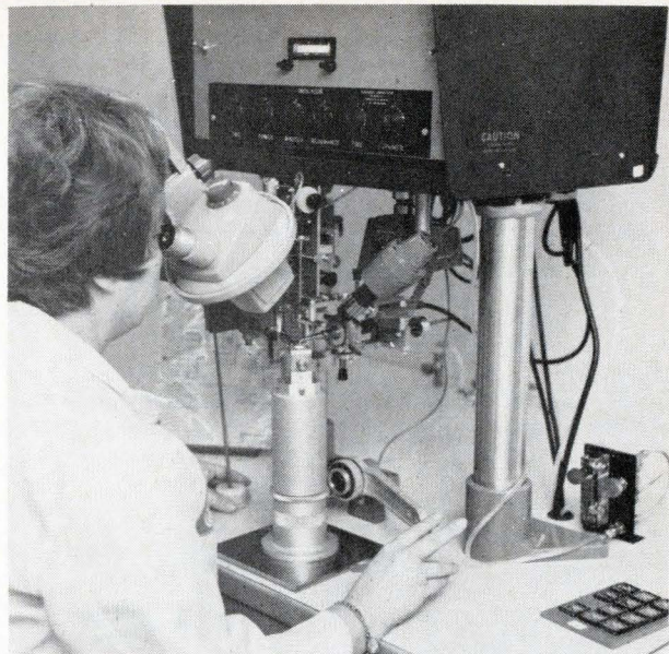
Ultrasonic bonder attaches gold leads to chip mounts and to thin-film conductors on the hybrid-circuit substrate. The close-up photograph at the left shows the bonding tip poised above a transistor mounted on a ceramic channel.
