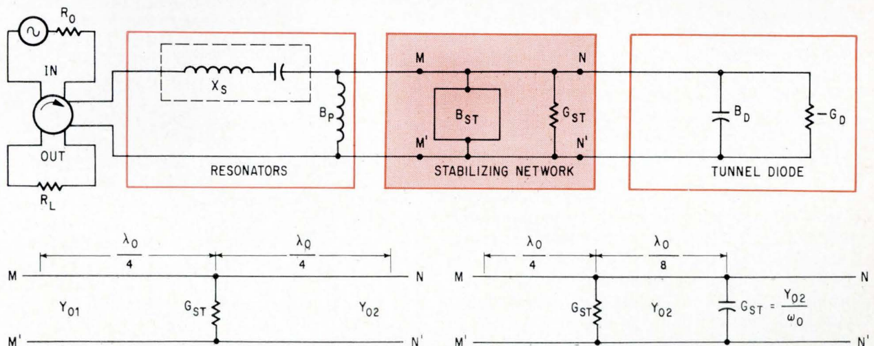
To prevent oscillations outside the circulator passband, the tunnel diode circuit includes a stabilizing network, consisting of B_{ST} and G_{ST} . Typical stabilizing circuits shown below are the shunt, left, and the capacity-loaded types.
