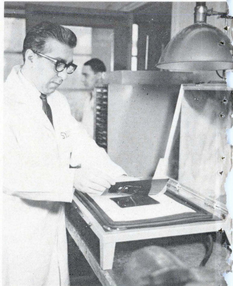
Reduced size negative is used to expose a light-sensitive coating on the copper clad dielectric. After spraying with a suitable etch, only sections of copper corresponding to the center conductor configuration will remain.
