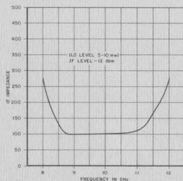
Fig. 3. Typical impedance levels measured at IF ports.
