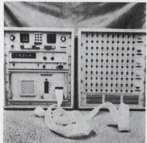
Static strain data acquisition system 910 features a random access keyboard for manual channel selection. It scans at a rate of 5 per second and handles 50 to 1,000 channels in 10 channel increments. Input to the system is by shielded cable to either barrier terminal strips or MS type 5-pin connectors. Electronics Ltd., P.O. Box 1972, Cedar Rapids, Iowa 52406. [428]
