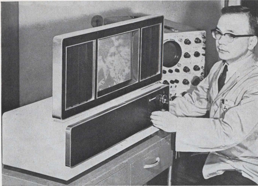
Tuning in. Still under development, the flat screen has a 13-in. diagonal. The receiver is being adjusted by Masami Yoshiyama, the author and head of the project. Though resolution is below par for close viewing, the tv picture at left, made from a live telecast, is comparable to those of some low-cost video tape recorders.
