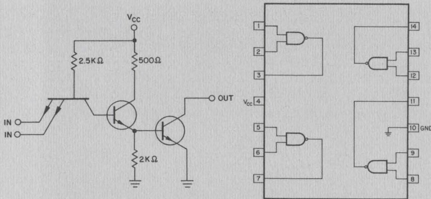
Fig. 1. Circuit and logic diagrams of SG-350 line/lamp driver.
