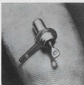
Gas-filled metal diodes serve as protective devices against transients or other sharp spikes, such as those which can puncture MOS FET's. Inherent firing voltage is 80 to 89 v. Leakage resistance is greater than 3.5 \times 10^{14} ohms. Repeatability of firing voltage is approximately \pm 5\% and self capacitance 1.1 pf at 100 khz. Victoreen Instrument, 10101 Woodland Ave., Cleveland. [438]
