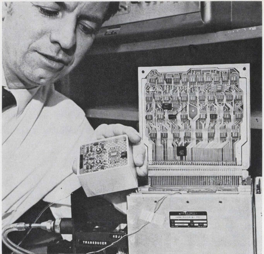
Key element. At the heart of the Honeywell air data system is a pressure sensor that converts data into formats acceptable to a digital computer.
