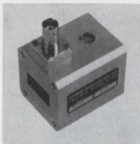
Impatt-diode oscillator X935 is for mechanically-tunable service in the 8.2 to 12.4 Ghz band. Power output is 100 mw c-w into termination with vswr less than 1.3:1. The unit has a single power supply requirement of 75 v at 50 ma. Size is 1.63 x 1.63 x 2 in. block with BNC bias receptacle. Price is $395. Somerset Radiation Laboratory Inc., 2060 N. 14th St., Arlington, Va. [402]
