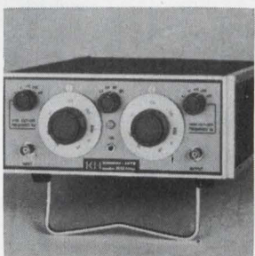
Solid state variable filter model 3550 is tunable over the range of 2 hz to 200 khz and provides low-pass, high-pass, band-pass, and band-reject operation. Mode of operation is easily selected by a front panel switch. An input FET amplifier provides high input impedance and zero db insertion loss. Price is $525. Krohn-Hite Corp., 580 Massachusetts Ave., Cambridge, Mass. [386]
