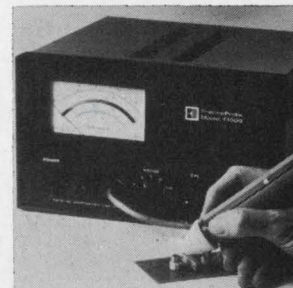
Infrared thermometer called ThermoProbe T-1000 can spot check, monitor, and record temperature of circuit board components without contact. It measures temperature in 4 switch-selectable ranges from 20^\circ to 500^\circ\text{C} , with emissivity compensation from 0.2 to 1 on all ranges to provide accurate readings of a variety of surfaces. Raytek Inc., 1277 Terra Bella Ave., Mtn. View, Calif. [368]
