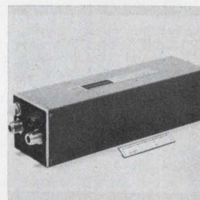
Permanent-magnet-focused, traveling-wave amplifiers offer 100 mw power output in S band (WJ-477), C band (WJ-476) and X band (WJ-472). The single-reversal units also have in common 13 db maximum noise figure and 30 db minimum small signal gain. Packaging is 3 x 3 x 10.5 in. and weight is 6.5 lbs. Watkins-Johnson Co., 5333 Hillview Ave., Palo Alto, Calif. [408]
