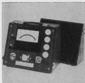
Laboratory standard r-f peak wattmeter 4345 is for pulsed transmission systems. It samples forward or reflected power in an accurately machined 50-ohm reference line section. Full scale power is selected in five values from 250 w to 5 kw. Frequency range is 950-1,300 Mhz. Insertion vswr with connectors is less than 1.08. Bird Electronic Corp., Aurora Rd., Cleveland. [361]
