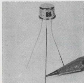
Triple-diffused silicon power transistors series SDT4921-SDT4925 are 300-v, 5-amp devices in TO-5 cases. They feature ultrasonically bonded leads and gold silicon eutectic die mounting. Beta at a collector current of 1 amp is a minimum of 20 and a maximum of 60. Collector to emitter voltage is less than 0.5 v. Solitron Devices Inc., 1177 Blue Heron Blvd., Riviera Beach, Fla. [440]
