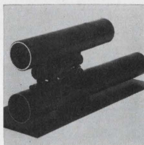
Diode laser transceiver TR-1 consists of a diode laser array, laser modulator, transmitting optics to yield a 12 milliradian beam divergence; the receiver contains collecting optics, a narrow-passband filter, aperture stop to determine acceptance angle, photo diode and power supply as well as pre-amplifier. Seed Electronics Corp., 9 Cypress Dr., Burlington, Mass. [383]
