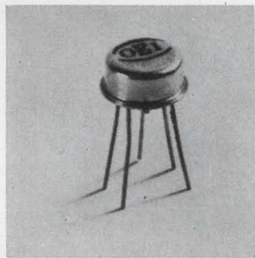
Monolithic timing circuit model 7100 is for any type of timing application, from monostable delay circuits to turn-on delays. Features include: 10 \mu sec to 1 hour time delays; only 1 to 2 external components required for the majority of applications; and output compatible with 10 volt analog, MOS, RTL, DTL and TTL forms of logic. Optical Electronics Inc., Box 11140, Tucson. [441]
