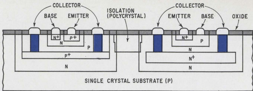
PNP TRANSISTOR
