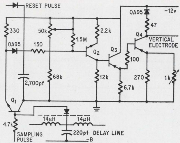
Brightness circuit. Acting as a variable resistor, the input transistor accepts a signal proportional to the delay line voltage when a negative sampling pulse is present.
