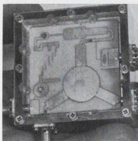
S-band parametric amplifier is built in hybrid microwave IC format on a single substrate. Principal components are a ferrite junction circulator, input matching networks, a high cutoff frequency varactor diode, pump and idle frequency filtering and an avalanche diode oscillator pump source. Range is 2.2-2.3 Ghz. American Electronic Laboratories Inc., Colmar, Pa. [406]
