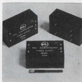
Power supply model PD-15 is a \pm 15 v unit designed for operational amplifiers and IC's. It is an isolated supply and operates from 28 \pm 4 v d-c source. Line regulation for a \pm 4 v change is better than \pm 0.5\% . Output ripple is less than 0.3% and the unit will operate from -20^\circ to +71^\circ C (case temperature) without derating. Mil Associates, Dracut Road, Hudson, N. H. 03051. [388]
