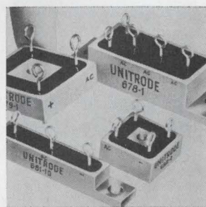
High-current, controlled-avalanche rectifier assemblies in the Magnum series have a piv range of 100 to 600 v. They include 25 amp single and three-phase bridges, 10 amp single-phase bridges, and 15 amp doublers and center-tap rectifiers. Units have prices varying from $3.43 to $12.60 in lots of 100. Unitrode Corp., 580 Pleasant St., Watertown, Mass. [439]
