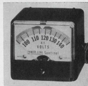
Power line sentinel voltmeter model 658-R offers an expanded scale meter movement reading 100/140 v, jeweled bearing moving coil D'Arsonval type with full wave bridge rectifier having wide operating frequency range. Accuracy from 110/125 v is \pm 2\% , below 110 and above 120 a-c volts, \pm 3\% accuracy. Hoyt Electrical Instrument Works Inc., Cambridge, Mass. [364]
