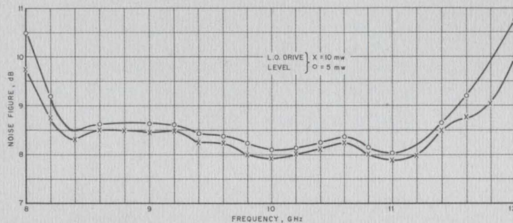
Fig. 1. Typical noise figure plot of X-band mixer over frequency range.
