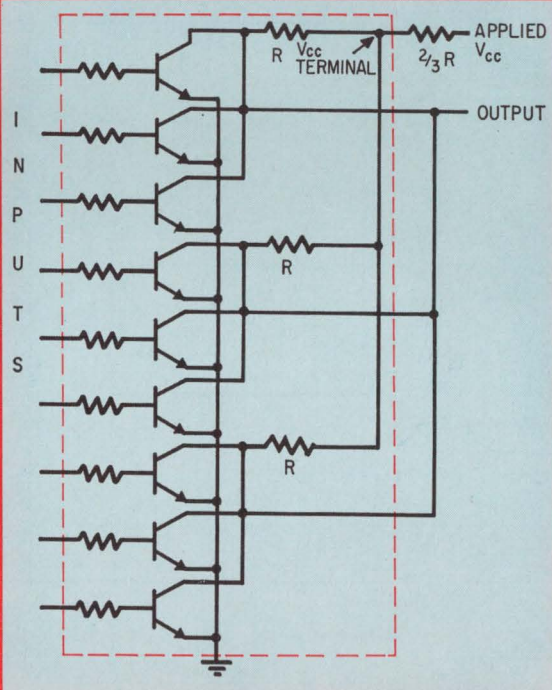
Packed. A new V_{cc} applied through an external resistor allows the collectors in a multiple-gate IC to be tied together.
