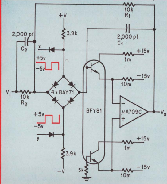
Better tracking. The dual transistor reduces the feedback capacitor's discharge current and, therefore, reduces the hold error.
