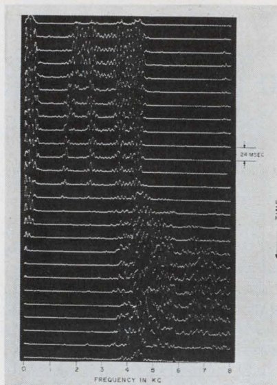
Voiceprint. Spectra of the spoken word "is", sampled every 24 msec. These are examples of input to the MCU-6.
