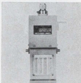
Three-stage Satcom receiver filter model 40C146000 operates over a frequency range of 7.25 to 7.75 Ghz with an insertion loss of 0.60 db at center frequency. It features a minimum instantaneous 0.7 db bandwidth of 50 Mhz over its tuning range, insertion loss of 0.60 db at center frequency. Frequency Engineering Laboratories, P.O. Box 527, Farmingdale, N. J. 07727. [407]
