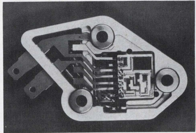
IC regulator. Using thick-film circuit on ceramic substrate, this voltage regulator produced by Motorola for Ford is typical of the units now replacing conventional relay-operated designs.
