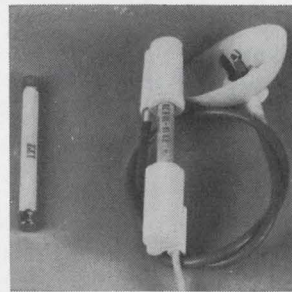
Selenium high-voltage rectifier TV18-TOK70 for black-and-white tv application features high life expectancy. The 24 kv piv rectifier has the length of a comparable h-v tube rectifier, 2 \frac{3}{4} in. The baseplate material has a thickness of approximately 0.003 in. compared with 0.012 in. of standard material used until now. ITT Semiconductors, 6416 W. Belmont Ave., Chicago 60634. [443]
