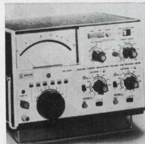
Model PM6509 meter performs leakage current, breakdown voltage and resistance measurement in pico and nanoamp regions without auxiliary equipment. Current measurements down to 3 pa, breakdown voltage up to 1,000 v and resistance measurements up to 100 teraohms are accurately performed. Price is $1,100. Philips Electronic Instruments, Mount Vernon, N. Y. [366]
