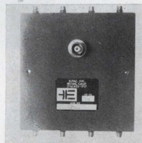
Stripline microwave power divider works in a frequency range from 8 to 12 Ghz. It accepts up to 50 w c-w input and provides 8 outputs mutually isolated by at least 10 db. Output signal phase is identical within \pm 10^\circ at all output ports. Insertion loss is 9.5 db \pm 1 db to any output port. Input vswr is 1.5:1 max. Elpac Inc., 18651 Von Karman Ave., Irvine, Calif. [404]
