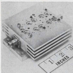
Solid state, high power r-f amplifier provides 100 w peak pulse power or 75 w c-w in the frequency range from 200 to 500 Mhz. A variety of models is available to provide gain values from 4 to 30 db. Power requirement is +28 v d-c, and input vswr is 2:1 maximum. Size of the 8 db model is 3.5 x 3.75 x 1.5 in. Acrodyne Industries Inc., 666 Davisville Road, Willow Grove, Pa. [401]
