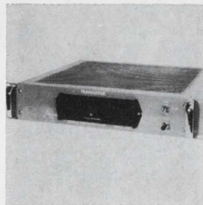
Digital data translator accepts up to 20 bits, in any weighted code, for translation of purely numerical data into 8 significant decimal figures of preselected scale factors and units. Complete translation of a 20-bit input takes 1.5 msec max., permitting 500 translations/sec to be made. Price $4,300. Adtrol Electronics Inc., 116 N. 7th St., Philadelphia 19106. [422]
