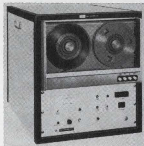
Data acquisition system model 710 can multiplex and digitize 64 channels of low-level analog data onto magnetic tape. It contains a 16-channel FET multiplexer which is expandable to 64 channels with a switching speed of 1 \mu sec/channel. Accuracy of the integrating digitizer is 0.015% of full scale at 15 msec/conversion. IRA Systems Inc., 332 2nd Ave., Waltham, Mass. [423]
