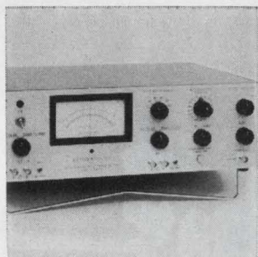
Audio-video phase measurements with an active RC filter for increased response time are provided in the model 351 differential phase meter. The balanced or unbalanced inputs permit phase measurements on transmission lines, lattice filters, etc. without additional circuitry. Input sensitivity is 1 mv per channel. Wiltron Co., 930 East Meadow Drive, Palo Alto, Calif. [362]
