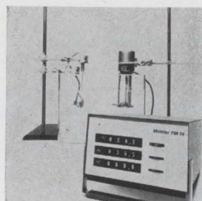
Direct-reading digital thermometer TM16 measures temperatures in the -20^\circ to +300^\circ\text{C} range with 0.05°C reproducibility and digital indication in 0.1°C increments. The temperature of liquids, vapors, and semi-solids such as greases and pastes can all be measured or controlled with the TM16. Price is $895. Mettler Instrument Corp., Nassau St., Princeton, N.J. 08540 [366]
