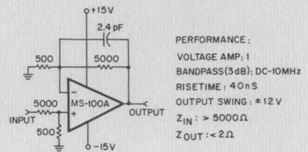
Fig. 3. MS-100A in the non-inverting configuration.
