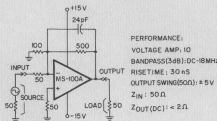
Fig. 2. The MS-100A as a video power amplifier.
