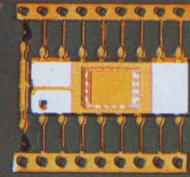
AlSiPak ® No. SZ-80108-AC 16 lead package with device area .170 x .220
