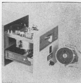
Magnetic tape system CONCEPT is a modular automatic system for electronic data processing peripherals. It employs a self-threading enclosed reel of 1/4-in. tape called the Neopaq. When inserted and locked in place, the tape is in direct contact with the central capstan, the only driven member in the system. Newell Industries Inc., 795 Kifer Rd., Sunnyvale, Calif. 94086 [387]
