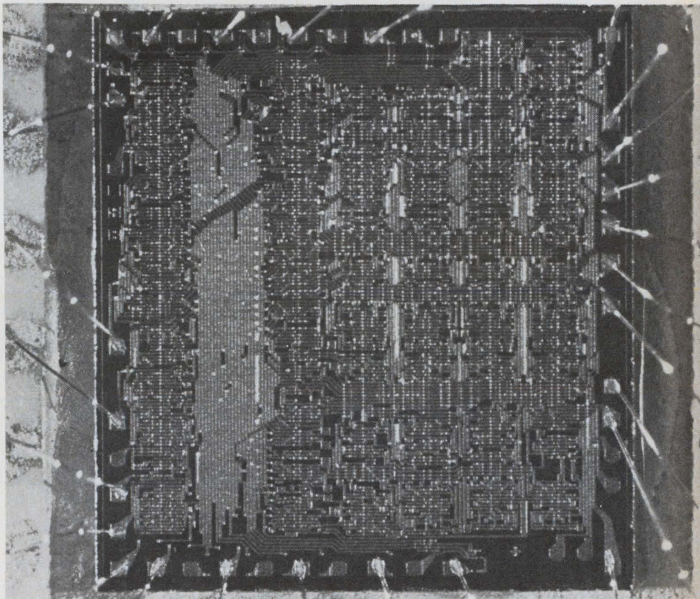
Massive potential. Low-power C/MOS allowed RCA to put 750 devices on 145-mil/155-mil parallel processor built for NASA's Goddard Space Flight Center.
