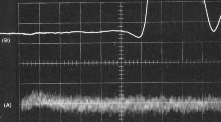
(A) Noisy signal to Boxcar Integrator. (B) Recovered second harmonic signal at output of Boxcar Integrator.
