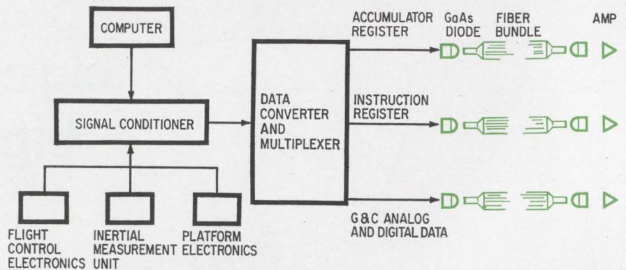
Linking the lines. Autonetics has used 70-foot-long fiber-optic bundles to move data in this guidance and control system in a high-energy electromagnetic pulse environment.
