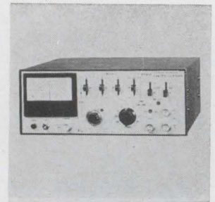
Phase sensitive detector model 822 has a frequency response of 1hz to 1 Mhz. Range is 100 \mu\text{V} resolution to 1 v full scale referred to input. It recovers signals 70 db below noise. Output stability is better than 0.005% of full output /°C. Time constant is 1 msec to 10 sec. Price is $770. Keithley Instruments Inc., 28775 Aurora Rd., Cleveland, Ohio 44139 [364]
