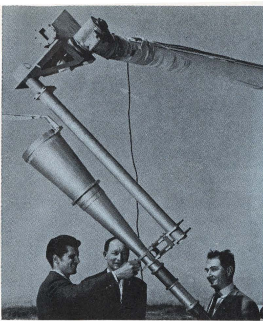
Horning in. These conical antennas will transmit downlink signals from Intelsat 4 to stations on earth. The satellite simultaneously will carry 6,000 telephone channels and 12 color tv programs.
