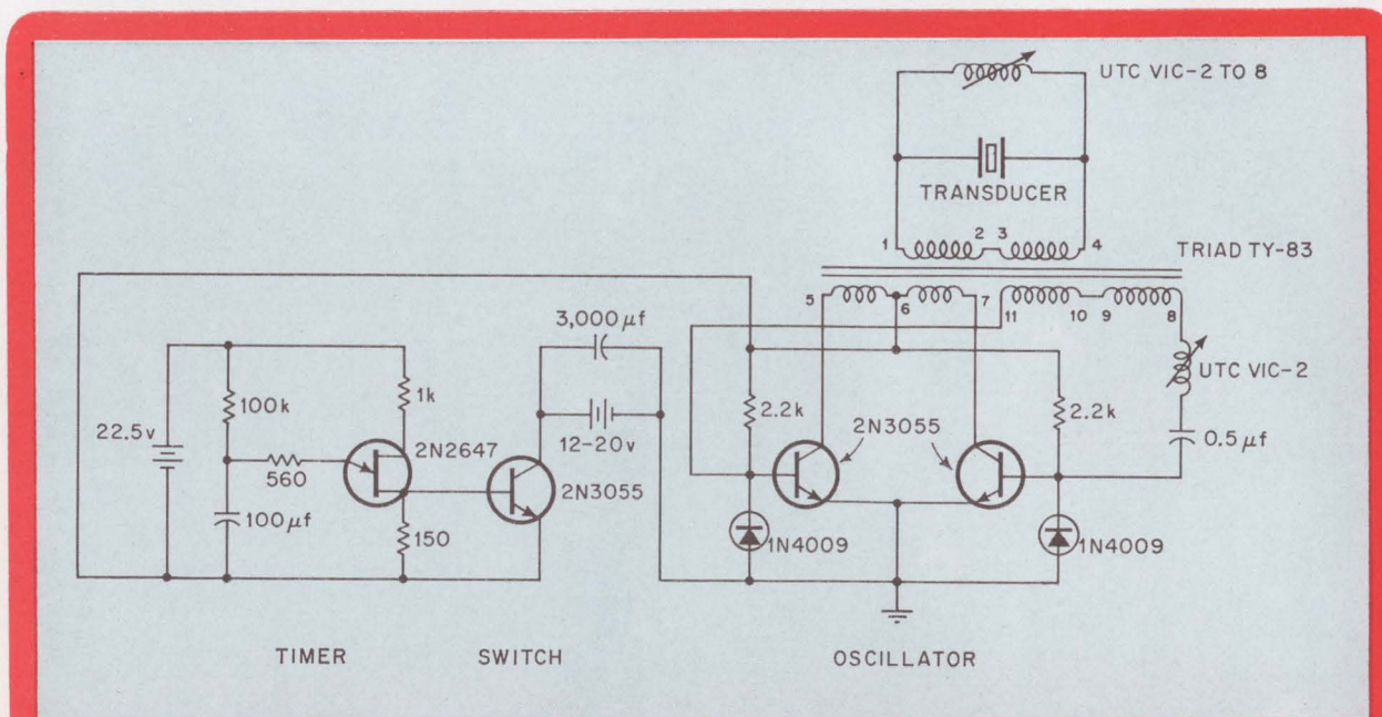
Making waves. The oceanographic pinger generates sounds underwater at a particular frequency. Pulses from the oscillator are stepped up in voltage to drive the transducer. Sound waves generated by the transducer have a frequency which can be adjusted by varying the inductors.
