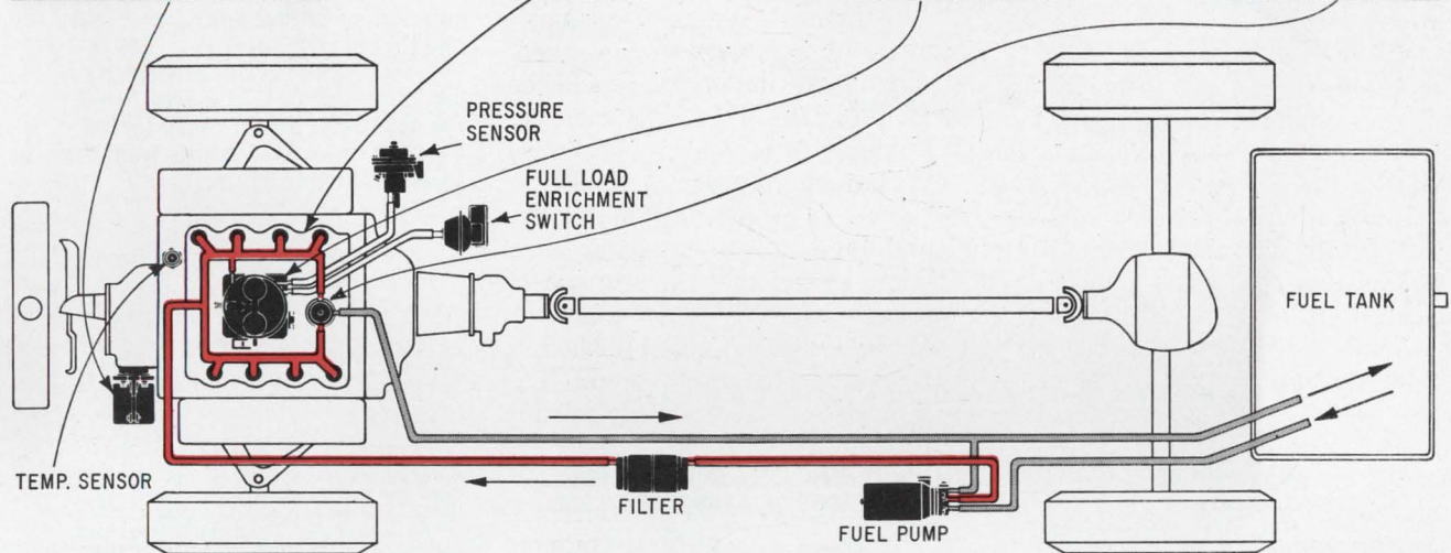
Gassed. Faced with ever-tightening antipollution laws, Detroit's automakers are warming to the virtues of electronic fuel injection. Pictured above is Bendix system now expected to ride on 1971 model cars as an option.
