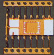
AlSiPak ® No. SZ-80107-AB 14 lead package with device area .170 x .200
