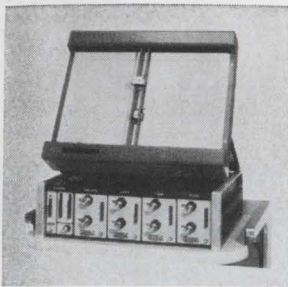
X-Y recorder called Plotamatic 901-2P is a high-speed unit. It features all plug-in electronics, a digital time base with 1% accuracy and sweep speeds from 0.2 sec/in. to 1,000 sec/in. Sensitivity down to 40 \mu\text{V}/\text{in.} , d-c common mode rejection in excess of 150 db, and automatic line coding are offered. Bolt Beranek and Newman Inc., McGaw Ave., Santa Ana, Calif. [361]
