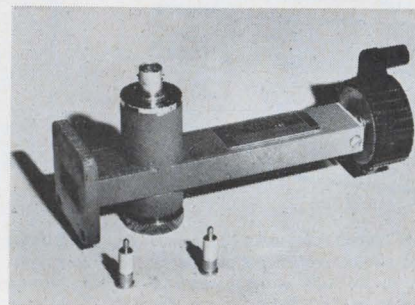
For experiments. Impatts are in front of detector mount.
