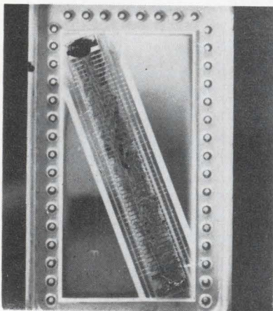
Tight fit. Fabricated in the lab, this new 50-tap filter makes a package of only 1¾ x 1⅛ inches.
