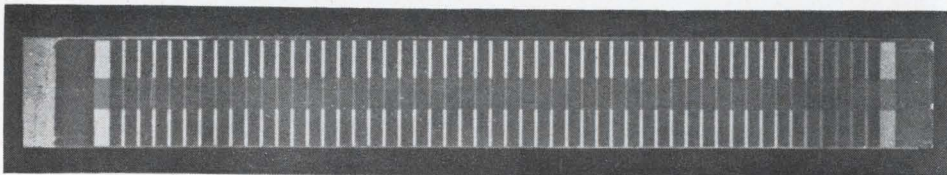
Long codes. These laboratory-fabricated matched filters can handle the complex codes of today's radar. Top, an 11-tap line designed for a 150-Mhz carrier with a bit rate of 1 Mhz. Bottom, the largest capacity to date, a 50-tap, 120-Mhz filter with a 5-Mhz bit rate.
