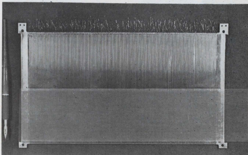
Beribboned. Plated wires laminated in plastic run across five-turn word lines. When several planes are clamped together, ribbon is held rigidly between planes, keeping magnetostrictive effects low. Loops of ribbon linking different planes serve as simple interconnection wires.
