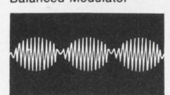
Balanced Modulator
