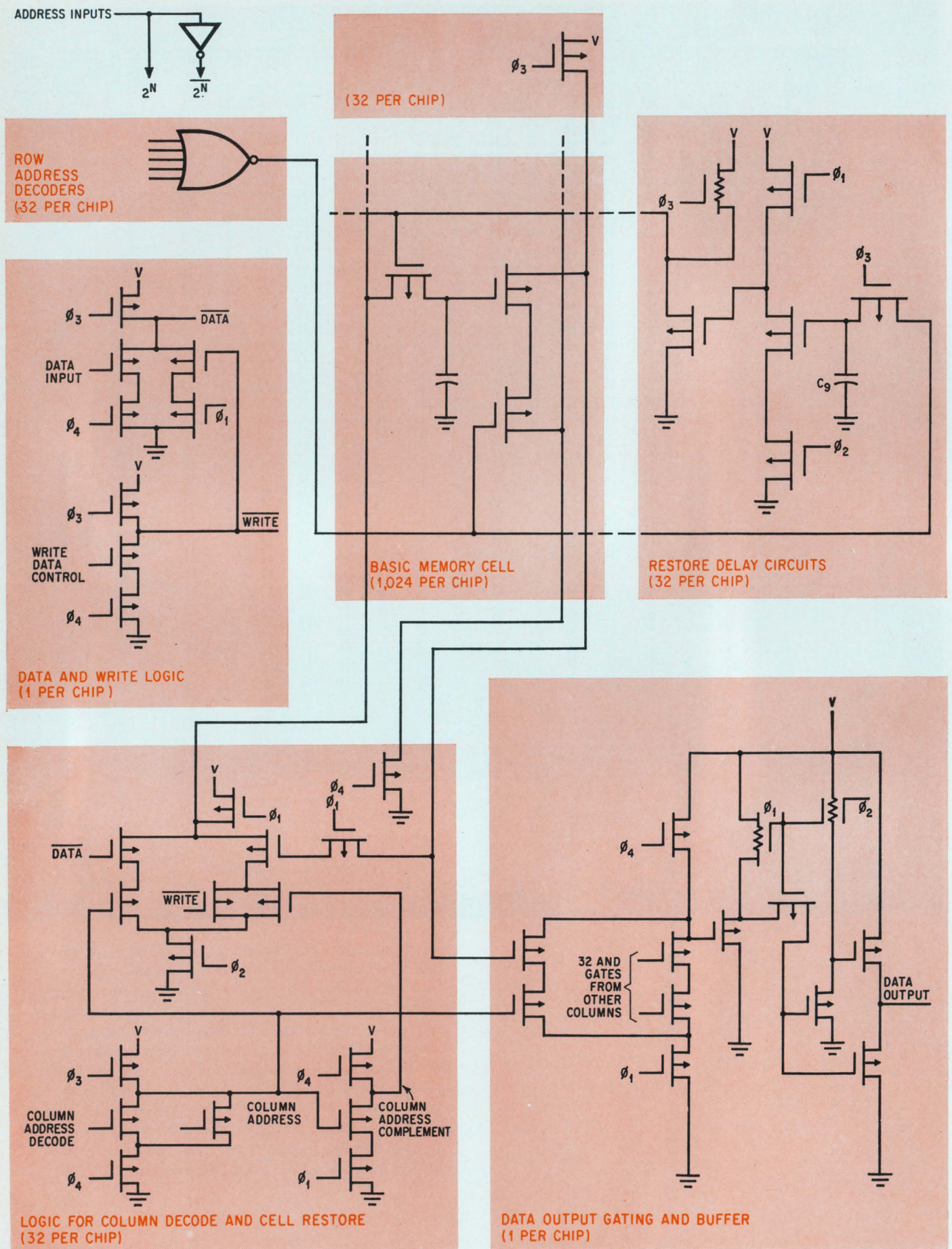
One-chip design. The memory contains all of the circuits required for a 32-row by 32-column random-access memory on a single silicon chip—including one write data input logic stage, one output buffer, and 64 row- and column-selection gates.
