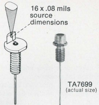
Single laser diode assembly
