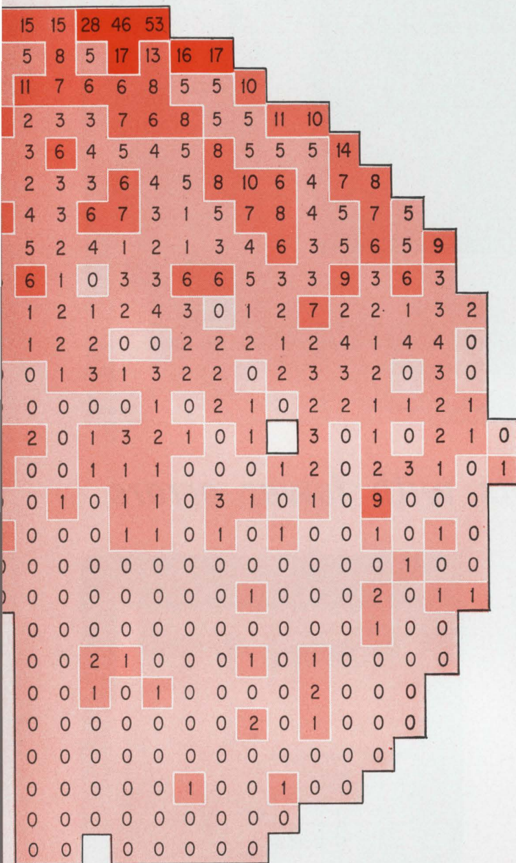
Top to bottom. Distribution of defects on a half-wafer after a single critical process operation shows a gradient from top to bottom. The gradient varies in magnitude and orientation with the operation, so it's difficult to decide on an overall defect distribution. Numbers indicate defects in the area that a single IC will occupy. The empty space near the center is occupied by a test pattern.
