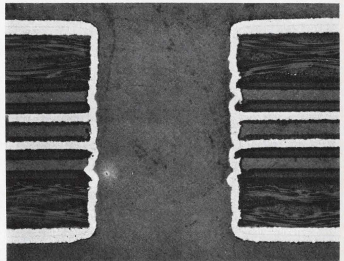
Smooth or smear. Plated-hole wall (top) through six copper-clad circuit layers and 10 epoxy-glass adhesive layers, is fairly smooth because adhesive doesn't extrude during drilling. But smear occurs (below) in sandwich consisting of one polyimide circuit layer between two epoxy-glass layers. Hole diameter is 0.028 inch. White surfaces in cross section are clad or electrodeposited copper.
