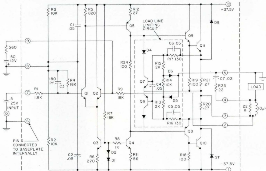
SCHEMATIC OF TA7625A HYBRID POWER MODULE.
