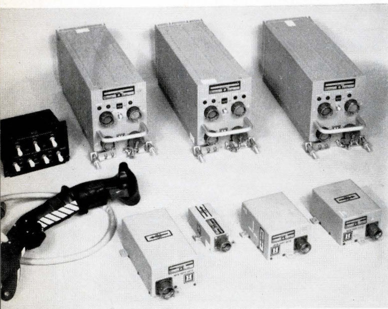
5. Sized up. Components of the control and stability augmentation system made by Honeywell for Grumman Aerospace Corporation's F-14A—the Navy's new air-superiority fighter. Similar components could be used in FBW designs.
