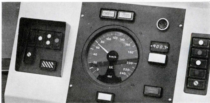
Prototype. Light-emitting diodes form rays, showing maximum permissible speed, around dial and form number display, showing distance to next speed change.
