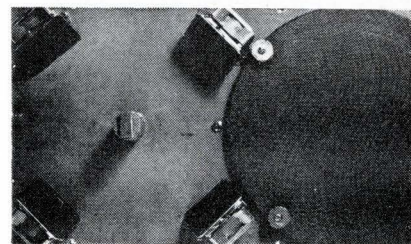
Top view. Mid-range speaker points up and four tweeters aim at central post.
