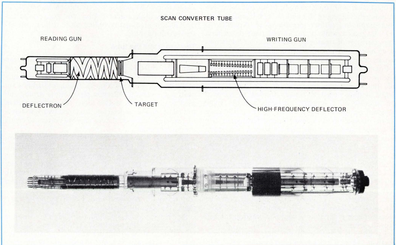
1. Double header. New scan-converter tube is double-ended in design. Target in center is an array of silicon diodes measuring \frac{3}{8} by \frac{1}{2} in. Note deflectron-type deflection system on read gun (left) and delay-line construction on extremely fast write gun (right).
