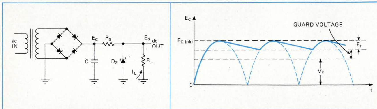
2. Precaution. Guard voltage of shunt-regulated supply prevents ripple voltage from dropping capacitor voltage below output voltage.
