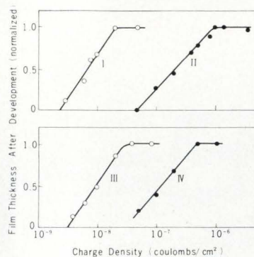
Exposure characteristics of epoxidized polymers and their starting polymers: I, epoxidized polybutadiene; II, polybutadiene; III, epoxidized polyisoprene; IV, polyisoprene.
