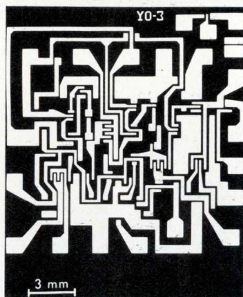
Chromium Mask for IC which is made with an electron-beam drafting machine, utilizing Hitachi's epoxide-containing polymers.
