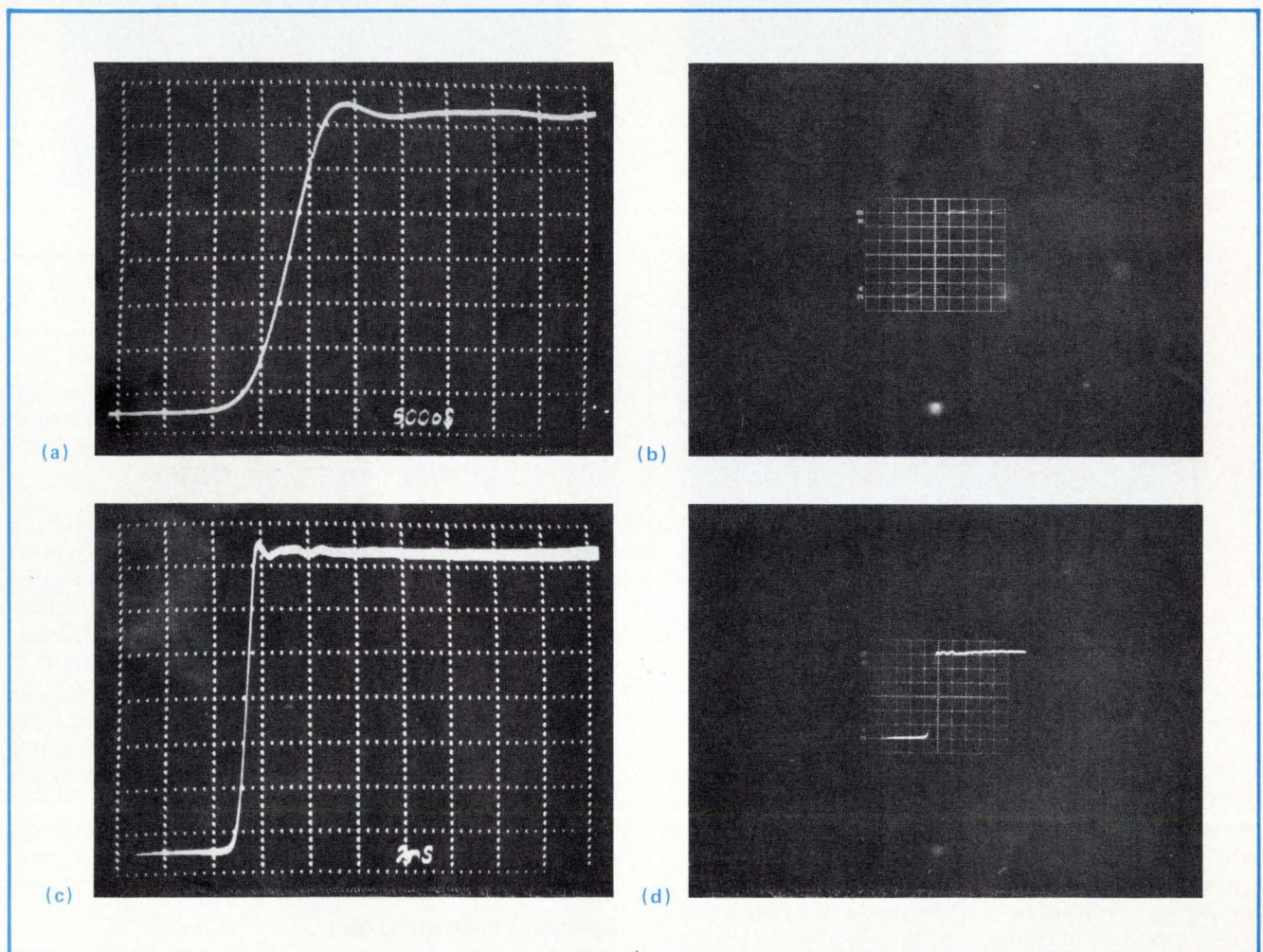
3. Big and fast. Large photos at left, (a) and (c), are taken from a 20-by-25-cm TV monitor displaying data captured by the scan-converter tube. Upper photo (a) has a horizontal calibration factor of 500 ps/div; lower photo (c) is 2 ns/div. The corresponding oscilloscope photos at the right were taken from the screen of a Tektronix 7904 with ASA 10,000 film. A reduced scan was used to increase brightness.
