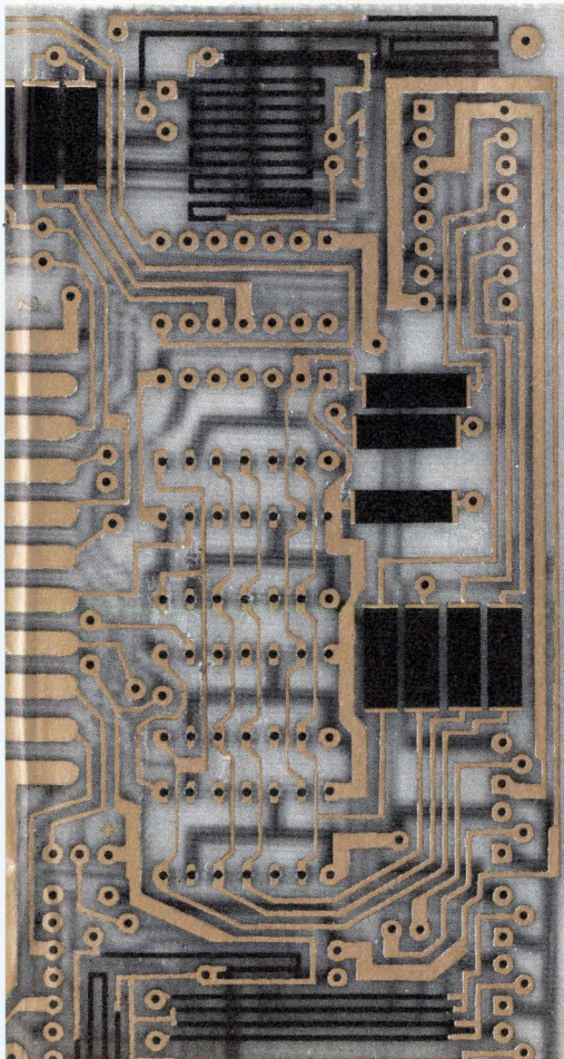
Multilayer printed circuit boards
