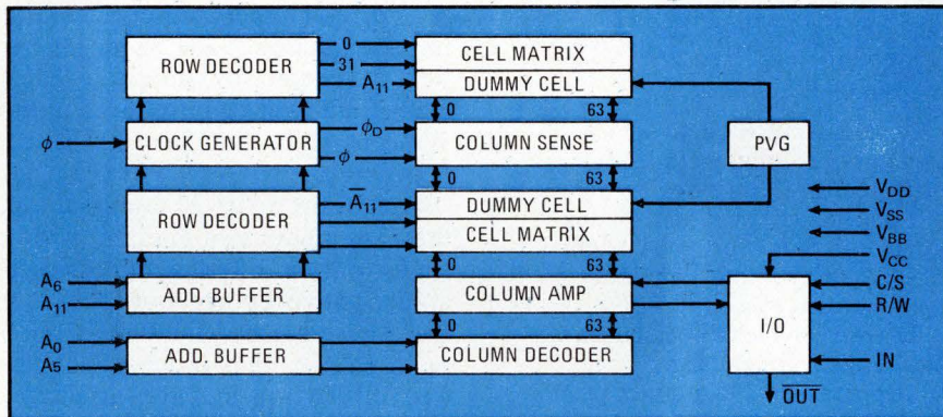
Memory component. Internally, the 4,096-bit random-access memory is a simple structure, organized in 64 columns by 64 rows, with columns and rows selected through a decoder.
