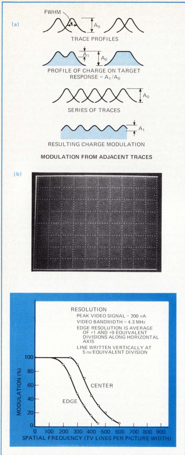
5. Resolution. Gaussian distribution of electron-beam intensity ultimately limits resolution. As beams get closer together, their profiles overlap and the modulation in the charge pattern is decreased. If they intersect at the full width at half maximum (FWHM) points, the modulation is completely lost (a). Resolution of 150 line pairs written at a speed of 200 divisions per microsecond demonstrates tube's performance (b). Resolution is better at the center than at the edges, having a value of approximately 400 TV lines per picture width at the center, and 300 lines per picture width near the edges (c).
