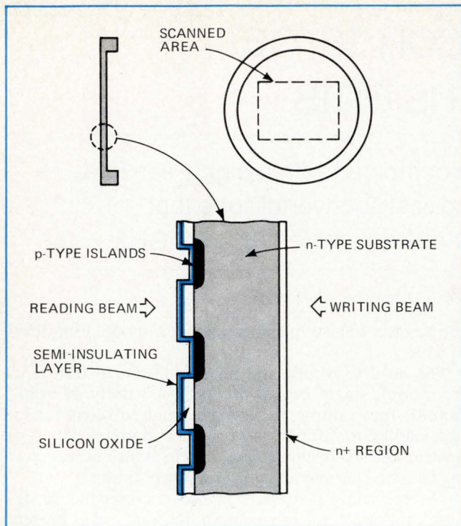
2. The target. Thinned n-type silicon substrate shown in the enlarged view is about 10 micrometers thick. Diffused into its back is a thin + layer that creates an internal field and repels carriers away from the surface. Over the front is a semi-insulating layer that prevents charging of the oxide web surrounding the diodes.
