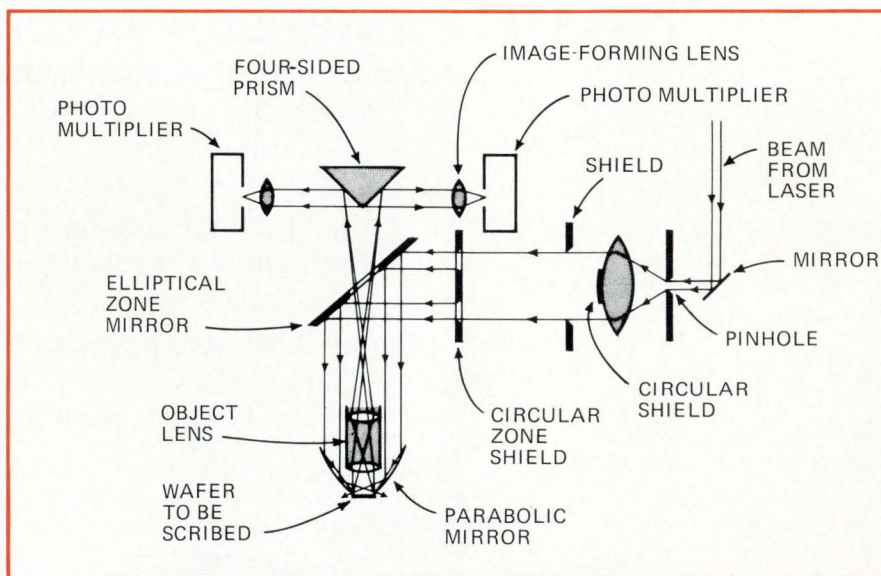
In the fold. Laser beam is bent by mirror before entering optical system that produces a tubular beam. Reflection from wafer goes to four-sided prism used to sense position.
