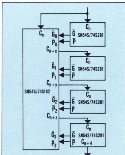
Fast, simultaneous carry generation over any bit length can be achieved by combining S281s and the 54S/74S182 look-ahead carry generator. 16-bit addition time is 27ns, typical.
