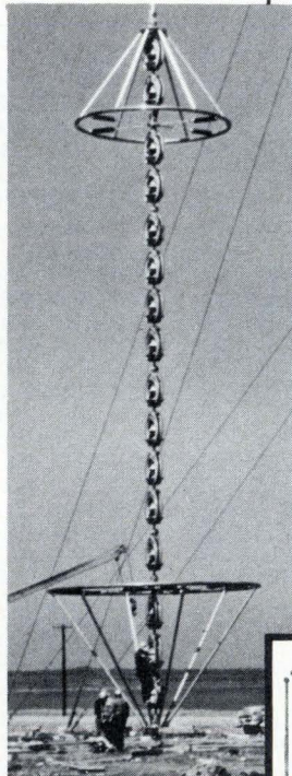
Large structural-guy insulator assembly with grading rings
