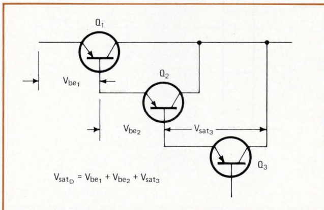
2. Unsatisfactory. Simply cascading three similar transistors gives a saturation voltage that is much too high.
