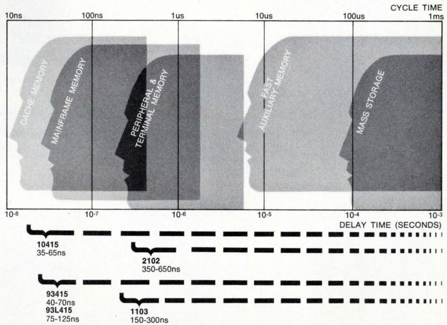
Match-up of Fairchild 1K RAMS with typical memory applications
