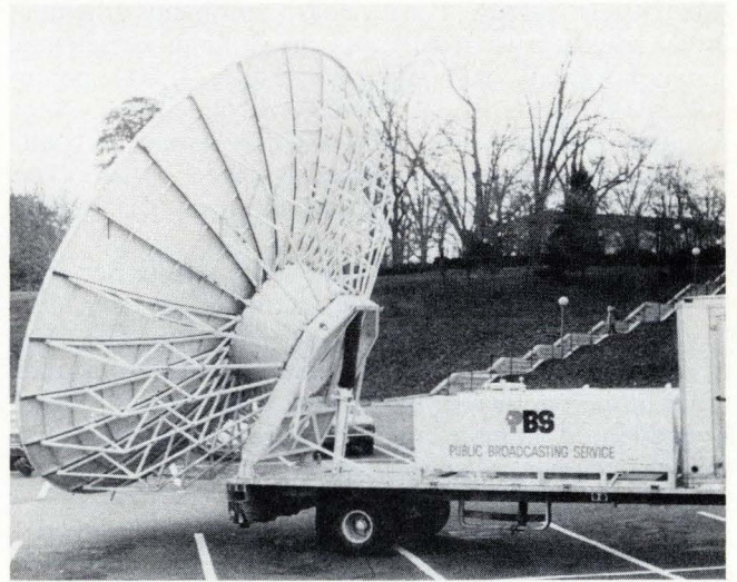
3. TV tests. The Public Broadcasting System used a 10-foot transportable earth terminal for television reception tests from Anik I.
