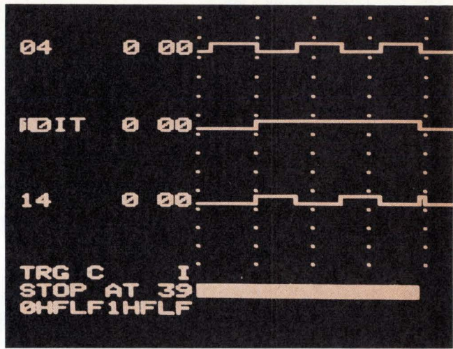
6. Capture. Glitch on trace 14 occurs at the trigger point denoted by end of trigger delay bar at screen bottom. This, teamed with transitions on other channels, could cause a system malfunction.
