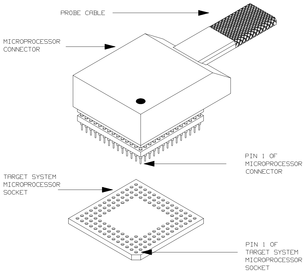
Figure 6-1. Installing Emulation Probe Into PGA Socket
