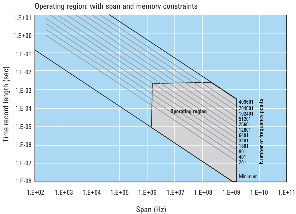
Figure 6. The true operating region is fully described when constrained by all the previous parameters: number of frequency points, span, and oscilloscope memory. See Appendix D for operating region charts for the various supported oscilloscopes.
