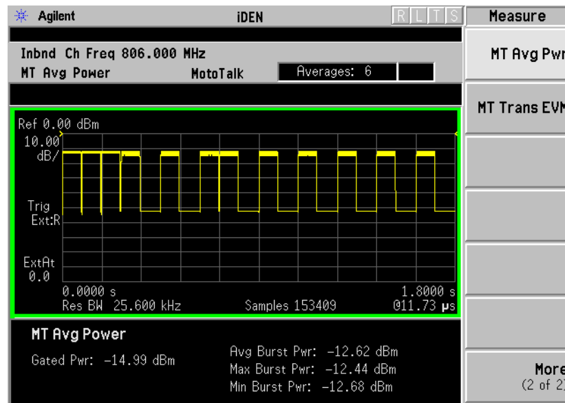
Figure 3-12 Average Power Measurement Results- RF Envelope Window
