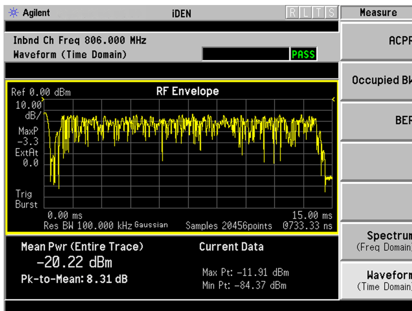
Waveform Measurement Results- RF Envelope Window
