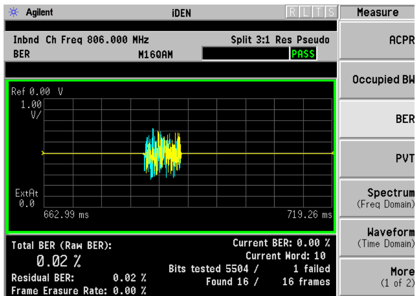
Figure 3-5 WiDEN Bit Error Rate Measurement Results
