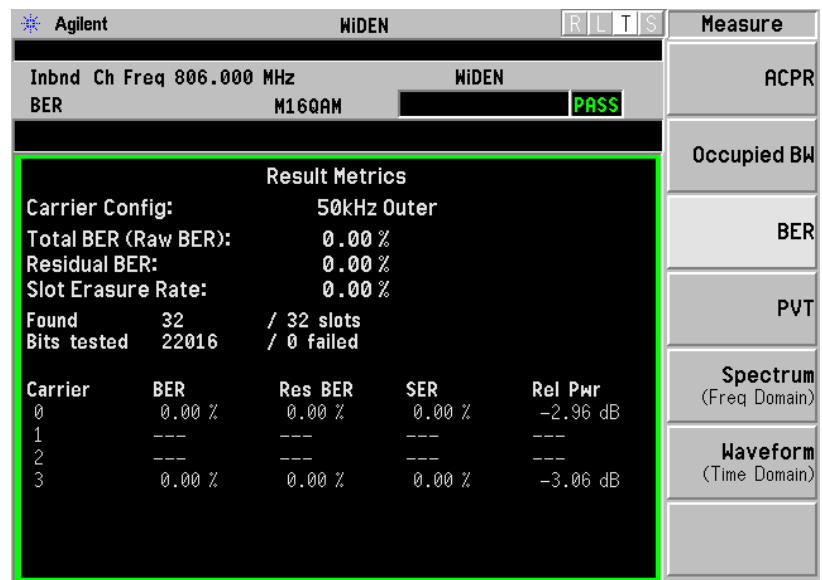
Figure 3-5 WiDEN Bit Error Rate Measurement Results
