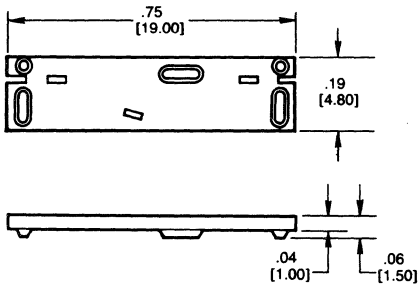
STANDOFF MODEL 700 A
