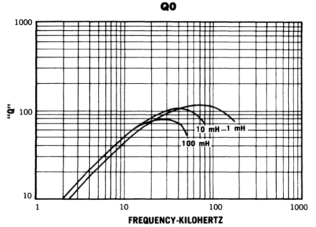
TE-5 and TD-5
