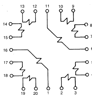
20A03 SCHEMATIC
