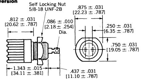
PH-25A Smaller version of PH-25
