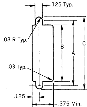
PANEL CUTOUT
