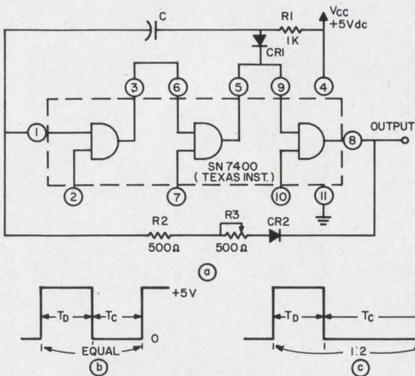
1. Square-wave generator (a) uses charge and discharge paths of capacitor C as timing elements. With R3 shorted, the output is symmetrical (b). As R3 is increased, the symmetry is affected and the pulse is slowed down (c).
