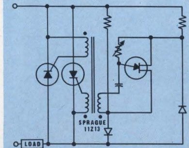
This unijunction-transistor/transformer triggering circuit is a typical application for Type 11213 Trigate Pulse Transformers.
