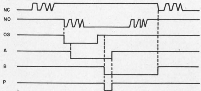
2. These waveforms result when any switch is depressed.
