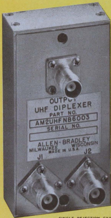
SINGLE REJECTION CAVITY TYPE DIPLEXER—COMPARABLE TO A PACK OF REGULAR SIZE CIGARETTES IN SIZE
