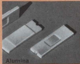
Alumina Length .760 \pm .005 Thickness .050^{+.005}_{-.000} Counter Bore Depth .008^{+.003}_{-.000}
