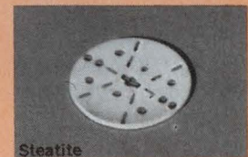
Steatite O.D. .636 \pm .007 Thickness .046^{+.002}_{-.000} Hole .042^{+.002}_{-.000}
