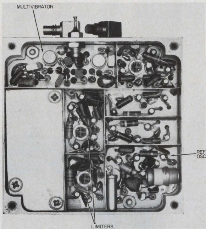
6. Modulator, built according to the circuit of Fig. 2, performs as a frequency source for telemetry transmitters in both the vhf and uhf regions.
