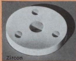
Zircon Center Hole I.D. .258 - .259 Grinding on 5^\circ Angle leaving .258 - .259 dimension .032 \pm .005 long
