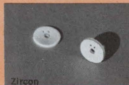
Zircon Thickness .030 \pm .002 I.D. .060 \pm .001 Two Holes .020 \pm .002 Hole Center .054 \pm .002 O.D. .273 \pm .001 Ground
