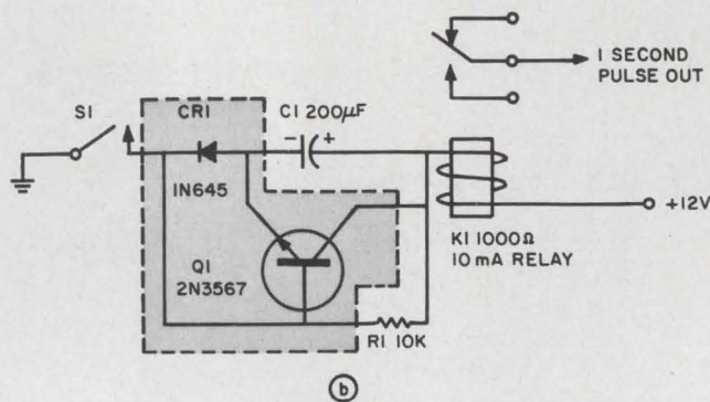
Improved operation can be obtained from the simple pulsing circuit (a) by the addition of a transistor-diode combination (b) which allows greater variation of pulse widths.
