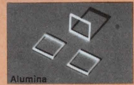
Alumina O.D. .250 Square Wall Thickness .015 \pm .002 Thickness .018 \pm .001
