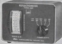
REFLECTOMETER Mod. 369 .. $115
