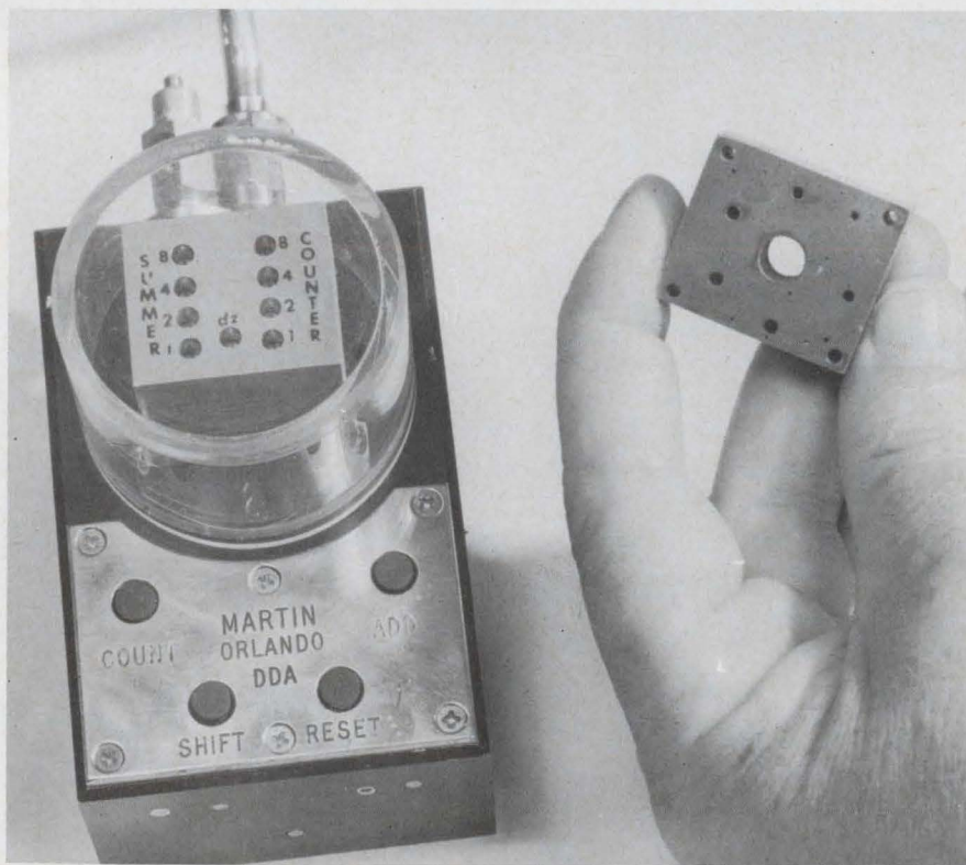
Digital differential analyzer can calculate areas under simple curves.
