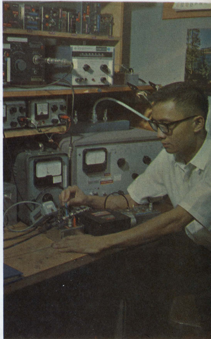
Noise figure measurements on an rf FET mixer are made by Siang Pink Kwok of Motorola Semiconductor, Inc. (Paper 8/1).
