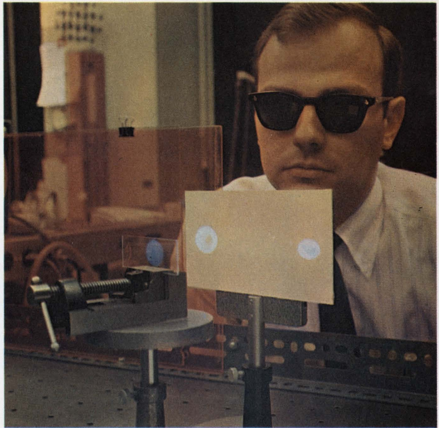
The two bright areas on the card illustrate the high efficiency—over 90%—with which a simple pattern formed in a new holographic material, dichromated gelatin, diffracts a laser beam directed by T. A. Shankoff of Bell Laboratories. The company hopes to store up to 10^8 data bits holographically on a glass slide coated with the emulsion.
