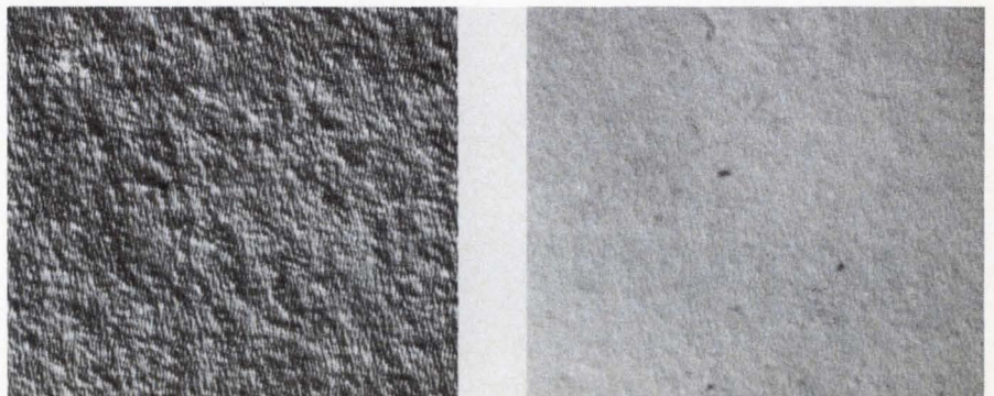
Chemically etching the emulsion gives a smoother surface (right) than conventionally processed hologram, as seen under 250X magnification. This technique is claimed by IBM to give phase-type holograms that diffract 40% of the laser beam into usable reconstructed images. Previous claims of 40% were accompanied by poor S/N.
