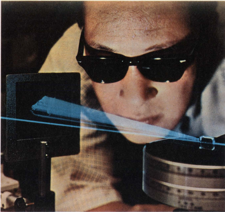
Lithium niobate crystal stores as many as 1000 holograms—but potentially many more—in a lithium niobate crystal. Fong Chen of Bell Laboratories reconstructs one such image. To get a new one, he simply changes the angle at which the laser beam enters the crystal.
