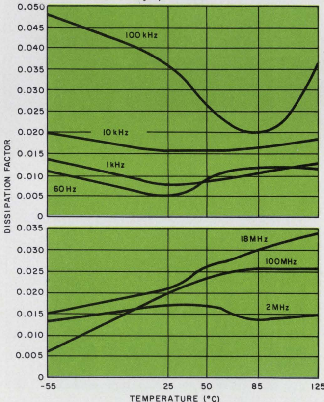
6. Effect of frequency and temperature on the dissipation factor of unfilled diallyl phthalate is shown for a frequency span of 60 Hz to 100 MHz.
