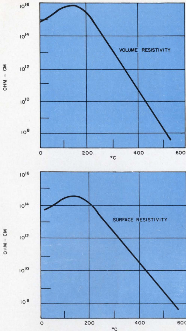
18. Resistivity as a function of temperature is shown for a representative glass-bonded mica. Values for both volume resistivity and surface resistivity are given.
