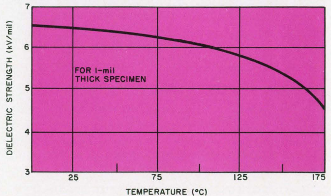
27. Important electrical properties of polyimides as a function of temperature.
