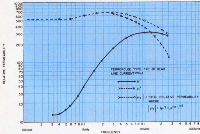
4. Total bead permeability, \mu_T , consists of a real component, \mu' , and an imaginary component, -j\mu'' .
