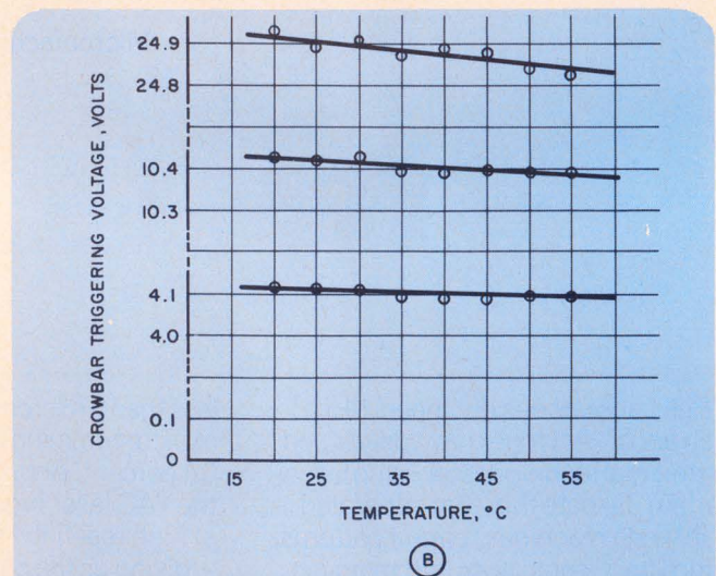
The SCR turns on, providing crowbar protection for the load, when the base voltage of Q_3 exceeds that of Q_2 (A). This turn-on voltage is exceptionally stable with temperature (B).
