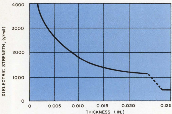
DIELECTRIC STRENGTH
