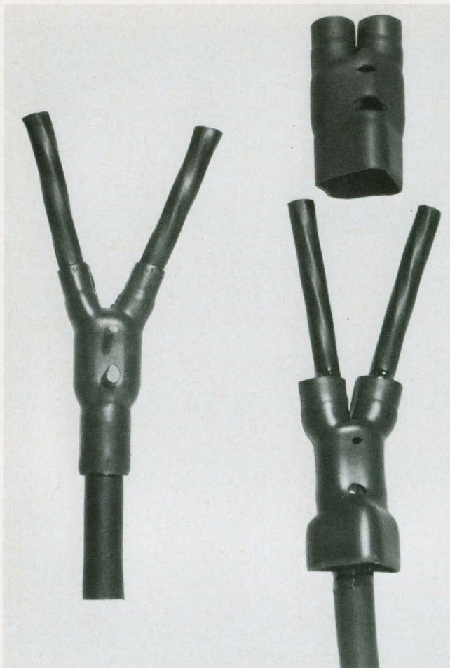
26. Irradiated, cross-linked polyolefins find use as heat-shrinkable cable boots. After being set in place, the oversized boot is heated, shrinking tightly around the cable. (photo courtesy Rayclad Tubes, Inc.)
