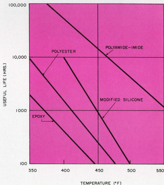
28. Thermal life of amide-imide wire enamels compared to other electrical insulation coatings.
