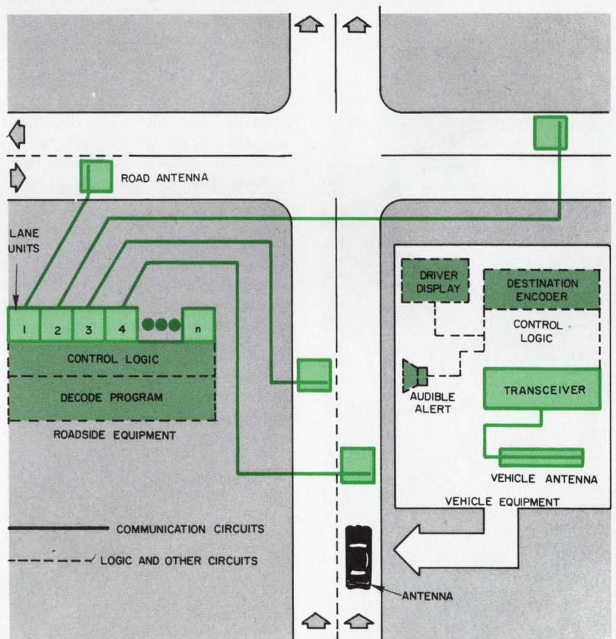
A driver approaching an instrumented intersection transmits a destination code to a roadside unit via a road antenna. The unit interprets the code, compares it with stored data and then transmits appropriate instructions to the driver, either to continue straight ahead or change directions at the next intersection.
