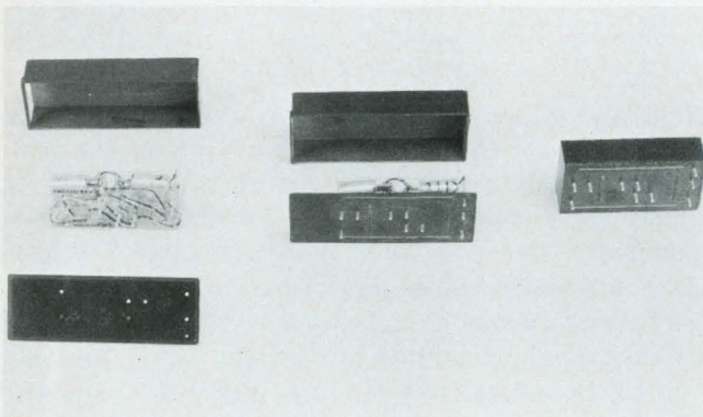
9. Epoxy molding material can be used for module cases (left), as well as for directly molded modules (right). (photo courtesy Westinghouse Electric Corp.)
