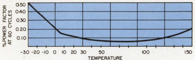
POWER FACTOR
