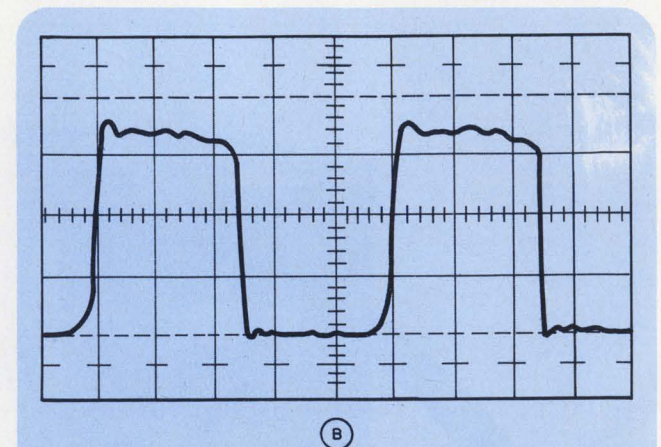
Frequency of the square-wave generator can be changed by changing the values of C_1 and C_2 . Output waveform from the circuit is shown in (b). Sweep speed was 0.1 \mu\text{/div} and sensitivity 1 V/div.
