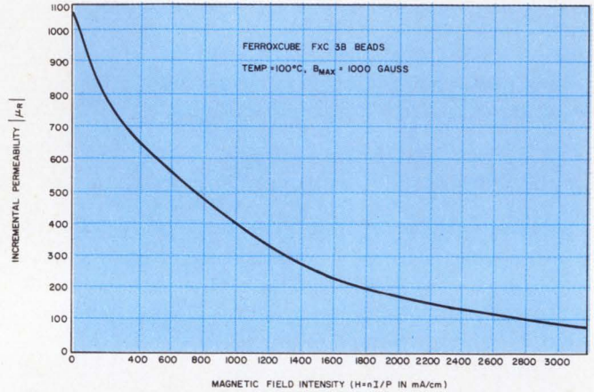
5. Line current, I , has a significant effect on the permeability of a ferrite bead.
