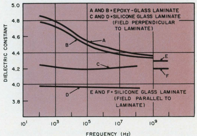
12. Dielectric constant vs frequency at room temperature for silicone-glass and epoxy-glass laminates.
