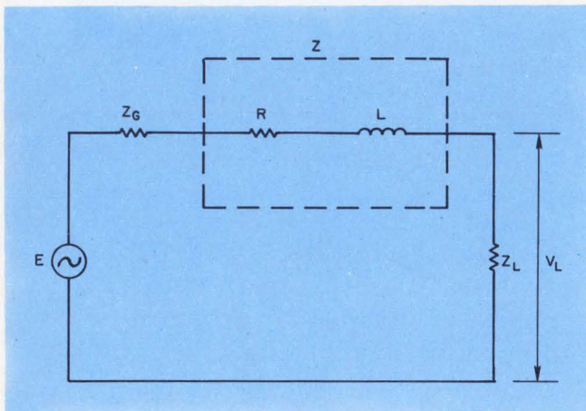
6. When a bead is placed on a line, the impedance, Z , of the bead and line adds to the existing circuit impedances, Z_G , and Z_L .
