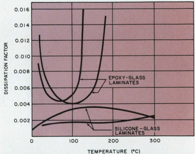
11. Dissipation factor vs temperature for silicone-glass and epoxy-glass laminates.
