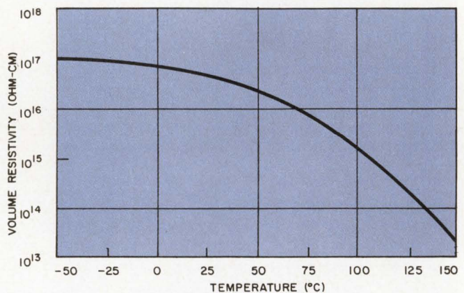
VOLUME RESISTIVITY
