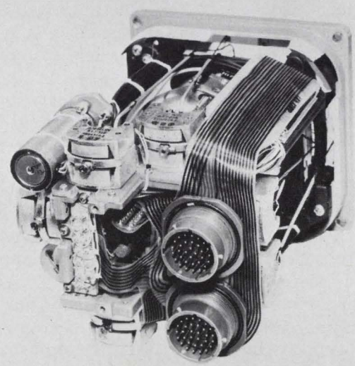
24. Capabilities of FEP flexible printed circuits for compact applications are apparent from the Sperry Phoenix Attitude Director Indicator, viewed here from the rear. (photo courtesy DuPont Corp.)
