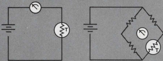
Circuit A
