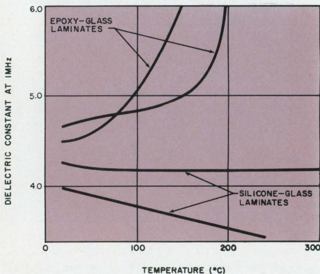
10. Dielectric constant vs temperature for silicone-glass and epoxy-glass laminates.
