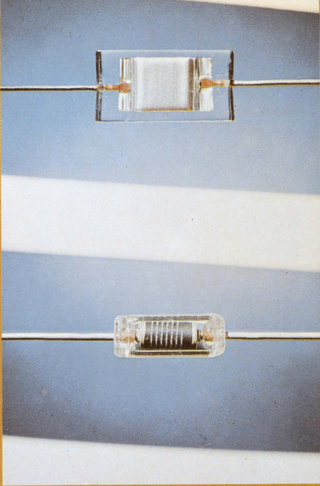
Glass is used as a sealer for this resistor and capacitor. The resistor element itself is a glass rod onto which a tin-oxide film is fused. (photo courtesy Corning Glass)
