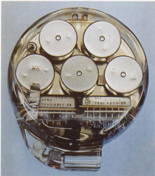
Meter readers use RCA circuits in several ways. In one, a CMOS memory stores the reading until needed. Manual reading, used in conventional billing, is eliminated.
