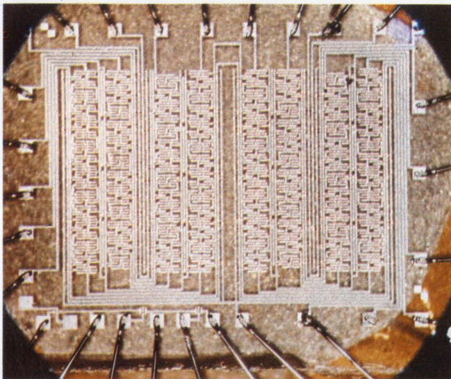
A test array from RCA uses SOS techniques for increased speed. The circuit contains a dual eight-stage digital parallel correlator that operates to 45 MHz.
