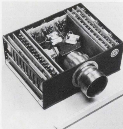
A prototype color TV camera that uses three 220-by-128-element, charge-coupled-device arrays has been built by Bell Laboratories.
