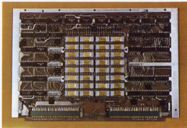
AMI's 512-bit static RAM—the largest in CMOS—is used in Rolm's memory board for the Rugged Nova minicomputer. The AMI memory features an access of 200 ns and an operational dissipation of 5 \mu W/bit.
