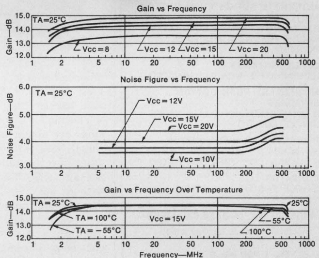
WJ-A5 TYPICAL PERFORMANCE
