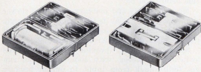
Low-profile relays that use permissive-make contacts are designed for tightly spaced printed-circuit boards. These relays are from C. P. Clare.
