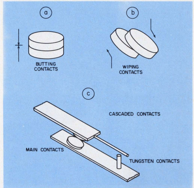
1. When you select a reed relay, check the type of contacts. You can get butting contacts (a), wiping contacts (b) or cascaded contacts (c).
