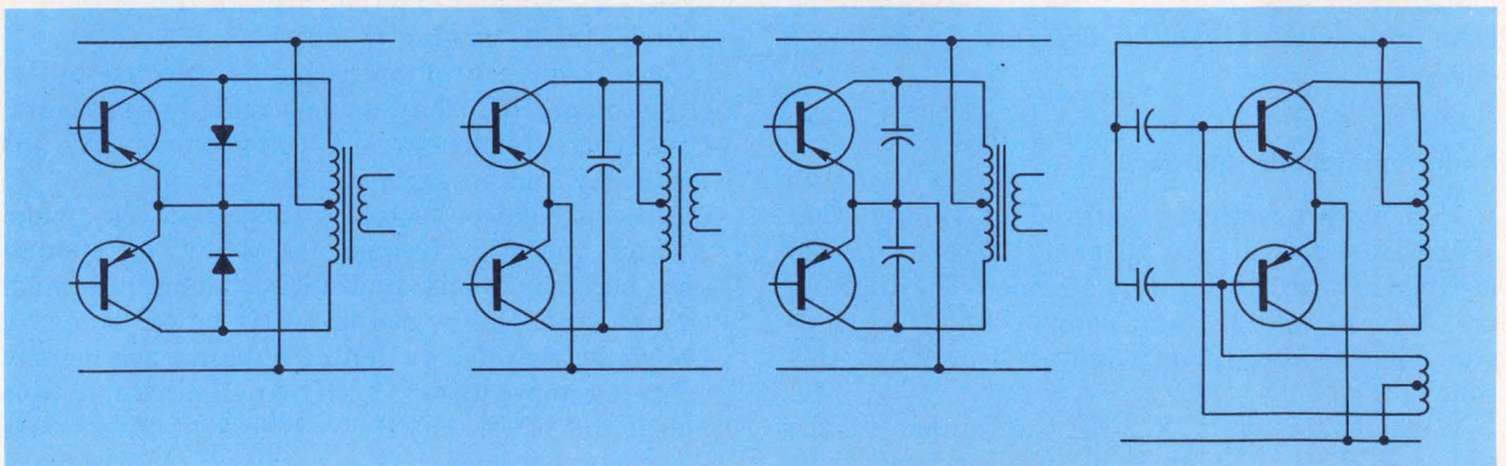
5. Transient spike-suppression networks can be added at various points in the converter. Either diodes or ca-
