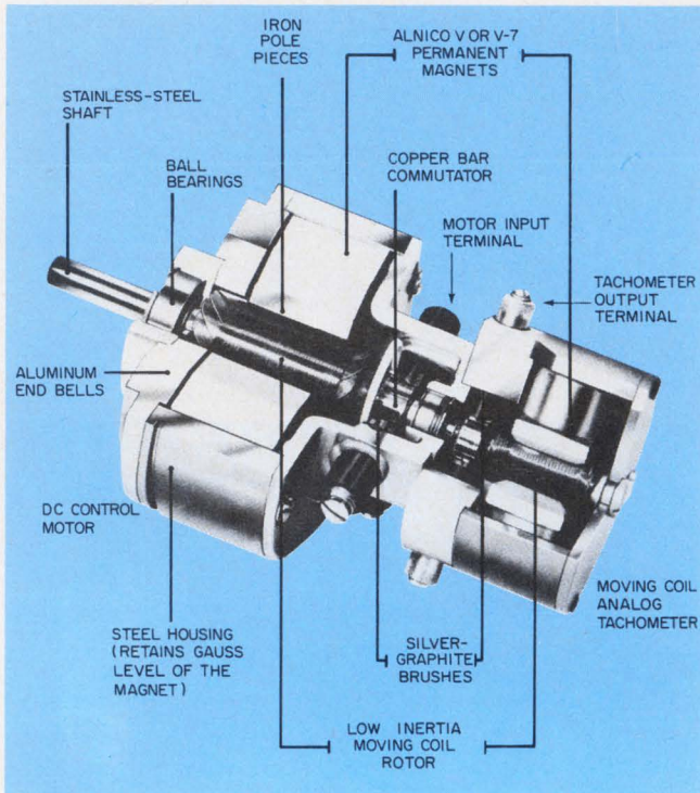
3. A hollow-rotor, permanent-magnet motor with a built-in tachometer for velocity feedback makes a convenient package for a speed-servo system.
