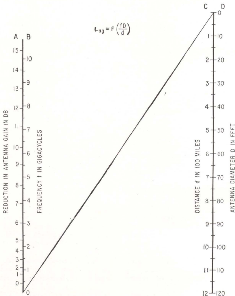
ANTENNA EFFECTIVENESS depends upon operating range as well as antenna physical characteristics; chart gives antenna gain reduction in terms of operating parameters—Fig. 1
