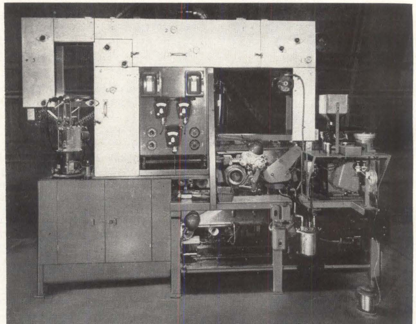
CONTINUOUS automated process for making radial lead resistors uses specialized equipment. Developed by Wilrite Products, it is modeled after equipment used by Centralab for making radial lead ceramic capacitors
