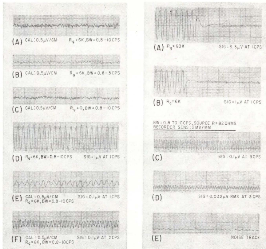
SEISMOMETER RECORDINGS show that high-impedance coils (A) can provide better S/N than low-impedance coils (B). Step-up transformer can enhance S/N and sensitivity of low-impedance seismometer coils (C, D and E)—Fig. 4
