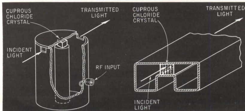
REENTRANT-CAVITY modulator (left) and traveling-wave modulator using cuprous chloride (RCA)
