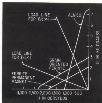
DEMAGNETIZATION section of hysteresis curve demonstrates ability of ferrite to retain field strength—Fig. 3
