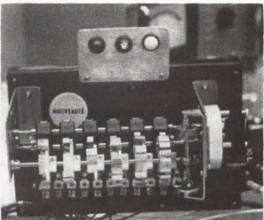
PROGRAM switch uses unusual drive developed by Alkan & Sinay
