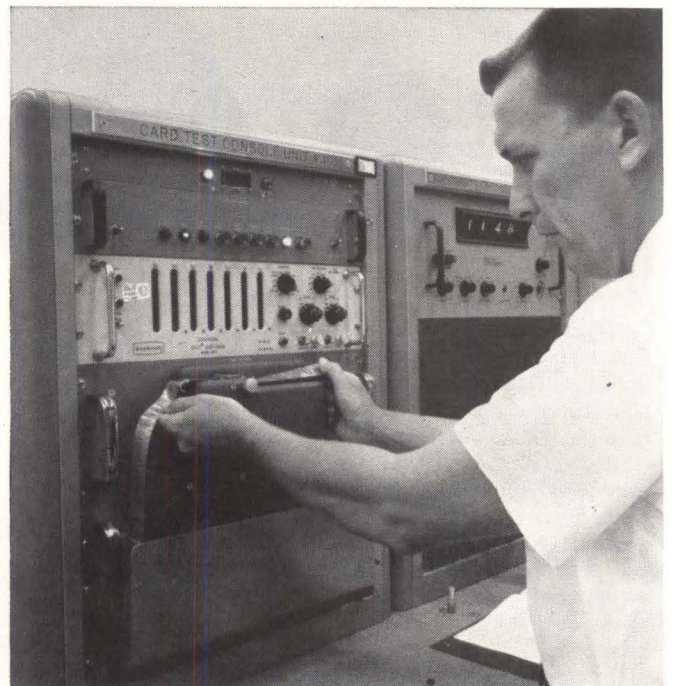
Carle W. Collins, production test engineer, Martin Company's Orlando (Fla.) Division, inserts coded Mylar tape into the reader unit of the Tape Programmed Automatic Tester which he designed.
