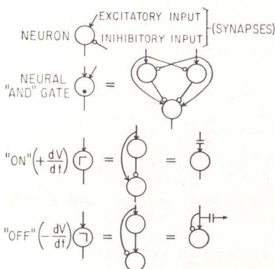
NEURON SYMBOLS and equivalent circuits—Fig. 1
