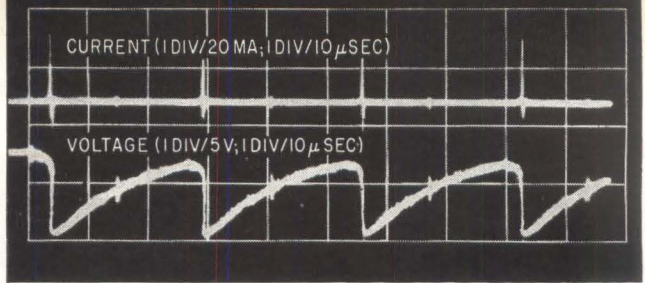
EXPERIMENTAL NEURISTOR STORAGE RING (left) and scope traces (right) of voltage and current of element of ring when a pulse is stored in it
