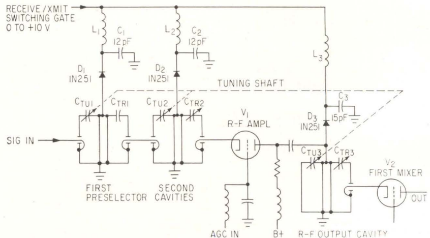
PROTECTIVE CIRCUITS and receiver's front end. A gate input (upper left) switches capacitors C_1 to C_3 across tuned cavities, thus detuning them and desensitizing receiver—Fig. 1
