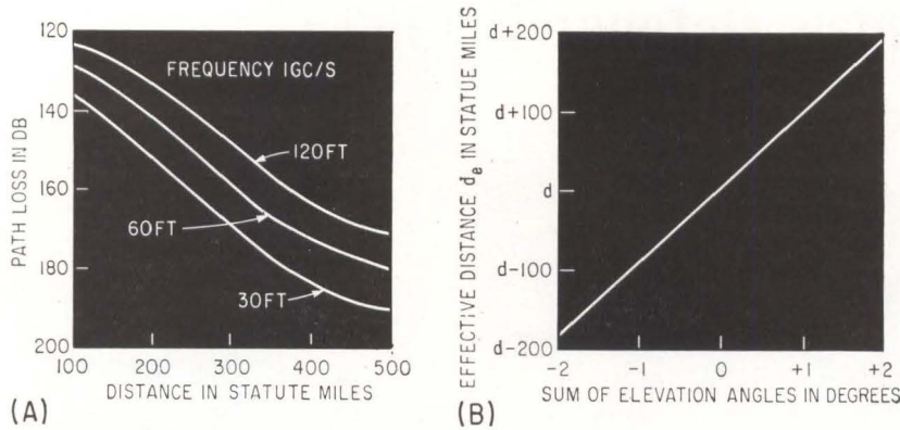
(A) DIVERGING CURVES show that large diameter antennas have relatively increased performance at long range (A), effective operating distance related to algebraic sum of terminal elevation angles (B)—Fig. 2
