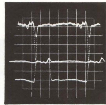
CURRENT LEVELS in the threshold tunnel diode. Waveforms (3.3 nsec per cm) are taken across the threshold tunnel diode for signal currents below and above the threshold level (upper trace); across the memory tunnel diode (lower trace)—Fig. 4
