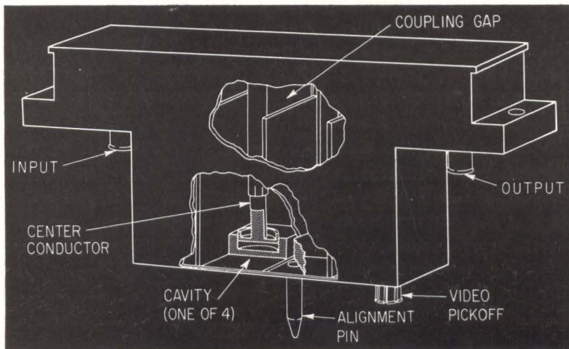
FOUR-SECTION FILTER sketch. Internal view shows center conductor of one of the four sections of the filter—Fig. 3
