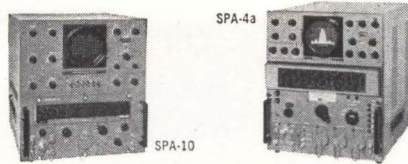
MICROWAVE SPECTRUM ANALYSIS 10-64,000 mc
