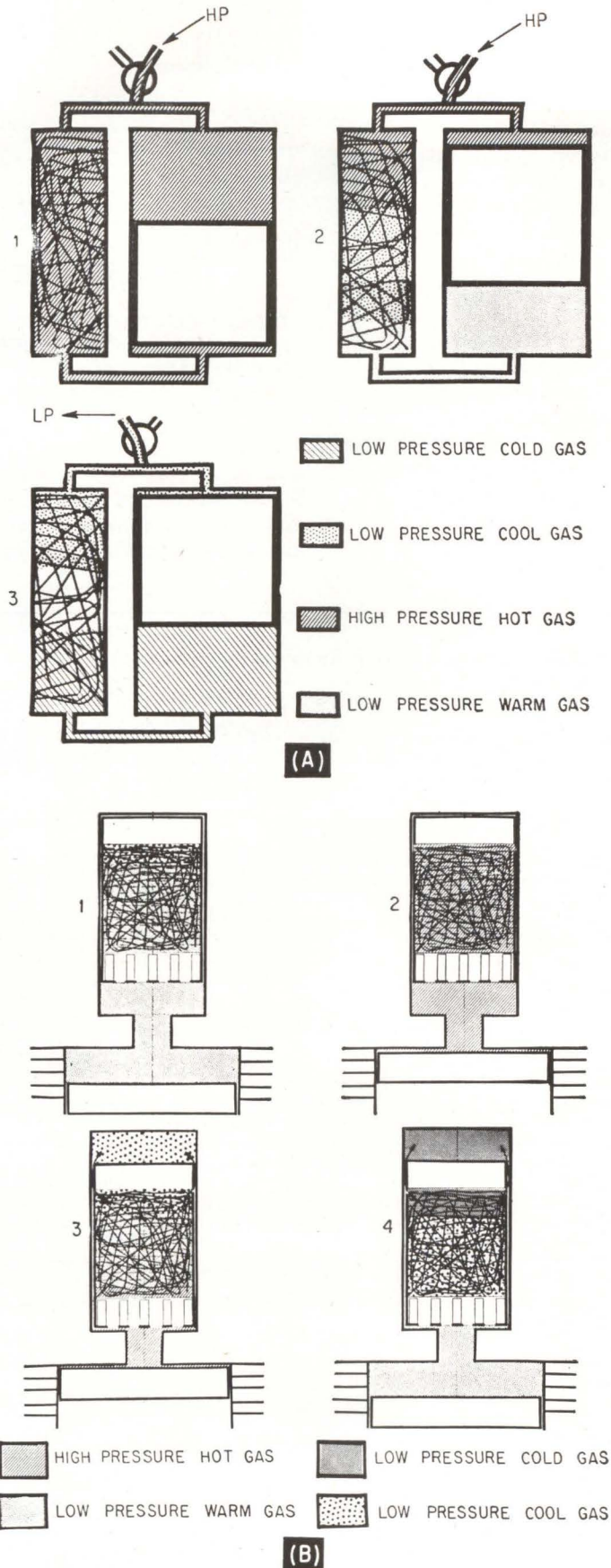
DISPLACER REGENERATOR piston displaces gases in and out of regenerator previously cooled by adiabatic expansion (A). Hybrid cooling system is most efficient for the range of -80 to -180^{\circ}\text{C} (B)—Fig. 5
