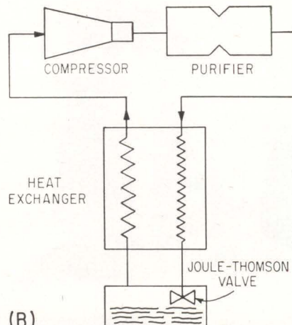
CARNOT CYCLE diagram is a reference for refrigeration-cycle efficiency (A) Regenerative liquifying process must take place below the inversion temperature of the working gas (B)—Fig. 3
