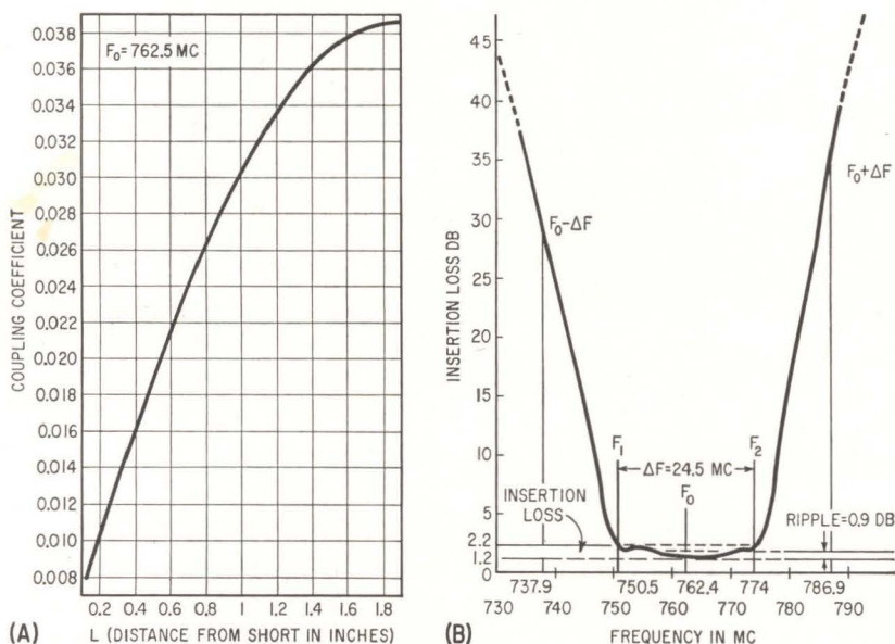
COUPLING COEFFICIENT is plotted against gap in (A). The response curve of a filter that was fabricated according to data of (A) is shown in (B)—Fig. 2
