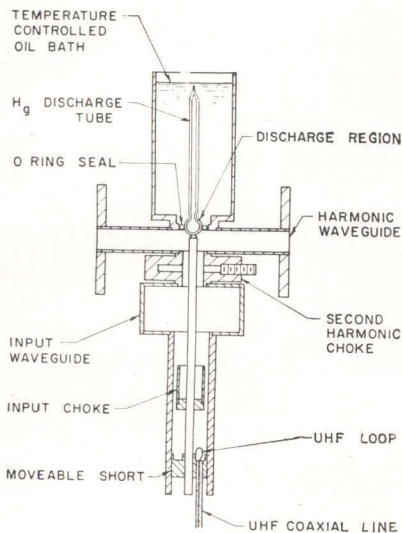
PLASMA-DISCHARGE generator used at Stanford to observe harmonic output and parametric oscillations in a spherical r-f discharge
