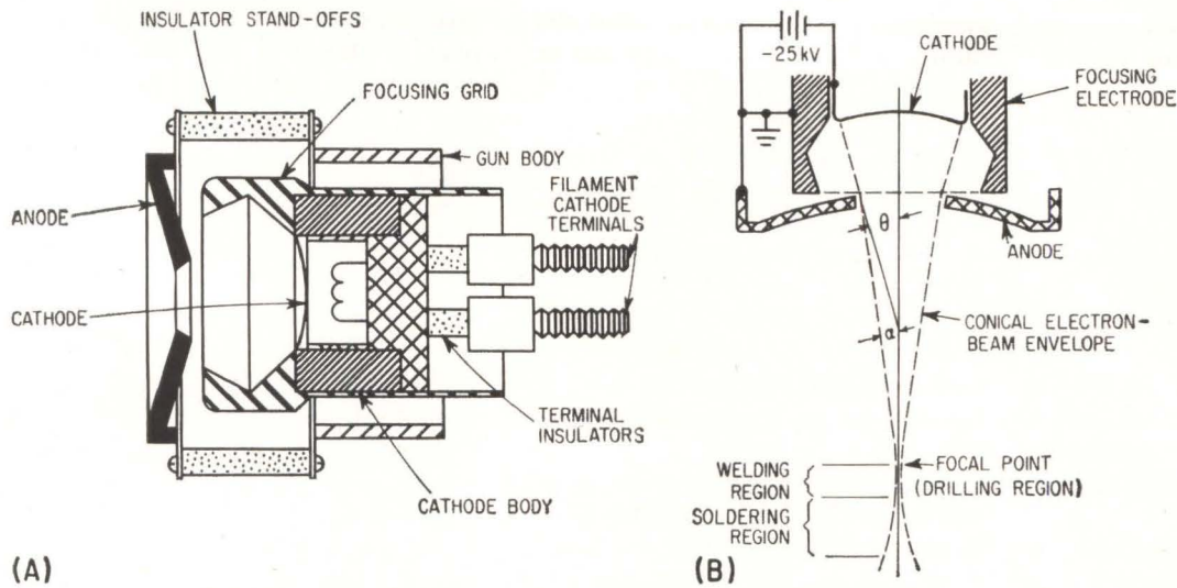
ELECTRON GUN (A) and electron beam envelope (B), showing the relationship of the gun electrodes required to obtain a sharp, electrostatically-focused beam—Fig. 2
