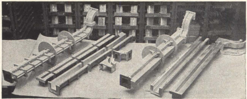
OLD UNIT (left) was made up of castings matched to form a continuous, unbroken channel. New unit (right) requires less milling and hand labor
