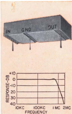
High frequency low pass filter. Zero to 700 KC within 1 db. 1.95 mc to 10 mc 40 db minimum. Source and Load 1000 ohms. Molded flat construction for printed circuit applications. Size: 1 x 2 x 1/8"; Wt: 1 oz. MIL-F-18327B.
