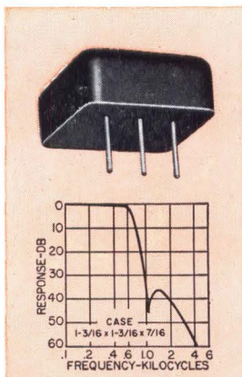
560 \sim Telemetering low pass filter. Available from 400 \sim to 70 KC. \pm 7.5% bandwidth flat to 1 db. Attenuation greater than 35 db beyond the 2nd harmonic of 7.5% frequency. Impedance 47K ohms. MIL-F-18327B. Wt. 0.8 oz.
