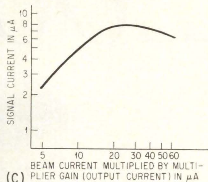
LIGHT-TRANSFER CHARACTERISTICS of the pickup storage tube (A); plot of S/N ratio and noise current as a function of beam current (B); signal output as a function of beam current (C)—Fig. 5
