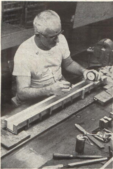
HAND LAPPING was used to obtain critical surface tolerances with old design
