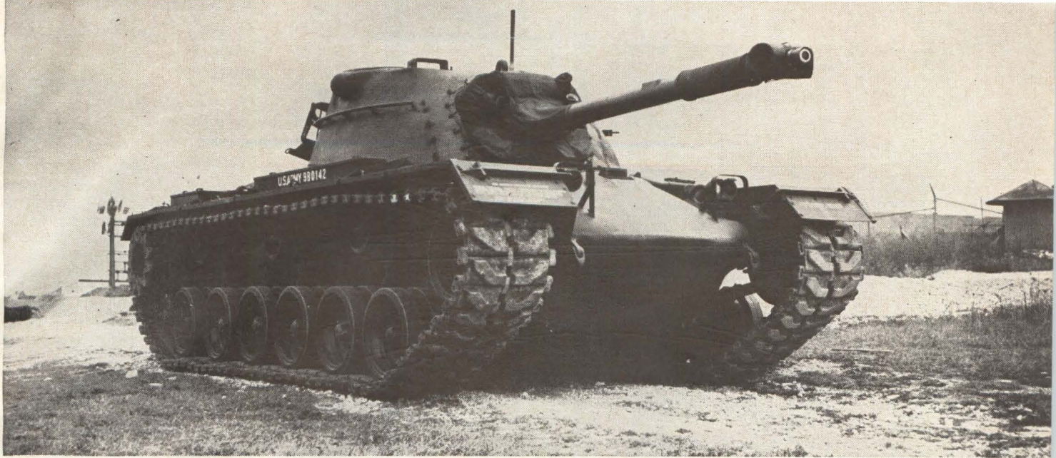
INFRARED photoelectric telescope is mounted in the M-48's gun. Radio antenna and infrared beacon assembly are mounted atop the turret
