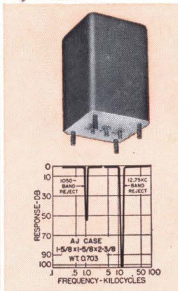
Band reject filters (two shown). The 1050 \sim filter has 50 db attenuation and is only 3 db at 950 and 1150 cycles. The 12.75 KC filter has more than 100 db attenuation and is only 3 db at 10.8 and 15 KC. Source and load 600 ohms, both are MIL-F-18327B.
