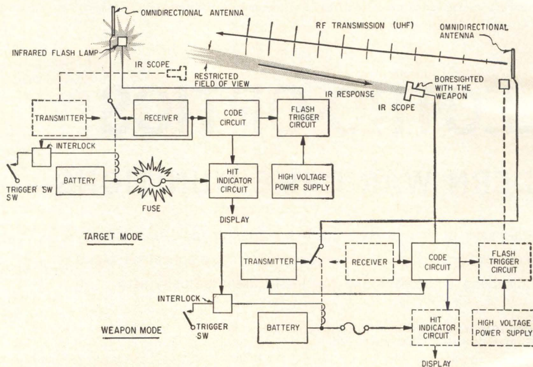
TARGET-WEAPON MODE for simplified hit indicator system. Pulling trigger turns-on weapon's transmitter and connects it to antenna. Target's weapon is locked-out of weapon mode. R-f signal blows a disabling fuse gun—Fig. 2
