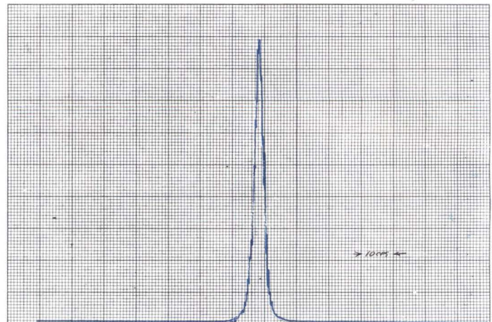
Spectral Purity —This power spectrum shows the excellent spectral purity of the hp 107A Quartz Oscillator. The output was multiplied to 24 gc, compared with the NBS ammonia maser, and the beat note analyzed using a narrow bandwidth analyzer. The vertical axis is in units of power, each division on the horizontal axis is 10 cps, analyzer bandwidth is 3 cps. Note the virtually nonexistent noise pedestal, narrow line width, and the absence of power line sidebands even when multiplied nearly 5000 times.
