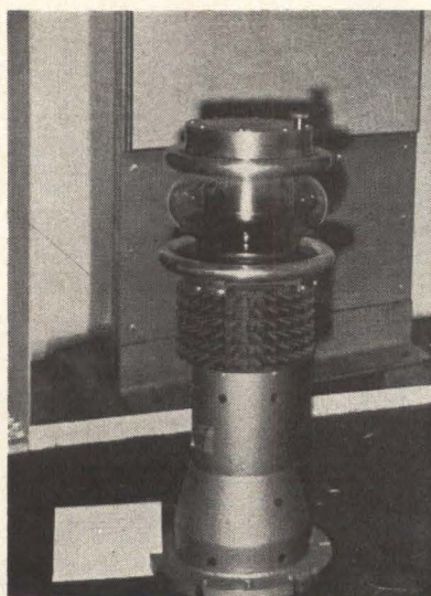
HEDGEHOG EFFECT at middle of tube is the magnet assembly and cooling fins of CSF's Artatron
