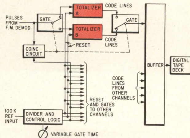
Two totalizer counters alternately sample analog data to permit high sampling rate with maximum accuracy.
