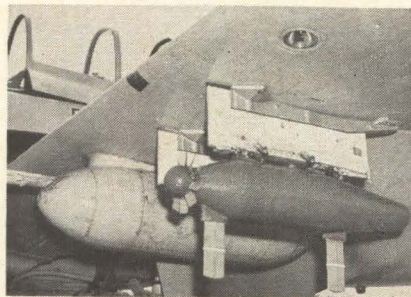
Airborne relay pod (foreground) , hung on the wing of an Air Commando aircraft, extends the range of a 10-watt ground station up to 180 miles. Built by the Radio Corp. of America, the uhf pod is one way to beat the problems of line of sight and of radio signal attenuation in the jungle.
