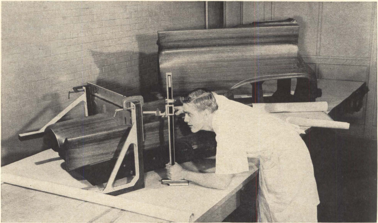
After clay, what? Wood carvers spend weeks carving accurate machogany exterior quarter panels and other parts. These are used for templates to make production dies. The same process takes only a few hours with tape control.
