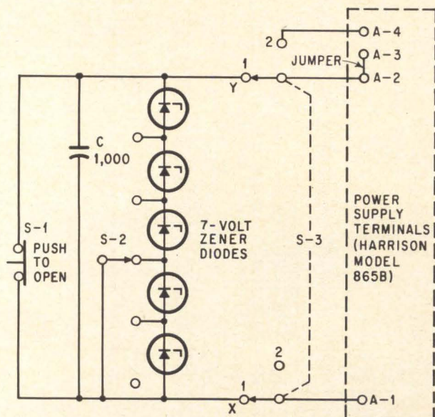
Addition of a 1,000- \mu f, 50-volt electrolytic capacitor to a standard transistor power supply allows slow voltage sweeping for classroom demonstrations.
