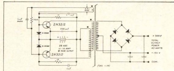
Miniature converter in which 2N3212 high gain, high current and fast switching speed characteristics provide a 40-watt output at an efficiency of over 87 percent.
