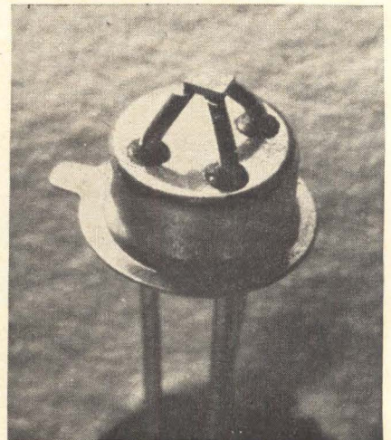
Chip sits on tripod formed by leads.
