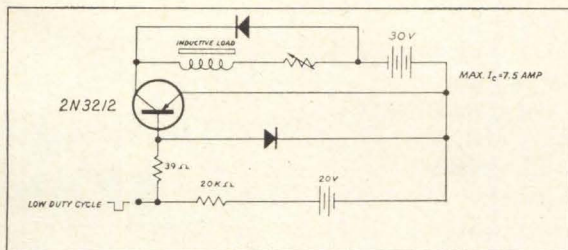
Miniature Solenoid Driver: Excellent high current gain of 2N3212 enables intermittent operation of solenoids at high currents such as 7.5 amperes. Duty cycles of 1 millisecond at 15 millisecond repetition rates are typical.
