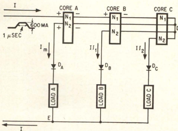
Current-steering circuit
