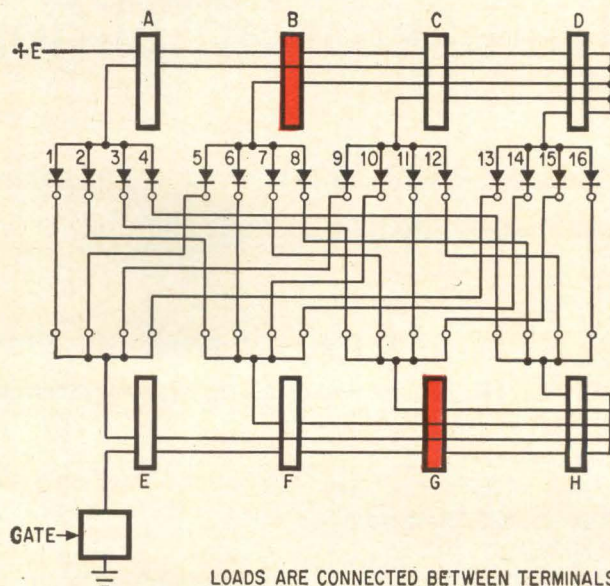
Memory addressing circuit
