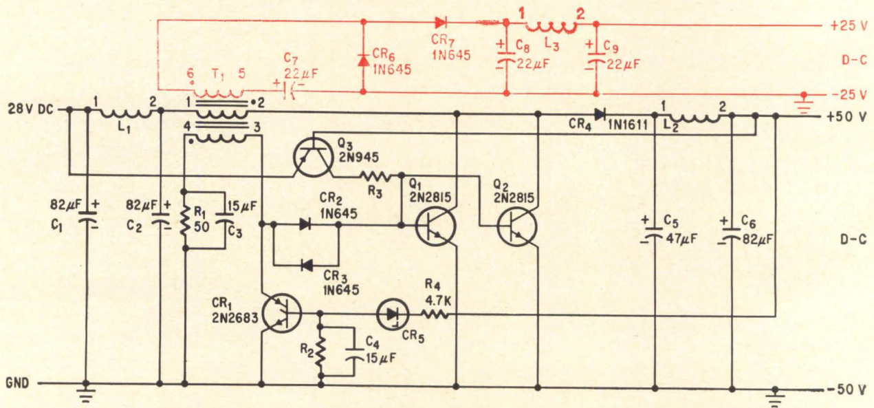
Power supply used on 28-volt d-c source produces both 25- and 50-volt d-c outputs.
