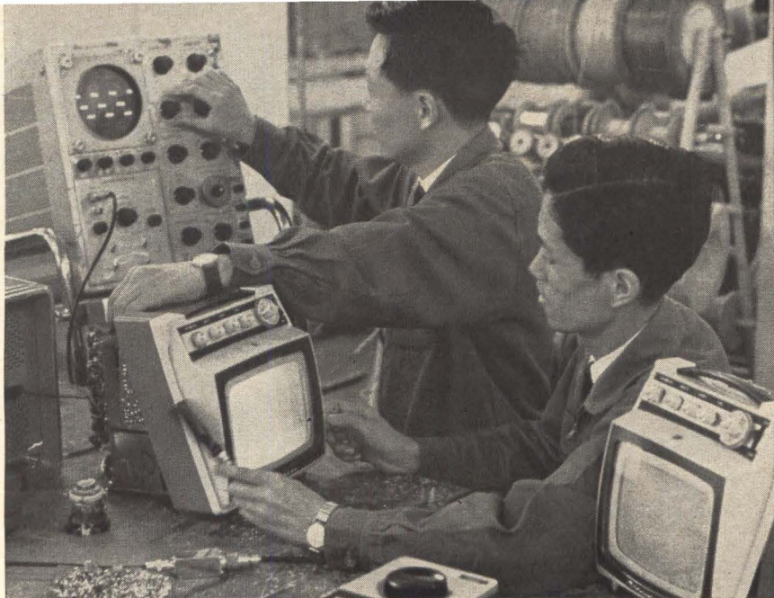
Vhf tuner for Yaou color set is aligned. Response curve is seen on scope.
