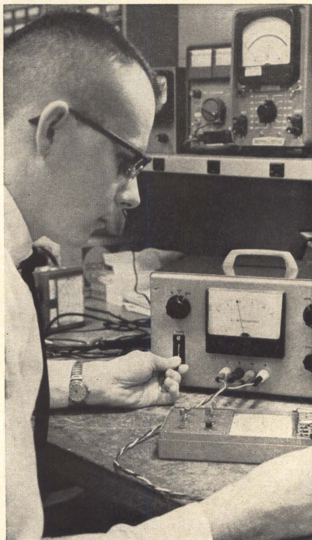
Typical test setup for measuring leakage current. Colored line shows extra bootstrap lead required for checking decoupled stage.
