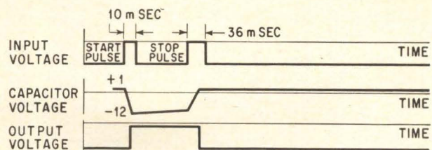
Waveforms for interrupted delay operation.
