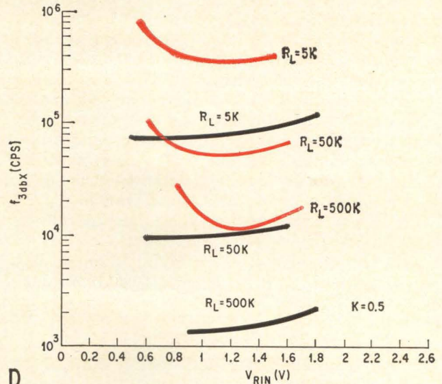
Power drain of circuit designed with a given resistor-tolerance margin can be minimized by adjusting the d-c emitter feedback voltage, V_{Rin} (A). Power drain of cascode amplifier (colored curves) is less than twice the drain of the common-emitter amplifier (B), while there is less than 1 db difference in power gain between the two circuits (C). Key advantage of cascode stage over common-emitter amplifier is the increased bandwidth (D).
