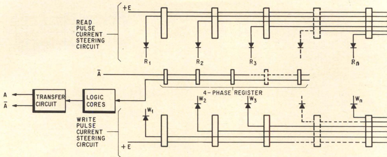
Current-steering circuits for register read-write pulses
