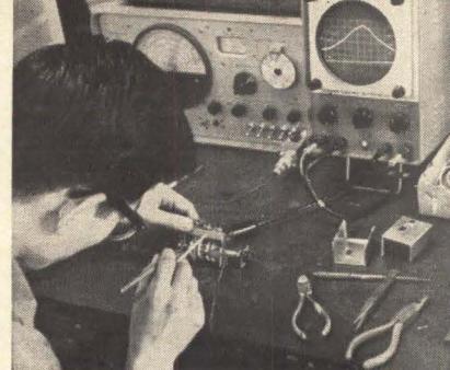
Vhf tuner for Yaou color set is aligned. Response curve is seen on scope.
