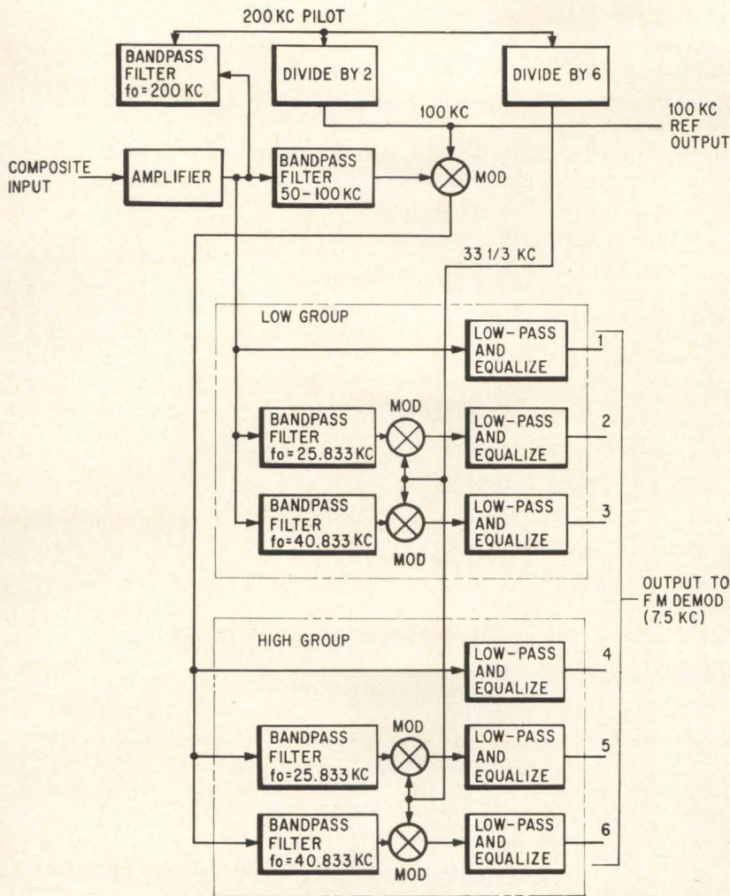
Reverse process of the multiplexer separates the six signal channels.
