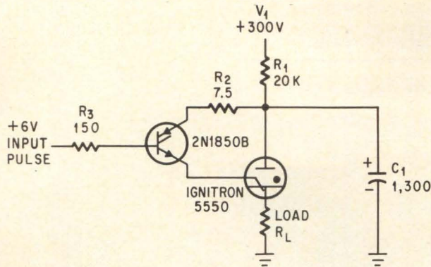
A Silicon controlled rectifier replaces a thyatron conventionally used to fire an ignitron.
