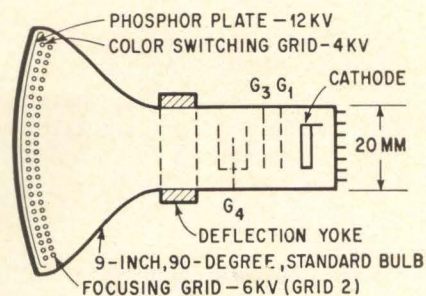
Locations of grids in tube
