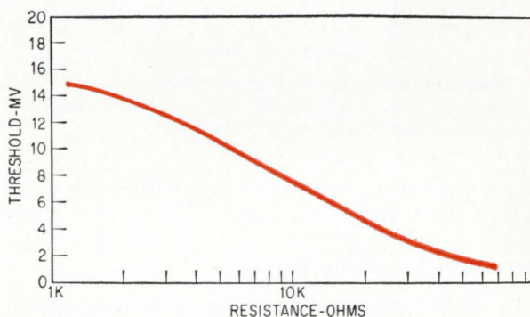
Threshold voltage can be varied by changing the resistance between pin I and ground.
