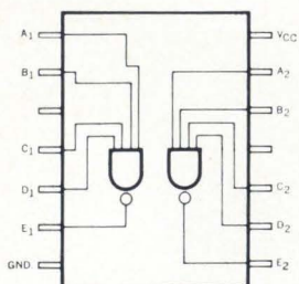
9004 Dual 4-input positive NAND gate.
