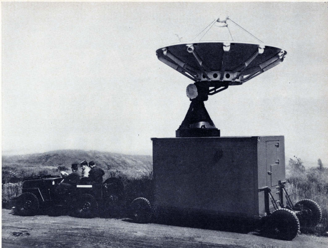
Sylvania's satellite communication terminal is one of the most mobile ground stations ever built. Weighing only two tons, it is readily transported by truck or helicopter. Three men can set it up in less than an hour. When used with Syncom III, this terminal provides one duplex voice channel and 16 simultaneous teletype channels.
