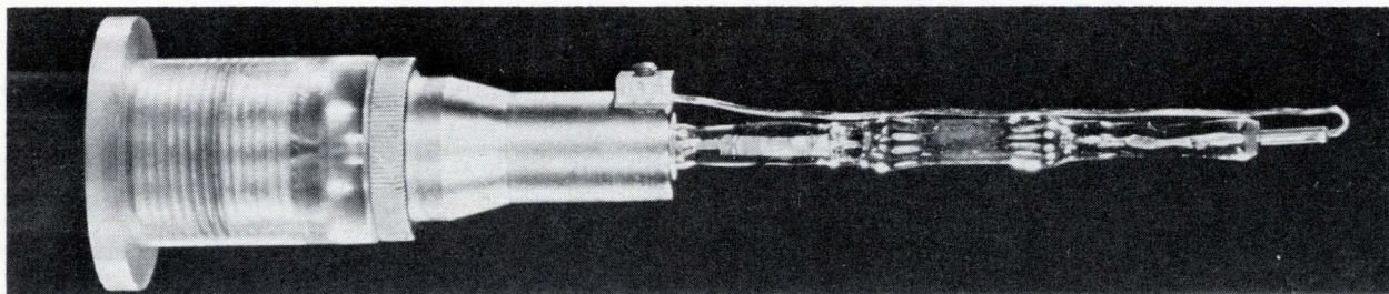
Ruby laser with repetition rate of 100 hz uses ellipsoidal pumping mirror, 1-inch-long ruby rod, high-pressure mercury-vapor flashtube. Absolute output efficiency is 0.22%. Flashtube, in photograph has preadjusted, interchangeable holder and electrical plug-in. It can be produced cheaper than xenon units.
