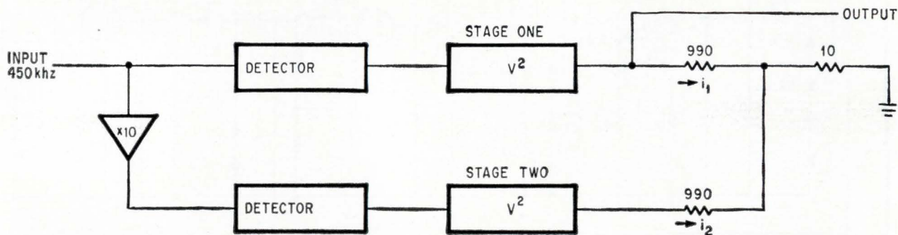
The 40-db input range of the diode detector is split into two 20-db segments, thus avoiding high-frequency saturation, low-frequency drift and nonlinearities inherent in other diode networks. Both stages are identical and operate at levels that produce the two segments. When matched, the stages give the proper output function by means of input amplifiers and output attenuators.
