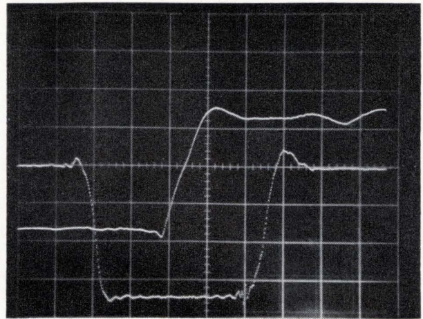
A 17-millivolt input pulse 100 nanoseconds wide (left) produces a negative output pulse less than 60 nanoseconds later. A similar pulse (right) can produce a positive output pulse with a similar propagation delay.
