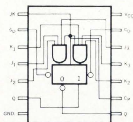
9000 J-K Flip-Flop: master-slave (dual rank) flip-flop with 3 J and 3 K inputs, J-K input, internal J-K connection, positive edge trigger, data input inhibit line (clock pulse), and asynchronous direct inputs to set and clear FF.
