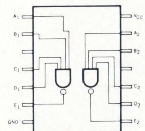
9009 Dual 4-input positive NAND "Power" gate.
