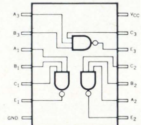
9003 Triple 3-input positive NAND gate.
