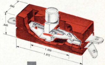
E13-00E GENERAL PURPOSE 15 amp, 125-250 VAC ¾ H.P. 125 VAC 1½ H.P. 250 VAC
