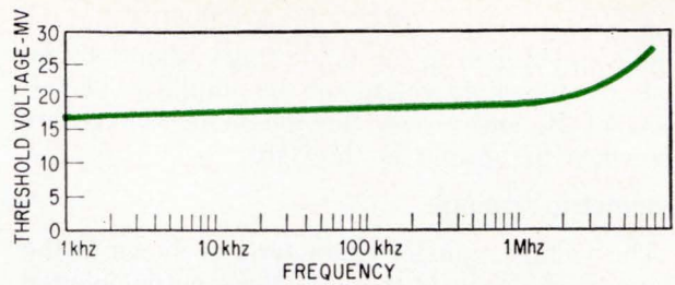
Frequency response of the sense amplifier, in terms of threshold, is flat up to one megahertz or more. Above that frequency the threshold voltage increases, reaching +3 db at 7 Mhz.
