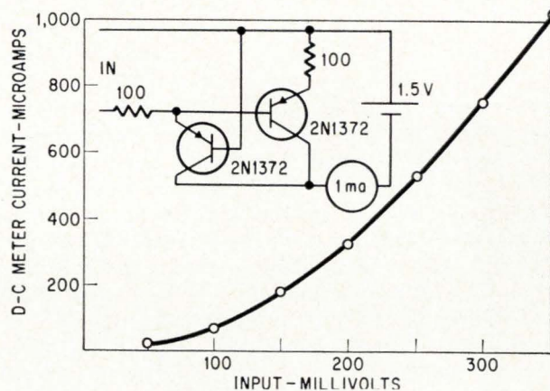
Milliohmmeter uses transistors as rectifiers with gain, permitting measurement of low values of a-c voltage.
