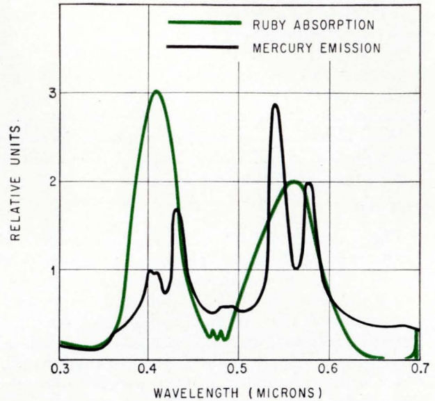
Absorption bands of ruby match very favorably the emission lines of the mercury-vapor flashtube. Peaks occur at almost the same wavelengths.
