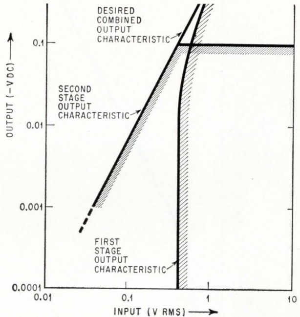
Output characteristics required to give a square-law device with a smooth transition between stages.
