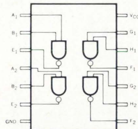
9002 Quadruple 2-input positive NAND gate.
