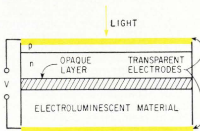
Electroluminescent panel, in cross section, from which a high-resolution paramosaic could be built.
