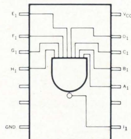
9007 8-input positive NAND gate.
