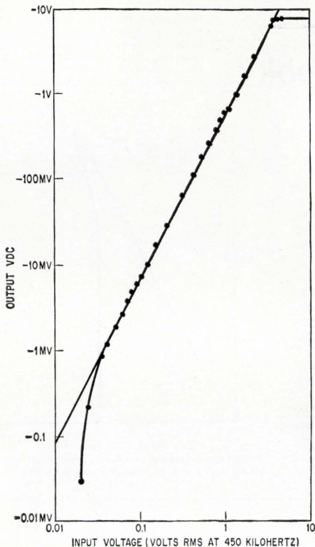
Measured output characteristics of the circuit operating with a 17-volt power supply. Adding stages extends the dynamic range on the low end without seriously affecting total accuracy. Greater accuracy is achieved by increasing the number of segments in each diode network.
