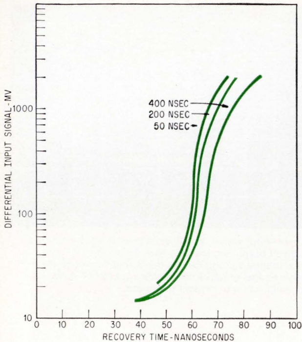
Recovery time depends both on differential overload and on pulse width, but is not seriously high even at inputs greater than a volt.
