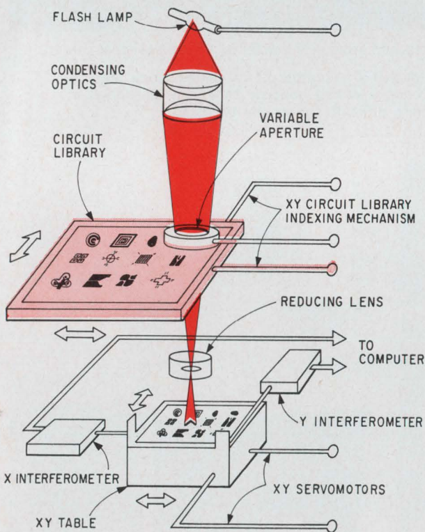
Mask-maker. Computerized artwork generator selects from circuit library the pattern to be flashed on high-resolution photographic plate. The xy table's position is controlled by the computer from information supplied by the interferometer. The xy drive for the circuit library moves by computer control to any of 49 discrete locations.
