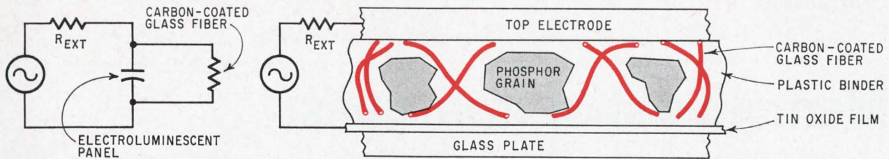
Placement. Electrically, an electroluminescent panel acts like a capacitor. To increase panel's impedance, carbon-coated glass fibers are placed in the dielectric, making contact with both plates.
