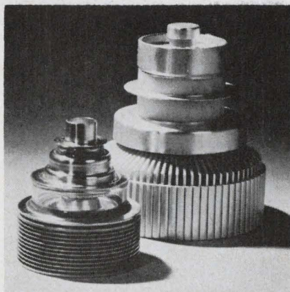
Passing it on. TH302, right, and TH328 amplify uhf signals at translator stations before retransmission.
