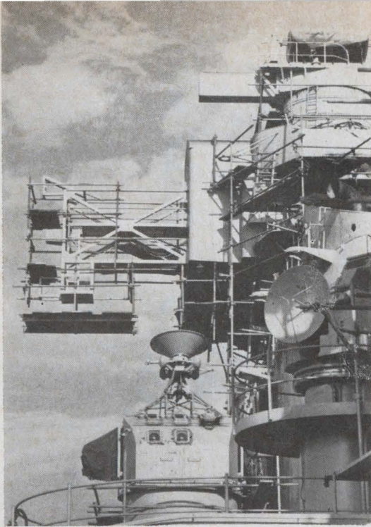
New. Electronic countermeasure gear goes in compartment, antenna on platform.
