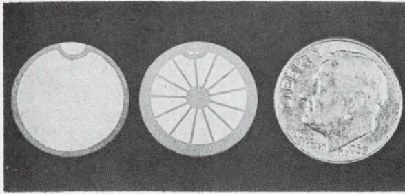
Ferroelectric pie. Costing only about a dollar, this little wafer can store a number and transfer it directly into an electronic counter. A voltage applied to the bottom layer bends it; the upper layer bends too, generating voltage pulses at the pie-shaped electrodes. Pulse polarity depends on previous polarization of the ceramic.
