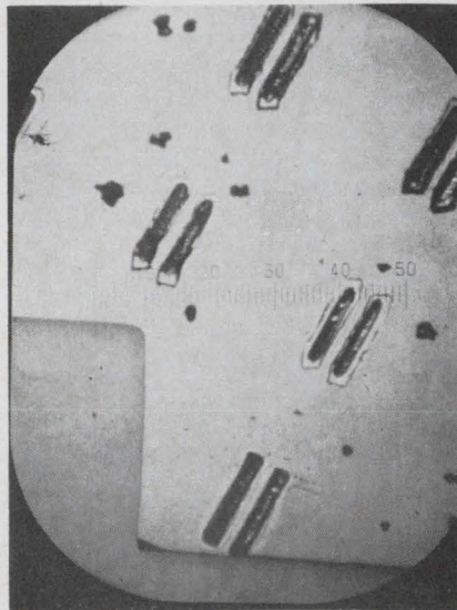
A sheet of Gunn devices. Higher microwave power is possible with better heat sinking.
