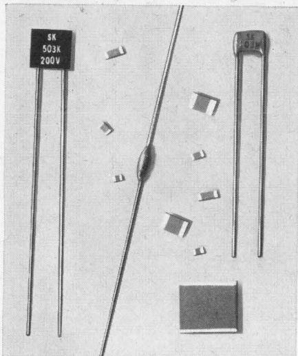
components and chips shown actual size
