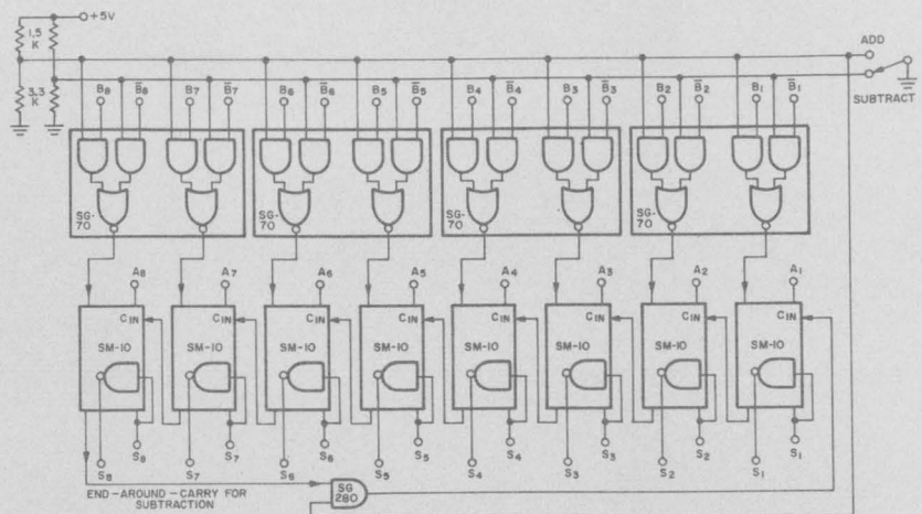
Figure 3. This parallel add/subtract configuration uses ripple carry propagation. This configuration will compute an eight-bit sum in approximately 135 nanosecs, or a difference in approximately 150 nanosecs. The SG280 dual 4-input AND/OR gate is enabled during subtraction to provide end-around-carry. The "B" register is made from only four SG70 Dual 2-Input AND-NOR Gates. Both the SG280 and the SG70 are standard SUHL gates.
