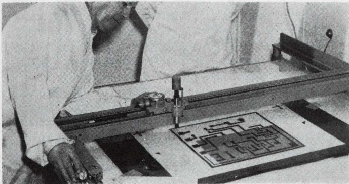
Large-scale drawing cut from rubylith . . .
