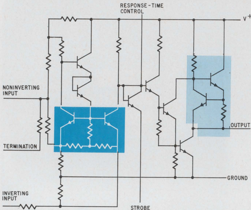
Better half. Common-base input stage and non-pnp-element, simulated output-stage current source help provide superior electrical performance in National's new dual line receiver. Only one side of the linear IC is shown.
