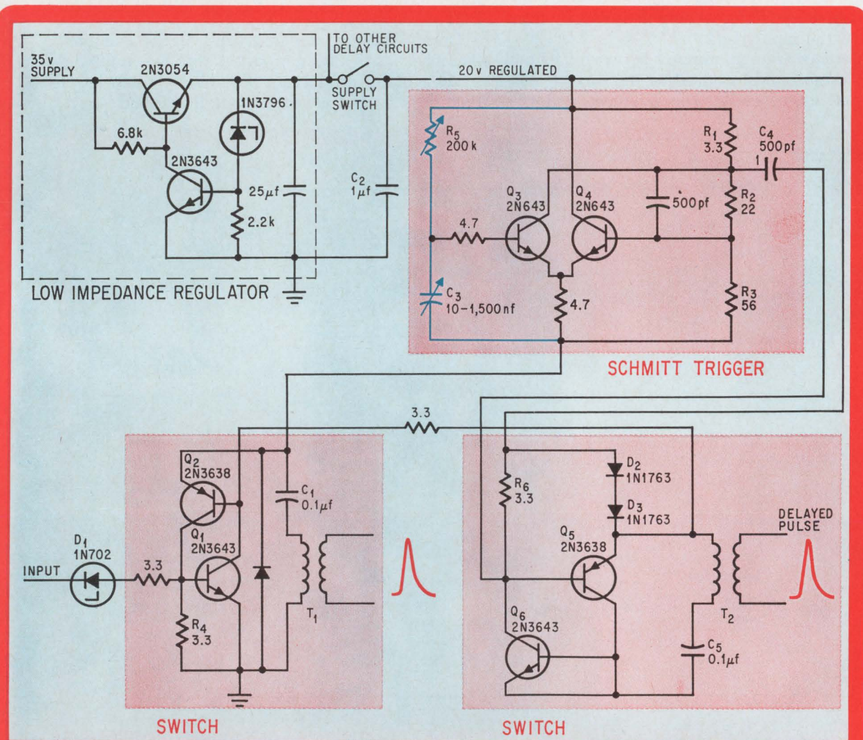
Delayed switch. Input pulse causes immediate conduction in transistors Q_1 and Q_2 , but has no effect on Q_5 and Q_6 until C_3 charges to a voltage that triggers Q_3 . The timer is reset when the switch is opened, stopping current flow through Q_2 and R_1 and removing the forward bias from Q_1 .
