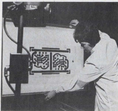
Scaled. Low-cost die stamping process for p-c boards begins with offset reduction of circuit's artwork.
