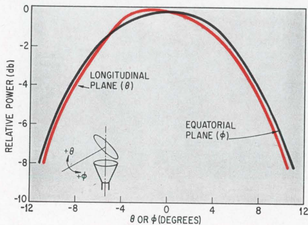
Planes in proximity. Antenna's radiation patterns for longitudinal and equatorial planes are within 0.3 db. Measurement frequencies are 3.7 GHz in transmit mode, left, and 6.425 GHz in receive, above.
