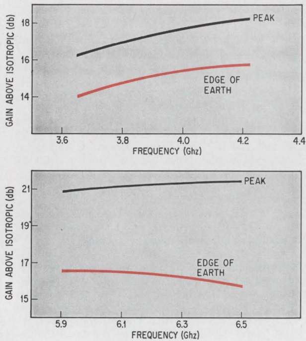
Big gain. Minimum edge-of-earth gain of 14.2 db across both transmit, top, and receive bands is well above the 13 db specified for the Intelsat 3.
