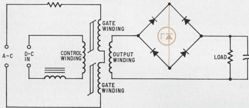
Circuit saver. One zener diode separates d-c control signal from a-c carrier in this magnetic amplifier that needs no external demodulator.
