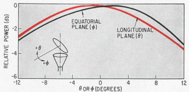
Planes in proximity. Antenna's radiation patterns for longitudinal and equatorial planes are within 0.3 db. Measurement frequencies are 3.7 GHz in transmit mode, left, and 6.425 GHz in receive, above.
