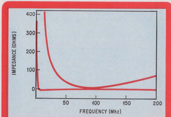
Showing up unknowns. The capacitor with its inductive leads resonates at about 90 Mhz. The inductive slope is due to the leads.
