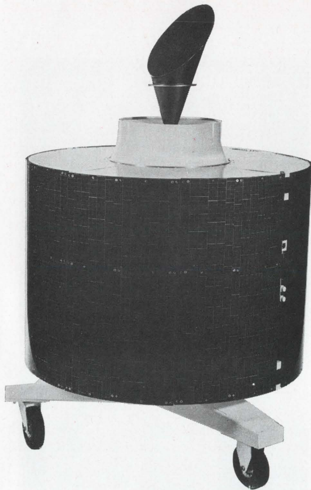
In-line. Mechanically despun antenna shown in mock-up, is mounted atop the Intelsat 3 communications satellite so that they both spin about the same axis.
