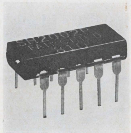
Junior size. Ten-lead hybrid is Fairchild's first plastic IC.
