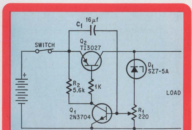
Circuit breaker. Series-transistor Q_2 is a low-resistance path for high battery voltage. Before full discharge, feedback opens circuit.
