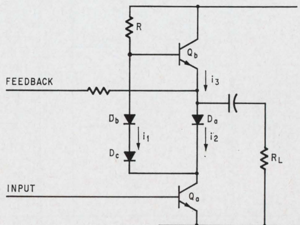
Basic audio amplifier. Output stage uses npn transistors and large negative feedback for good linearity.
