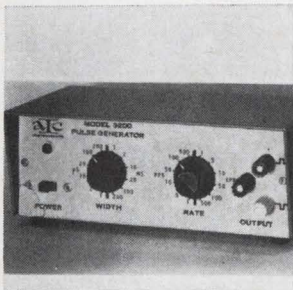
Pulse generator model 3200 has a crystal controlled clock and uses silicon transistors and DTL IC's throughout. Outputs consist of positive-going 0 to 5 v and negative-going 5 to 0 v pulse trains. Pulse width is switch selectable to 12 values from 1 \mu sec to 200 msec; pulse rate, in 12 rates from 1 to 500,000 pps. Price is $149. AIC Instruments, 6214 Royalton St., Houston. [369]
