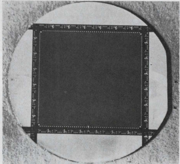
View. Monolithic germanium array, composed of 12,800 pnp transistors, was developed by Westinghouse as an infrared sensor. Scientists chose germanium over silicon, which is unable to detect in the 0.8-to-1.5-micron range. Work was supported by the Air Force.
