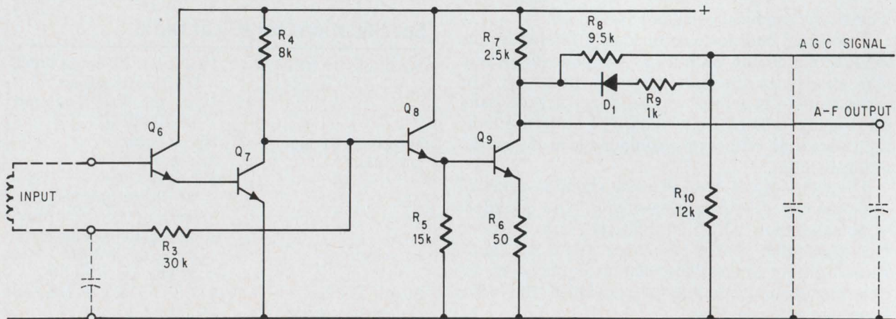
I-f amplifier and detector. Since most of the receiver's gain and all of the agc range are centered around stages preceding the i-f amplifier, the amplifier has been made simple to drive the low-level detector.
