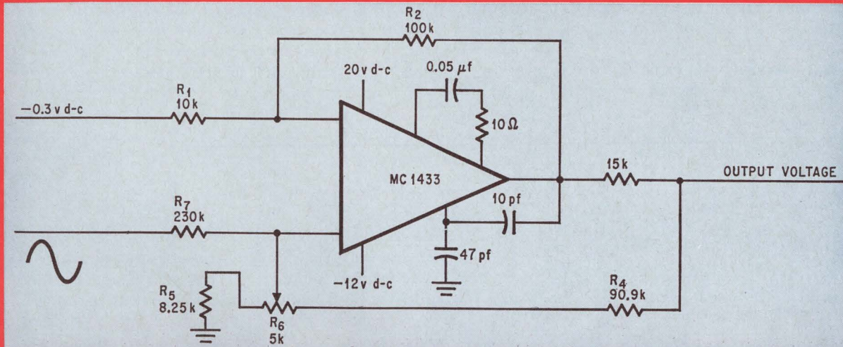
Constant current generator. The d-c input voltage—it is introduced at the point designated by 0.3v—changes level along with a-c signal at the non-inverting input. Consequently a varying d-c voltage is present at the output. The output voltage is used to modulate a double balance mixer.
