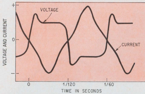
Design criteria. Voltage and current characteristics are selected to reduce the warm-up time of the bulb.
