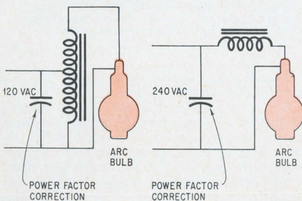
The old way. Conventional ballast consists of a large inductor and a power-factor correction capacitor.
