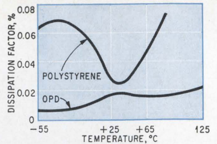
Flatter. Dissipation factor of polymer dielectric is always less than for polystyrene, and it varies less.
