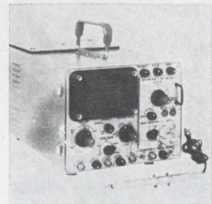
Explosion-proofed oscilloscope model K-106E can be used for on-the-spot check-out of electronic equipment at air fields and aboard ship where the use of high octane gas or the like creates danger of atmosphere ignition from electrical discharges or arcing. The unit is available in 7 or 10 Mhz bandwidth. General Atronics Inc., 1200 E. Mermaid Lane Philadelphia 1118. [376]
