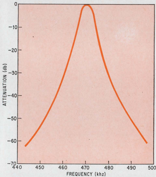
Selectivity curve. I-f filter selectivity curve has 1 db attenuation at \pm 1.6 kHz and 3 db attenuation at \pm 2.5 kHz.
