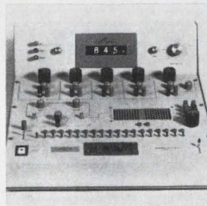
IC tester model 718 measures and displays with 3 decimal readout all important d-c parameters. Test connections and metering are made through a flexible programming matrix and lever switches which speed testing and reduce possibility of error. A built-in square wave generator provides dynamic inputs up to 10 Mhz. Microdyne Instruments Inc., Waltham, Mass. [373]
