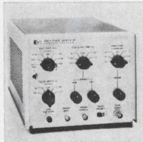
Variable rise- and fall-time pulse generator 8002A offers repetition rates from 0 to 10 Mhz, when controlled by external triggers, or from 0.3 hz to 10 Mhz with internal rate generator. Vernier control sets repetition rate anywhere within 30:1 range on any of the 5 ranges. Prices is $700; delivery, 4 to 6 weeks. Hewlett-Packard Co., 1501 Page Mill Rd., Palo Alto, Calif. [370]
