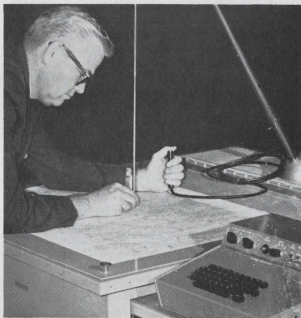
Tracing table. When graphic information isn't available on a slide the operator can trace the picture; the system automatically makes a slide.
