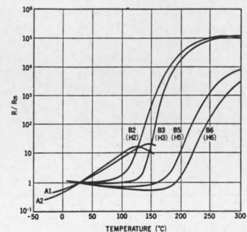
Temperature-logarithmic resistance characteristics of typical PTC-Thermistor.
