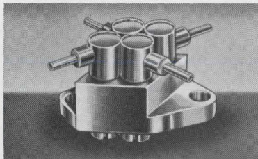
For coaxial applications, the above is a typical example of the metal blocks that can be supplied for simplified "high reliability" custom designs.
