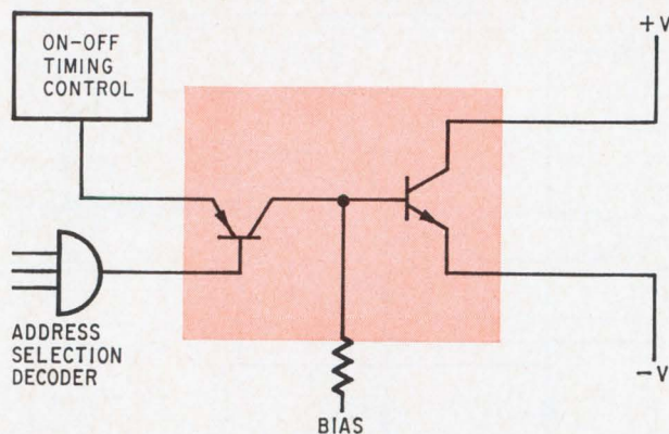
Memory driver. Here is an example of an interface circuit that connects to an IC at its input and provides high power efficiency at its output. Furthermore, it is easily packaged in large numbers on one substrate.
