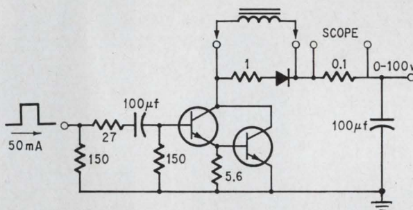
Tester. Simple di/dt measurements can be made with this, eliminating repetitive calculations.
