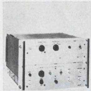
Real-time spectrum analyzer model SAI-21 provides complete capability for on-line analysis of voluminous data. It features an MOS shift register memory that eliminates drift and noise problems. The analyzer covers the frequency range from d-c to 1 Mhz, with 200-line resolution and 42-db dynamic range. Signal Analysis Industries Corp., 12 Di Tomas Court, Copiague, N.Y. [374]
