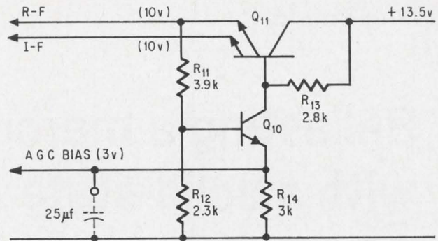
Supply decoupling. Extra decoupling between r-f and i-f is achieved by double-emitter transistor Q_{11} .
