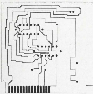
Figure D-14. Etching Master, Side 1
