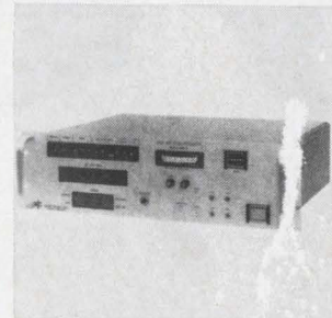
PCM bit synchronizer and detector model 830B is for the optimum recovery of data coded in any IRIG telemetry format. The design combines a second order phase-lock loop with detection circuitry that provides a bit error rate closely approaching the theoretical value for both negative and positive signal-to-noise ratios. Electrac Inc., 1614 Orangethorpe Way, Anaheim, Calif. [372]
