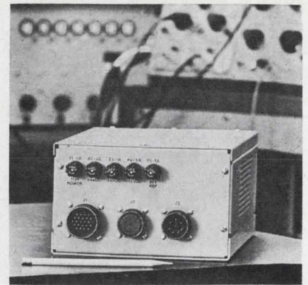
Tight packing. Built with MSI devices, the converter is the size of a shoebox.
