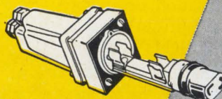
HGB-C panel mounted holder lamp indicating Military type FHL11U Single pole for \frac{1}{4} x 1 \frac{1}{4} in. fuses.
