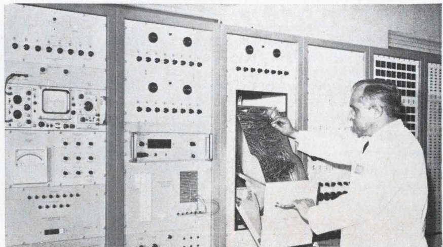
Sono buoni. Analog computer simulates what goes on in Italy's gas transmission network when the country's housewives attend to their spaghetti.
