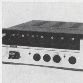
D-c voltage standard model 355 is 0.001% accurate. It has 10 ppm accuracy guaranteed for 30 days at standard reference conditions. Three decade ranges supply voltages from zero to more than 1,000 v with 7-place precision. Output current to 50 ma is available at any voltage setting. Price is $2,750; delivery, 60 days. Cohu Electronics Inc., Box 623, San Diego, Calif. 92112. [371]
