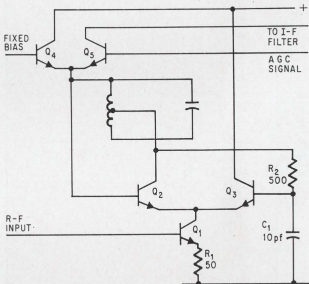
Self-oscillating mixer with agc. Designed for high conversion gain with low distortion, the mixer and agc unit can handle peak signals of over 100 millivolts.
