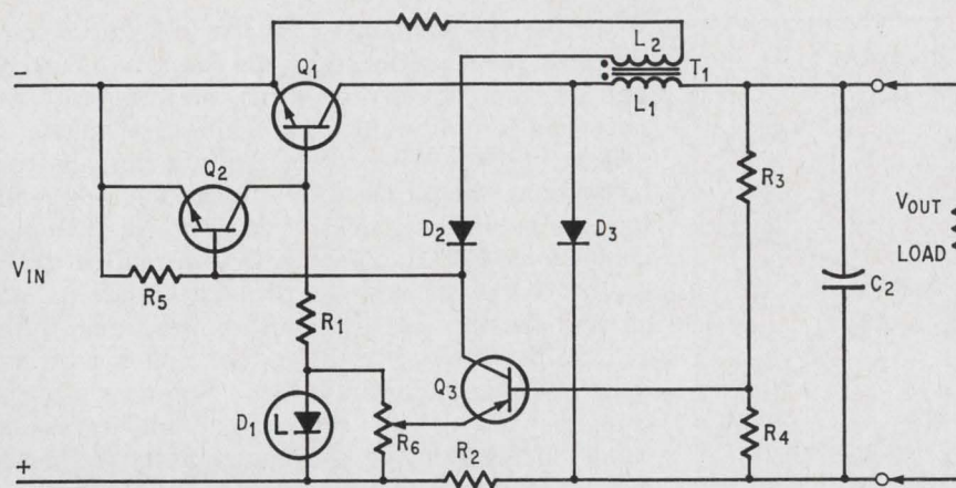
How it's done. The 120-volt switching regulator circuit monitors both current (through R_2 ) and voltage (through L_2 ) to keep the output at a constant level.
