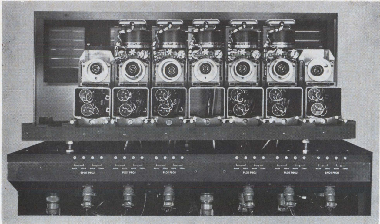
Blowup. Plotting, reference, and spotting projectors display variable and fixed information. Any of six colors can be selected by commands from the computer.
