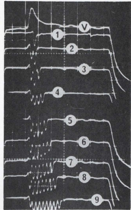
Fast count. The output pulses of a Gunn diode give a digital readout of analog voltage. An analog input pulse lasting 12 nanoseconds triggers the "9" reading at bottom.
