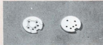
O. D. .367 \pm .003 Holes .041 \pm .002 Flat Within .002
