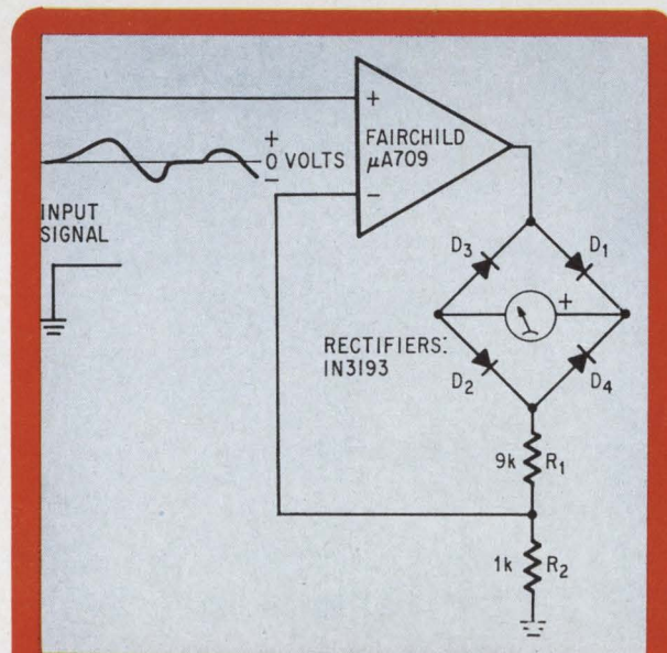
Accurate both ways. Variations in a voltage level are given meter-driven capability by the operational amplifier
