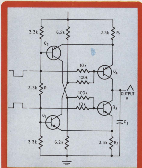
Sawtooth. Changing of capacitor C_1 by Q_4 's collector current forms the leading edge of the sawtooth.
