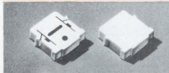
Width .420 \pm .003 Slot Width .015 \pm .003 Hole .021 \pm .001 Hole Spacing .372 \pm .002
