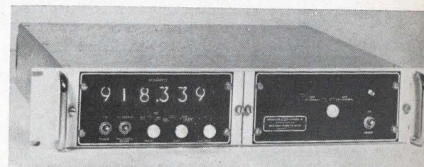
Stretchout. Extender, at right, pushes counter's range up another 700 Mhz.
