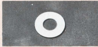
Metallized on O. D. I. D. .250 \pm .003 Thickness .018 \pm .001
