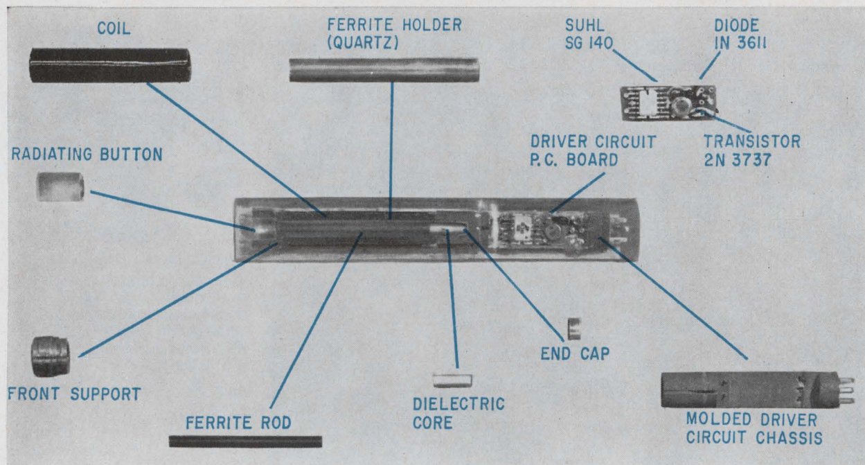
Piece by piece. Four-inch-long ferrite phase shifter for Raytheon's RARF antenna contains its own driver circuit and plugs into the face of the array.
