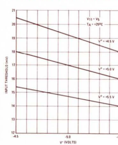
FIGURE 4 — TYPICAL INPUT THRESHOLD versus V -
