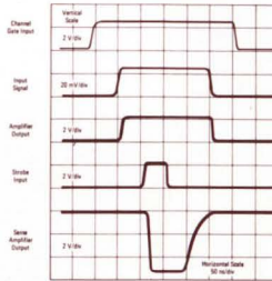
FIGURE 1 — TYPICAL OPERATION
