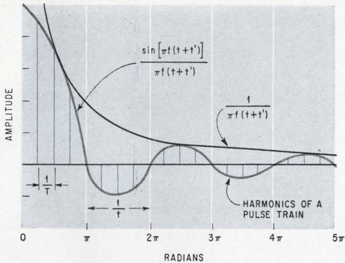
Spectral to broadband. The envelope of the maximum spectral lines, color, define the broadband spectrum, the black line. For convenience, the spectrum—approximated by three straight-line segments—is replotted in decibels and log frequency, right.
