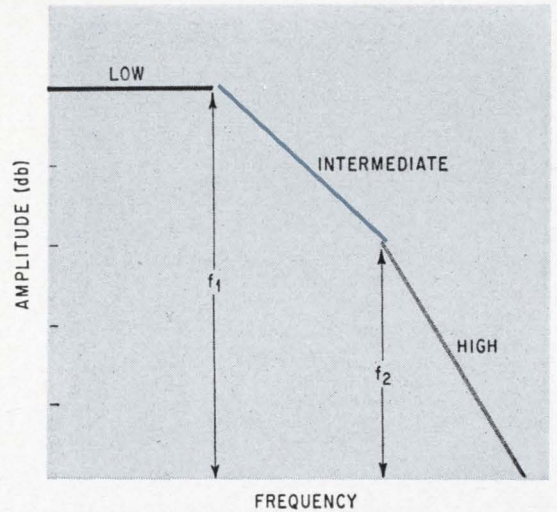
Spectral to broadband. The envelope of the maximum spectral lines, color, define the broadband spectrum, the black line. For convenience, the spectrum—approximated by three straight-line segments—is replotted in decibels and log frequency, right.
