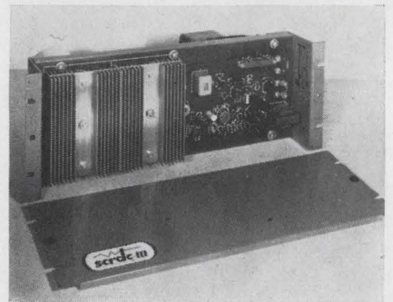
Checking out. The SCR's gate is fired by an error signal fed back from the power supply's output.
