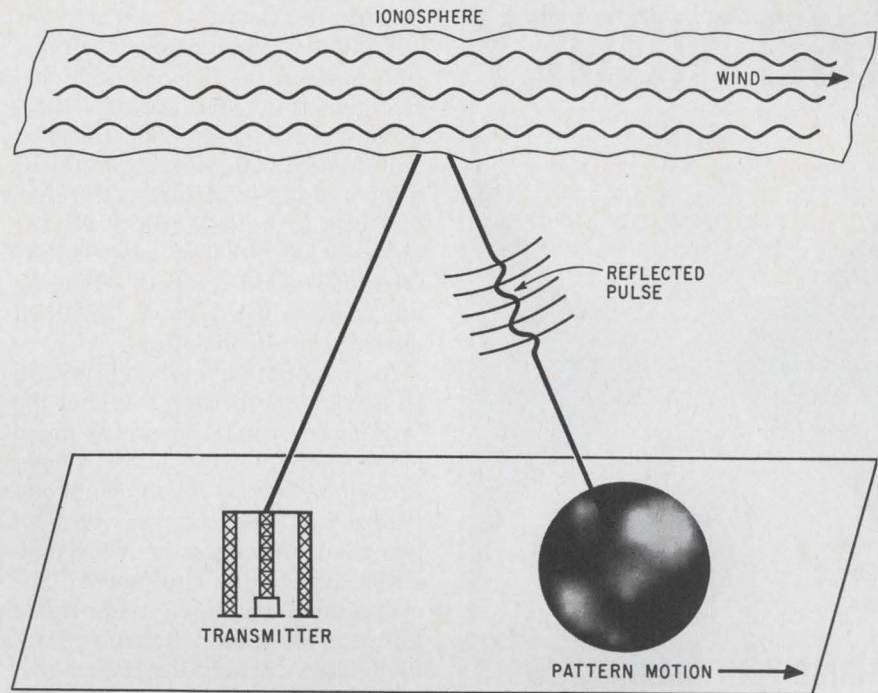
Light from above. The Australian system of measuring the speed and direction of the ionosphere's movement gives a visual picture when reflected pulse varies brightness of a light on the ground.
