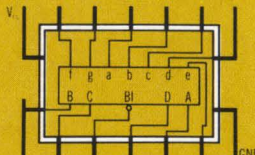
SN5449/SN7449 BCD-to-seven segment decoder-driver.
