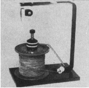
Combination dereeler and tensioner Mark 2 is for use on any type of coil-winding machine. It features a tensioning device that keeps the wire away from the spool flange. This eliminates kinking during dereeling. Constant positive action is easily adjustable for tension and wear. Price is $34.50. Excelsior Electronics Co., 7448 Deering Ave., Canoga Park, Calif. 91303. [418]
