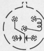
1 Form C, all contacts insulated from case
