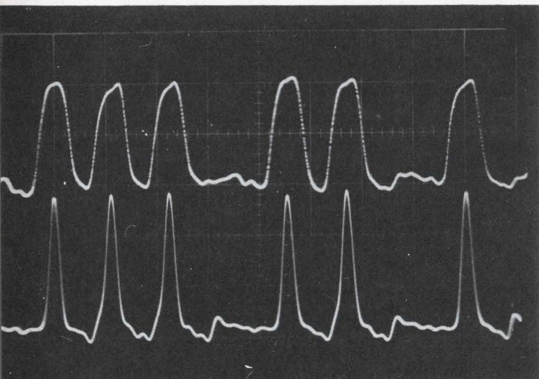
Conversion. Input electrical (224 megabit/sec) pulse stream codes output optical pulse stream.
