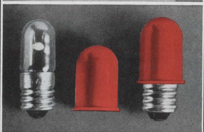
Light lookout. As long as all car lights are working, the magnetic field of the light coils is equal and opposite to the field of the ballast coils. When a light fails, a net field appears and the reed closes. The green lamp goes out and the red one glows.
