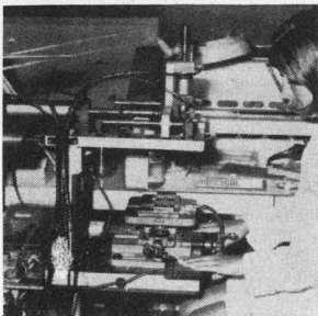
Bench model automatic screen printer, designated Accu-Coat model 3100, permits fine line metalizing (down to 0.004 in. line widths) using etched metal masks. The machine can be used for contact printing IC's. It accommodates masks or screens as large as 8 x 10 in. Price is $2,250; delivery, about 3 weeks. Aremco Products Inc., P.O. Box 145, Briarcliff Manor, N.Y. [422]
