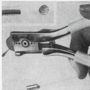
Wire and ribbon cutter called Square-Kut performs with equal efficiency on wire or tubing up to 0.0734 in. in diameter or on metal ribbon up to 0.025 in. thick and 0.125 in. wide. The smooth, flat-cut ends provided by the tool eliminate the need for secondary finishing on wires that are to be butt-welded or soldered. Henes Mfg. Co., 4301 East Madison, Phoenix, Ariz. [423]
