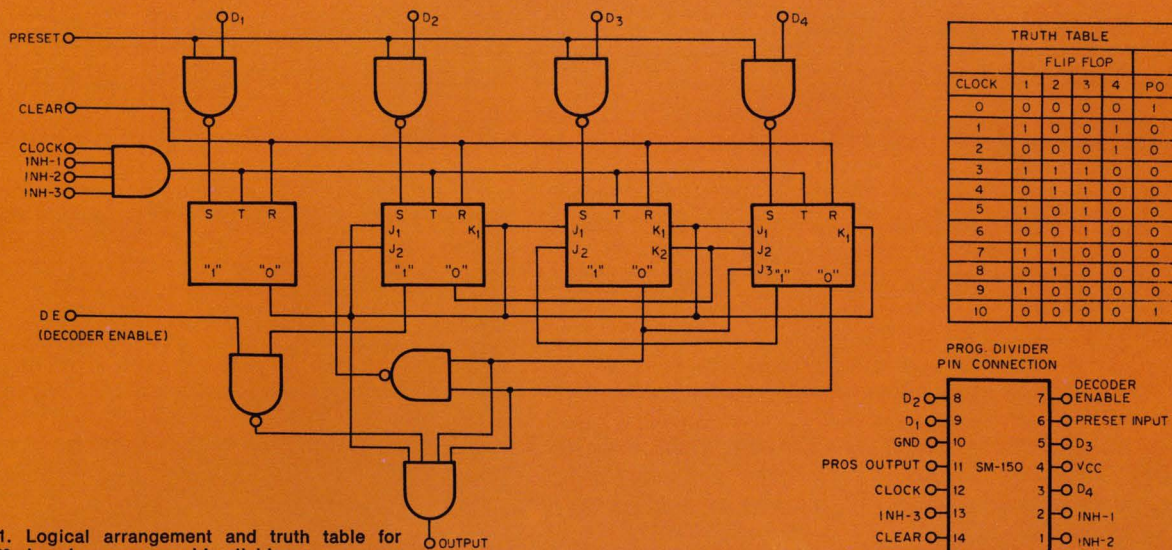
Fig. 1. Logical arrangement and truth table for SM-150 decade programmable divider.
