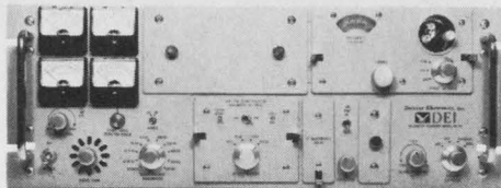
TR-711 . . . 55-2300 mHz tuning ranges. Solid state with switch selectable IF filters. All IRIG bandwidths. Plug-in record/playback converters, spectrum analyzer and oscilloscope.
