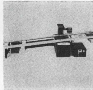
Wave soldering system handles any size p-c board and soldering circuit patterns from highly intricate to large ground areas without icicling or bridging. It includes a 10-ft anodized aluminum conveyor, a foam flux applicator, a pumping system that produces an infinitely variable solder wave from \frac{1}{8} to \frac{5}{8} in. high. Gale Systems Inc., 50 Main St., North Reading, Mass. [425]
