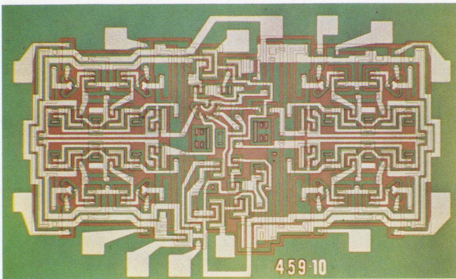
SM-130 comparator
