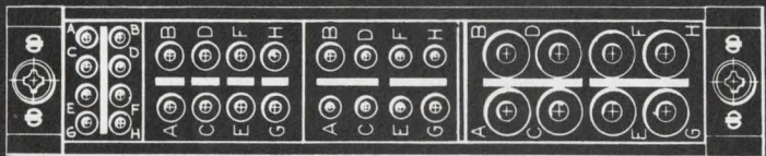
(below) Plan view of Sealok modules shows clear identification of contacts and bussing arrangements. Different bussing arrangements available in each module size.
