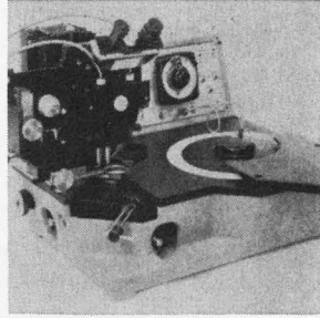
Optical mask alignment systems use fiber-optic light guides. Alignment of a semiconductor wafer to a mask and exposure of the wafer's photoresist coating are done semiautomatically in model 510 and manually in model 360. Both have lamp power of 200 w; UV reflectance of dichroic mirror, 98% or more at 4,000 angstroms. Electroglas Inc., 150 Constitution Drive, Menlo Park, Calif. [419]
