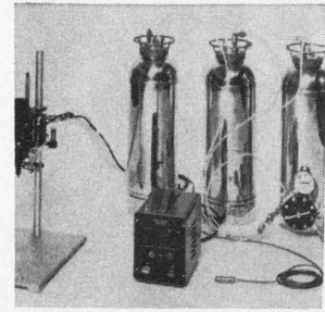
Processing equipment pots and encapsulates circuitry with foams, elastomers and solid resins. Output is up to 500 g/min. under continuous operation and 15 g/shot for single-cycle. Metering accuracy is better than 1% and ratio of components may be varied from 1:1 to 20:1 with max. viscosity of 20,000 centipoises. CBS Industries Inc., 2415 Campbell St., Oakland, Calif. [421]
