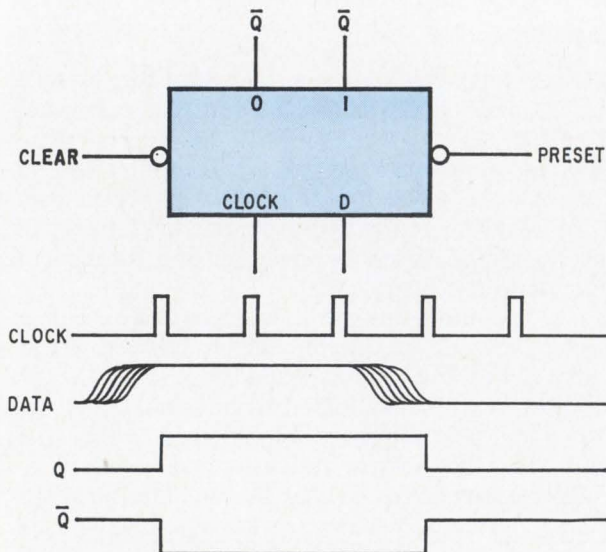
Logic configurations. All these gate forms are available in TTL circuits.
