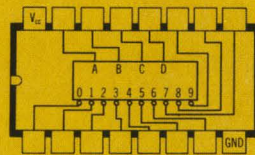
SN5444/SN7444 Excess 3 gray-to-decimal decoder.
