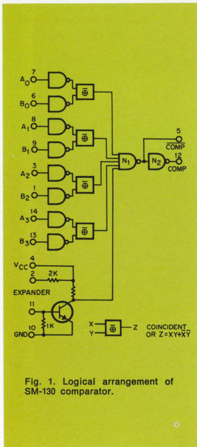
SM-130 comparator
