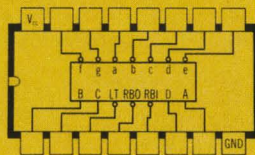
SN5446/SN7446 BCD-to-seven segment decoder-driver.
