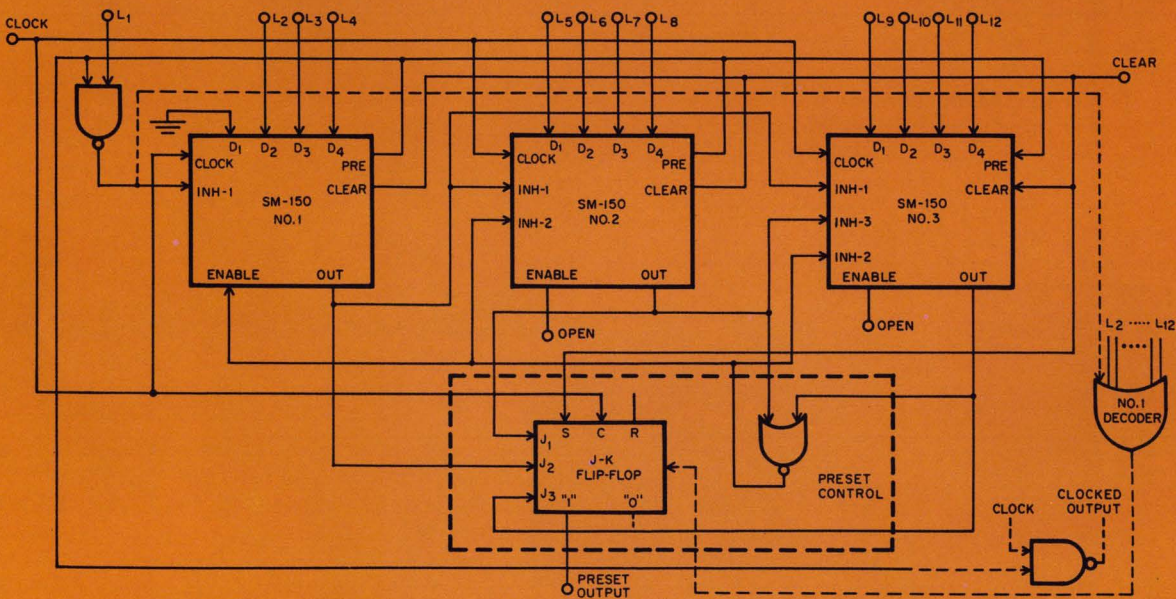
Fig. 2. 3-digit programmable divider.
