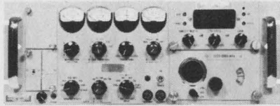
R-1074A-11 . . . 55-2300 mHz tuning ranges. Switch selectable IF filters and demodulators. Suitable for telemetry data reception and conical scan tracking. Automatic AFC reset carrier-operated relays.
