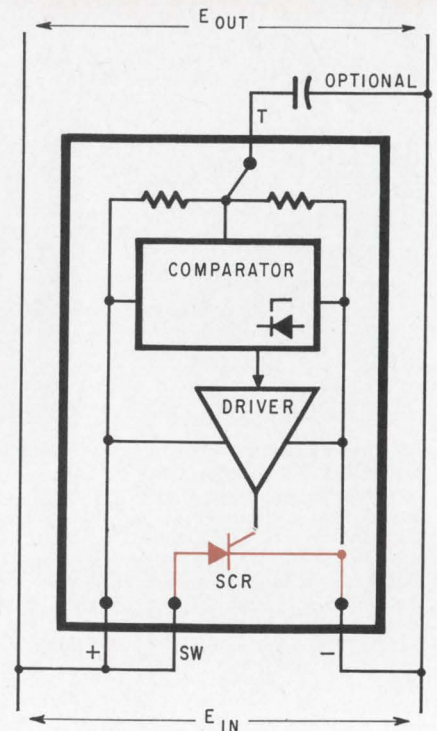
Protection. The thick-film crowbar is made for inputs up to 40 volts.
