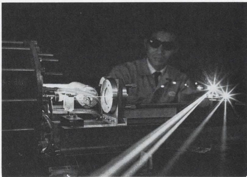
Turned on. A technician checks multicolored rays emitted by what Japan's Tokyo Shibaura Electric Co. says is the first long-life, high-output argon and krypton lasers made in Japan. They can oscillate over 11 wavelengths from blue to green; total output is one watt. Beryllium ceramics, rather than quartz, are used for the tubes.
