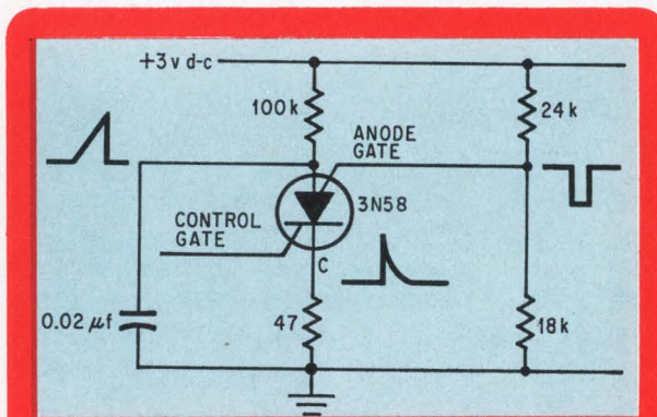
Switching oscillator. Compared with UJT versions, the SCS, with its simpler construction and lower dynamic resistance, yields a more efficient oscillator.
