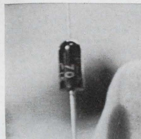
Plastic encapsulated zener diode BZX70 is a 2.5-w device. It measures approximately \frac{1}{2} x \frac{1}{4} in. with leads of just under 1 in., has a voltage range of 7.5 to 75 v. Surge rating is 100 w. As an aid to designers, the type number is clearly imprinted on the side. The devices are useful in communication and measuring equipment. Mullard Inc., 100 Finn Court, Farmingdale, N.Y. [439]
