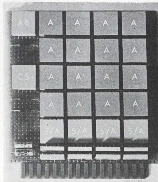
Modular. Cogar's "Mind Jogger" memory subsystem has a highly modular organization. Modules labeled A contain the memory arrays. AB represents an address buffer, CS is the chip-select module, and S/A indicates sense amplifiers. Capacitors and terminating resistors are located at the bottom of the card.
