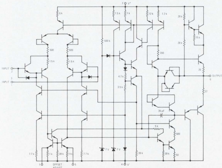
CIRCUIT SCHEMATIC
