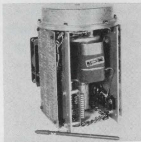
Disk memory system series 8100 has been developed to fit the mini-computer market segment that requires a combination of a compact and lightweight package with a bit storage capability approaching 145 K bits of storage. Package is 9 x 9 x 10½ in. Access time is 8.5 msec utilizing TTL interfacing. Information Data Systems Inc., E. Eight Mile Rd., Detroit, Mich. [363]
