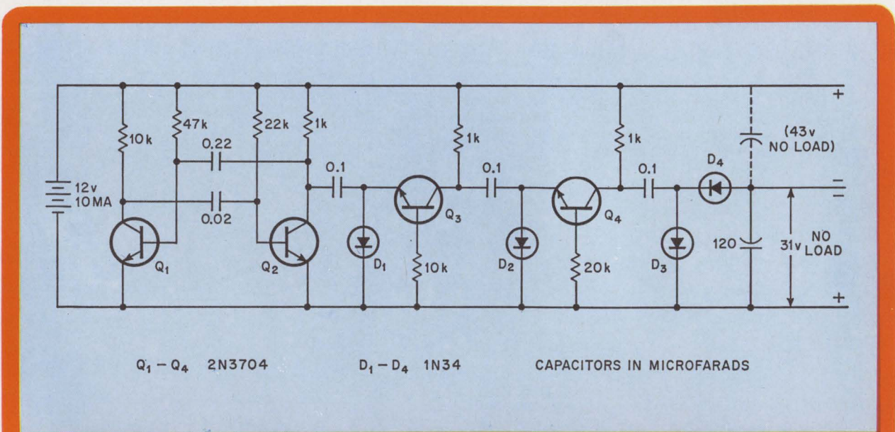
Series-aiding. When transistor Q_2 is off, the three 0.1-microfarad capacitors charge to the supply voltage. On the next multivibrator cycle, Q_2 turns on, also turning on transistors Q_3 and Q_4 . The three capacitors, now in series, unload their charge on the 120- \mu f output capacitor which charges to triple the supply voltage.
