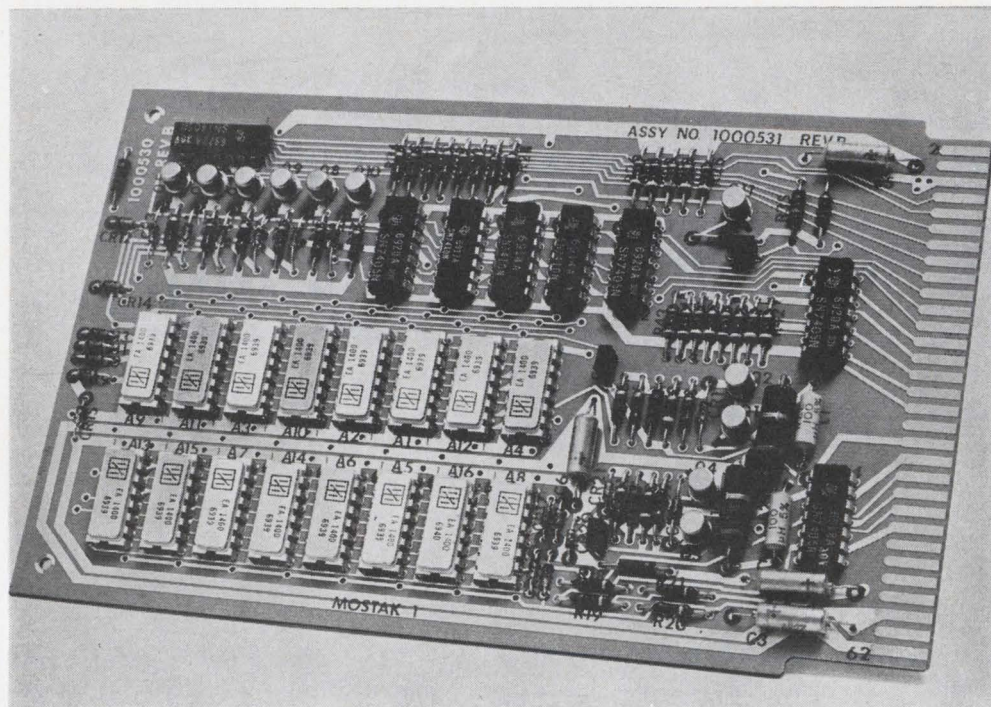
Subsystem. A popular approach to the semiconductor memory market is to manufacture a complete memory subsystem on a card, suitable for use as a scratchpad or buffer memory. The Mostak I random-access read-write memory, for example, manufactured by Electronic Arrays Inc., employs 16 MOS chips, each with 128 bit capacity.
