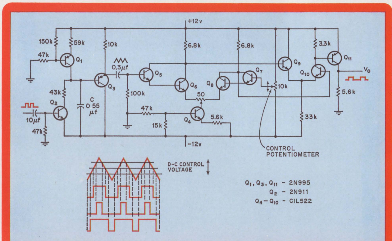
Modulator. A triangular waveform feeds one input of comparator Q 5 -Q 8 while a d-c voltage adjusted by the 10-kilohm pot feeds the other. When the d-c voltage exceeds the triangular voltage, Q 10 and Q 11 are off and the output is 0 volts. When the reverse occurs, Q 10 and Q 11 conduct and the output rises to 12 volts.
