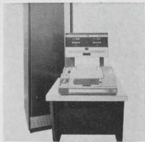
Algomatic 16 is a direct digital control and data handling system providing closed-loop control and data logging for 16 loops, expandable in 16-channel increments up to 128. Through its software, it processes the loop data using a control algorithm tailored to each loop. Data logging may be either full time or only for off-limit values. Research Inc., Box 24064, Minneapolis [361]
