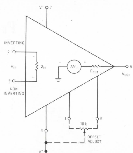
EQUIVALENT CIRCUIT
