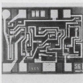
Voltage regulators SG105-205, and -305 feature output adjustable from 4.5 to 40 v, load regulation of better than 0.01%/ma and line regulation of better than 0.06%/v. With an input voltage of 50 v, they deliver loads up to 20 ma. The SG105 operates from -55^{\circ} C to +125^{\circ} C; the 205 and 305, from 0^{\circ} to +70^{\circ} C. Silicon General Inc., 7382 Bolsa Ave., Westminster, Calif. [442]
