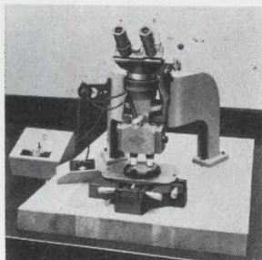
Zero-backlash instrument provides fast, foolproof microinch alignment of masks to wafers prior to exposure. This positioning is in all three axes (X, Y, and angle). Microinch movements can be made while observing mask and wafer positions through a dual-objective microscope. Each objective can be focused independently. The Jade Corp., Philmont Ave., Huntingdon Valley, Pa. [422]
