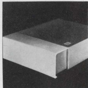
Parallel-input simplex modem 402C accepts 5, 6, or 8-level tape reader inputs and converts the data to parallel tones for transmission over the public telephone network. The modem is used in data collection systems and can be adapted to most parallel information applications. It operates at a speed of 75 characters/sec. General Data Comm Industries, Norwalk, Conn. [366]
