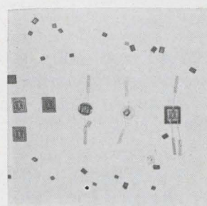
Silicon planar power transistors come in chip form for hybrid applications. Chips include the 2, 5, 10 and 20 amp families in npn, pnp and npn high voltage. In addition to their individual chip form, they may be mounted on a moly-tab or on moly pedestals with aluminum wire leads ultrasonically bonded to emitter and base contacts. Solitron Devices Inc., Riviera Beach, Fla. [443]
