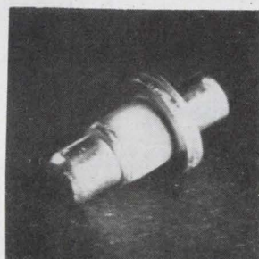
High power p-i-n diodes feature high dynamic Q switching in less than 300 nsec, high power handling capability, oxide and hard glass passivation, low C_T and high storage and operating temperature range. Units are recommended for use in r-f switching, limiting, phase shifting, duplexing and attenuating through Ku band. Microwave Associates Inc., Burlington, Mass. [441]
