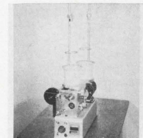
Front-loading bobbin winder model CHM-2 is a two-spindle machine. Infinite traverse adjustment is possible through a direct action adjustable cam. The machine combines automatic overrun compensation with automatic positioning of the guide for the start of the next coil without operator attention. Coil Winding Equipment Co., Railroad Plaza, Oyster Bay, N.Y. 11771 [428]
