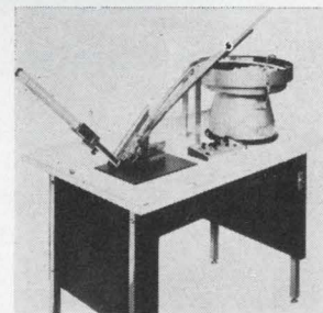
Dual in-line package insertion machine SM-2000 accepts DIP's from "sticks", loads them into carriers, and stacks the loaded carriers into magazines for further automated processing. It runs at rates up to 3,600 pieces per hour. Except for manual loading of carriers and DIP circuits, it is fully automatic. Weltek Div., Wells Electronics Inc., S. Main St., South Bend, Ind. [424]
