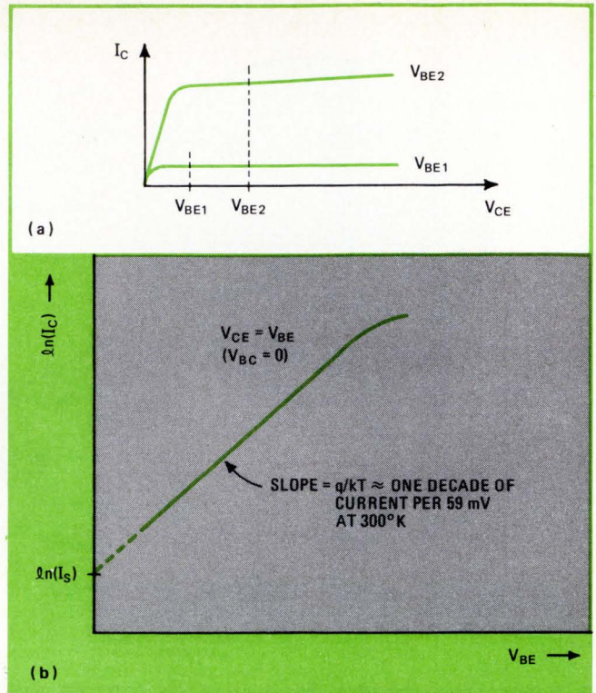
7. Determining saturation current. Parameter I_S (saturation current) is the third parameter that must be measured. It is a constant that can be computed from a single-point measurement of I_C at a constant V_{BE} value of V_{BE} = V_{CE} so that V_{BC} = 0 . The curve-tracer display of (a) shows I_C versus V_{CE} for a fixed V_{BE} . The value of I_S can also be extrapolated from a plot (b) of \ln(I_C) versus V_{BE} .
