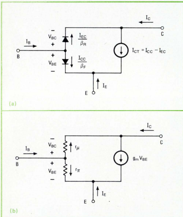
4. Changing model form. The nonlinear hybrid- \pi model of (a) is obtained by consolidating the two reference current sources of the transport model (Fig. 2b). The change in model form is strictly a matter of convenience. When the nonlinear hybrid- \pi model is linearized for a small-signal analysis in the forward active region, it easily reduces to the well-known linear hybrid- \pi model of (b).
