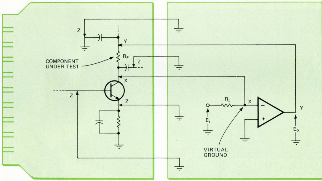
PRINTED-CIRCUIT BOARD
