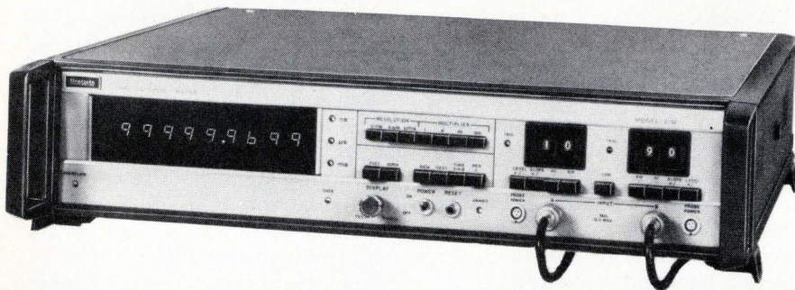
Debut. Femtosecond resolution of new time interval counter from United Systems Corp. should be useful for fusion lasers and in the design of high-speed logic families.
