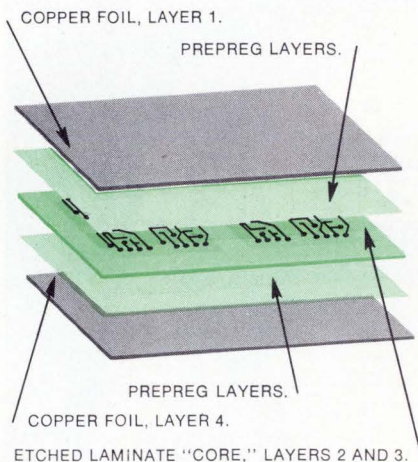
Typical Micapak™ multilayer "blank" (as large as 24" x 36") before lamination. Inner laminate is etched with both sides in registration to each other.
