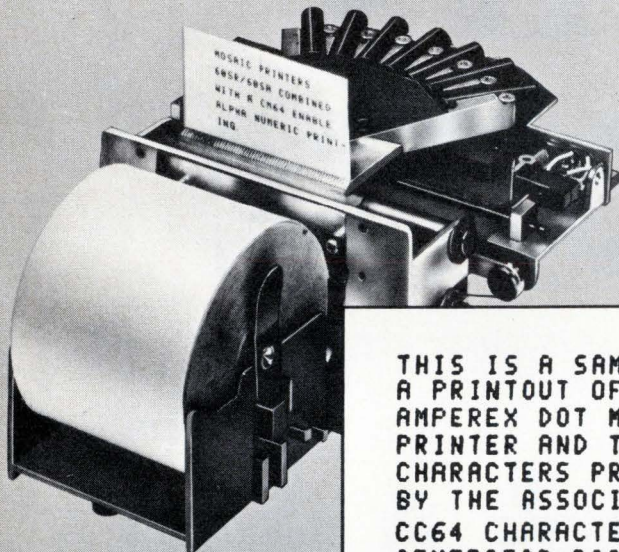
MODEL 60SA
