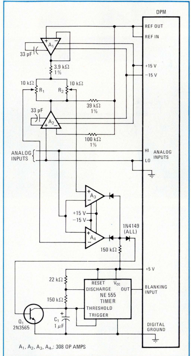
Limit checker. Potentiometers define upper and lower thresholds for permissible range of analog signal. When input is above or below the threshold range, the timer, connected as an astable multivibrator, begins to flash either the entire display or its polarity sign.
