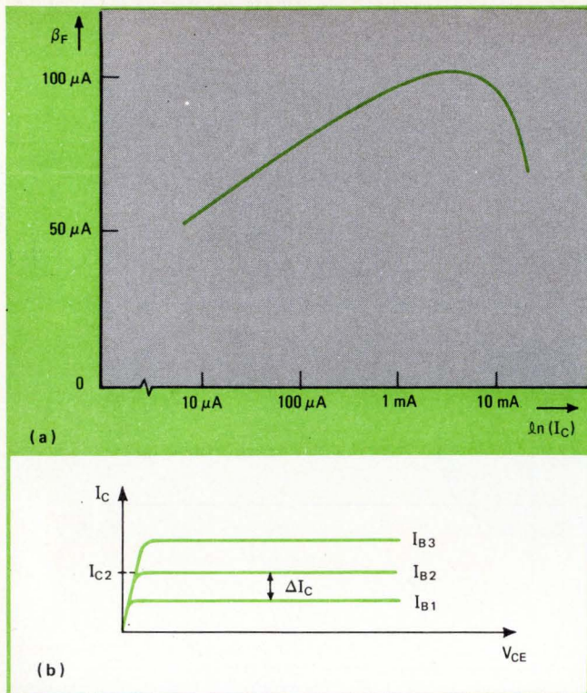
6. Determining the current gains. Parameters \beta_F (forward beta) and \beta_R (inverse beta) are two of the three parameters that must be measured to specify the first-level Ebers-Moll model. Although \beta_F typically varies with collector current, as shown in (a), it is assumed to be constant for this level of model complexity, as in \beta_R . The dc values of both betas can be obtained from the collector characteristics.
