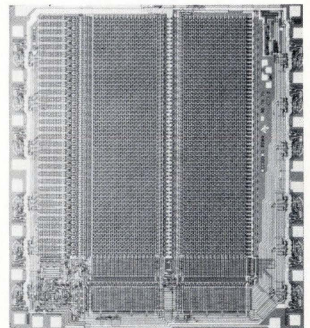
Remembering. The 4-k RAM comes in two pin configurations: the 16-pin version, such as Mostek's (top), and the 22-pin, an example of which is the Texas Instruments chip that is shown above.
