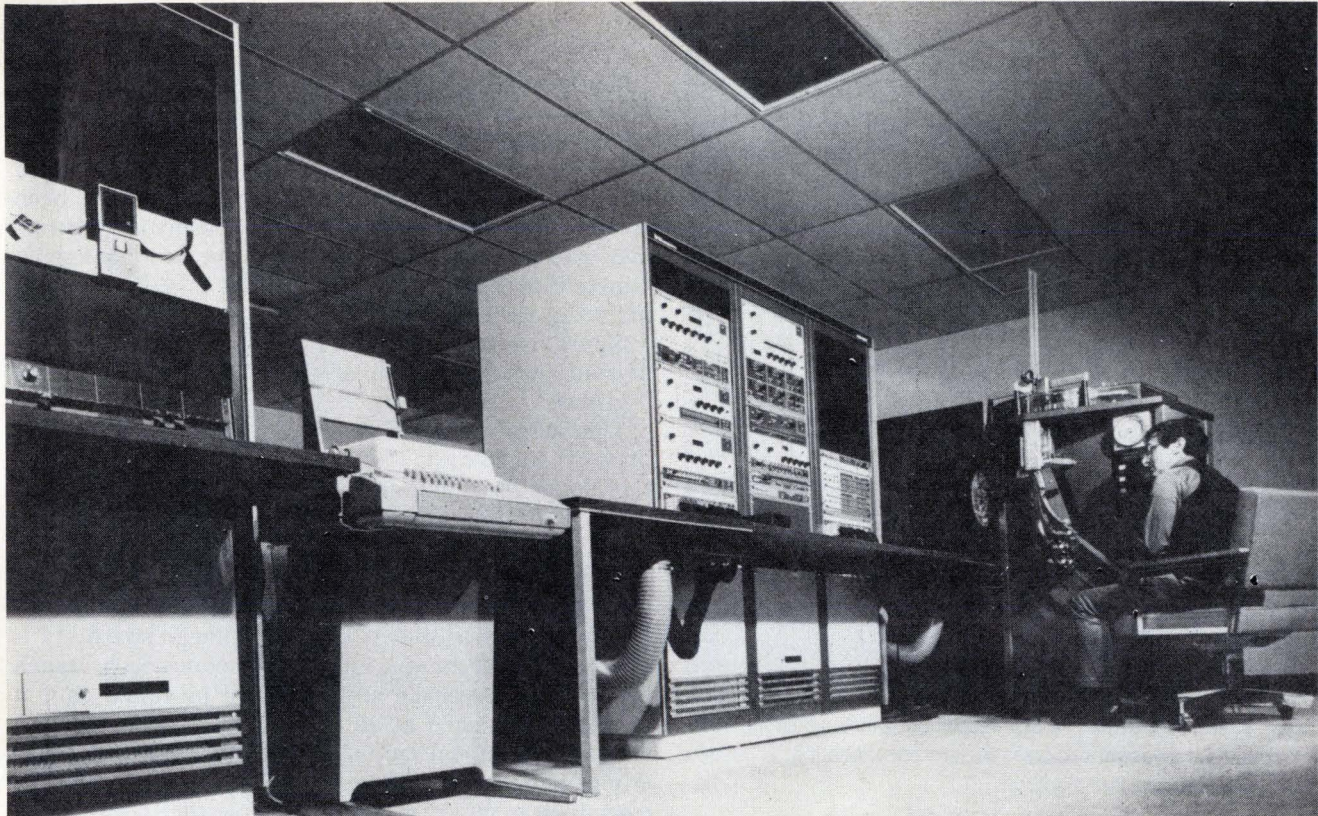
4. Diagnostic dreadnaught. Macrodata's MD-500 diagnostic-test system is designed to perform digital functional and parametric testing of bipolar and MOS LSI devices at data rates as high as 10 MHz. Parametric and functional testing may be performed simultaneously. Its compiler-based operating system can perform a number of tasks simultaneously, such as operating two test stations in parallel and compiling.
