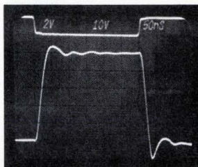
NON-COMPENSATED 10V/V GAIN STABLE INVERTING ONLY
