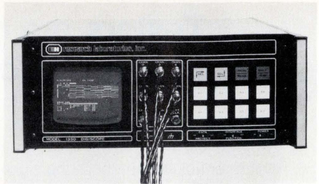
2. Time check. Either a timing diagram or the equivalent binary representation of the activity on eight signal lines may be displayed on E-H Research Laboratories' model 1330 Digiscope. The instrument is controlled by a National SC/MP microprocessor.
