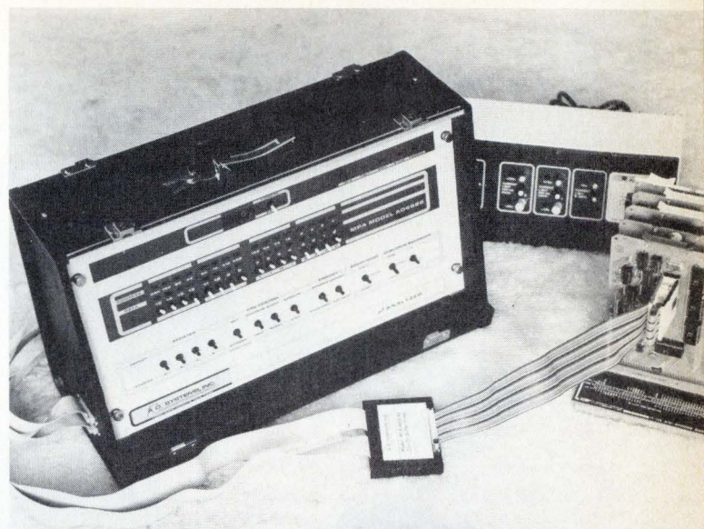
10. Independent. Connected to a microprocessor by a three-state buffered probe, the AQ6800 allows a designer to monitor the system under test and to deposit information into memory and registers without tying up interrupts or memory space.
