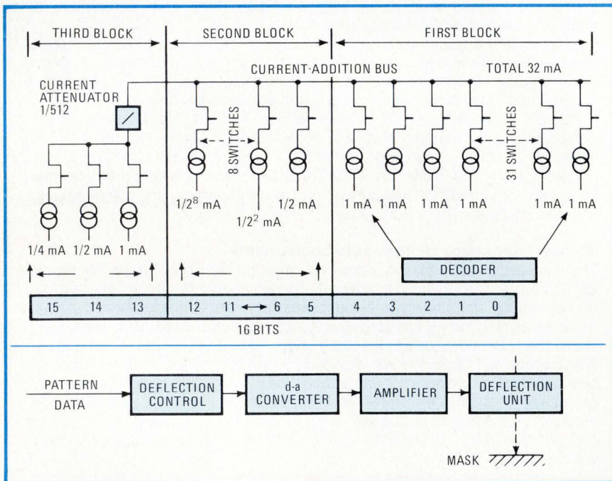
Exposure resolution. Heart of the NTT electron-beam exposure system is high-speed 16-bit digital-to-analog converter (top), which positions exposure points 0.03 micrometer apart. Controlled by patterns stored in computer memory, the system (below) consists of the deflection control, d-a converter, amplifier, and deflection unit.
