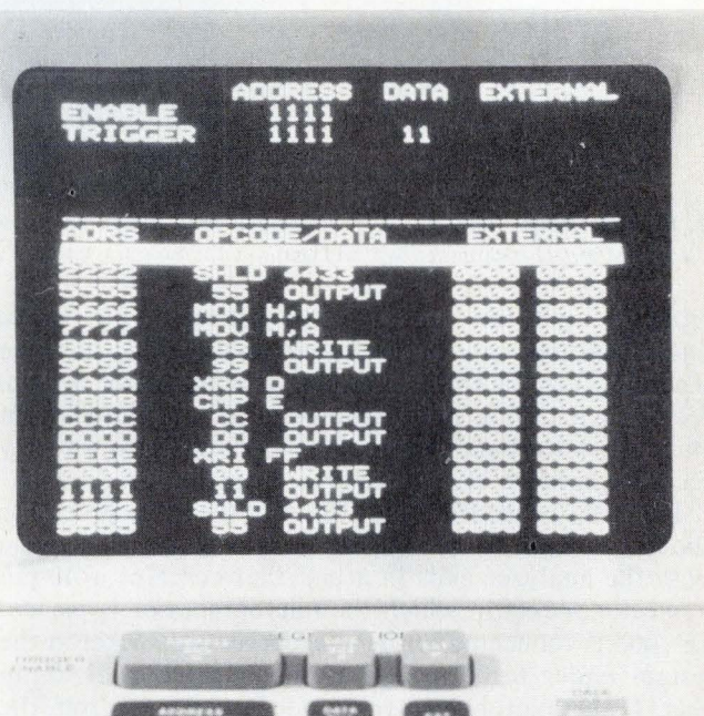
11. Convenience. Along with extensive triggering modes, Hewlett-Packard's 1611A microprocessor analyzer can convert binary information at its inputs into the alphanumeric mnemonics of an 8080- or 6800-type microprocessor's instruction set.
