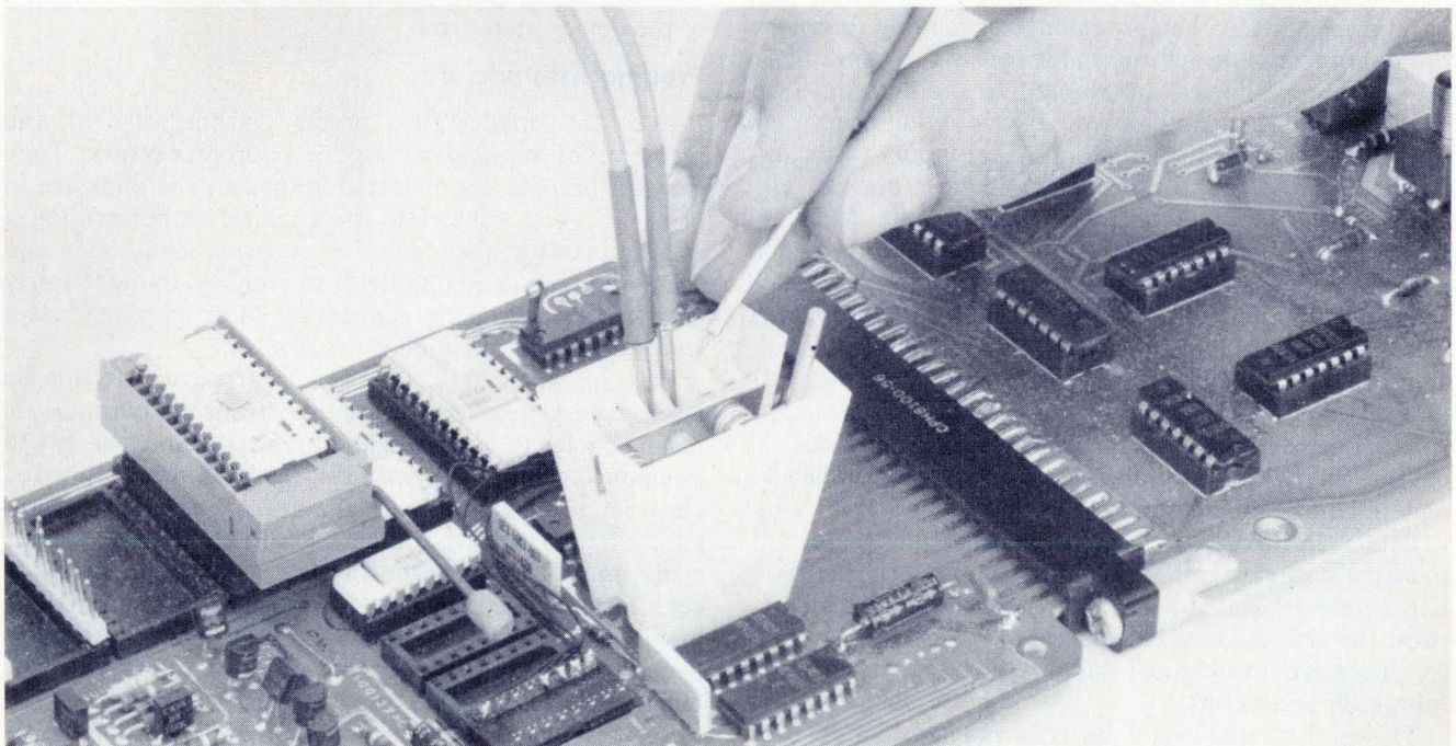
6. Contact housing. A metal pin through this HP test clip contacts an IC's ground pin and the clip's ground plane. With their grabber-hook tips removed, probes can then be inserted into the housing, connecting to both the IC pin and the ground plane.
