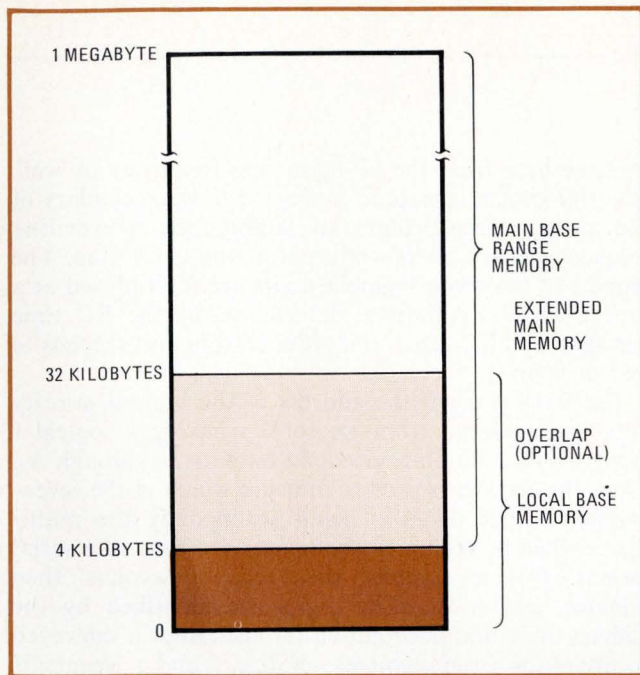
4. Offset. For the base-adder scheme, an offset address is loaded into a base register, the contents of which are then added to the local address bus to generate a 20-bit extended address. Local memory, however, is addressed by the microcomputer's 16-bit bus.
