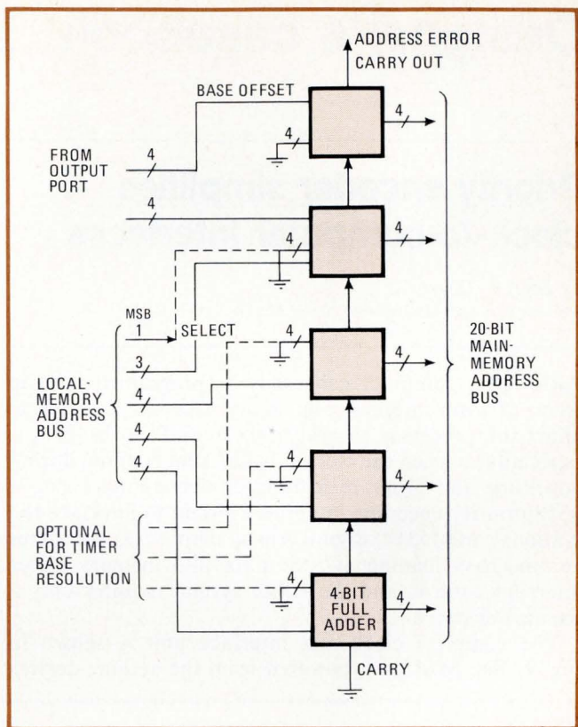
5. Quad adders. In base addition, the base offset value is added to the contents of the address bus by five quad adders. In this example, the most significant bit of the address bus is used to signify that main, not local, memory is to be accessed.
