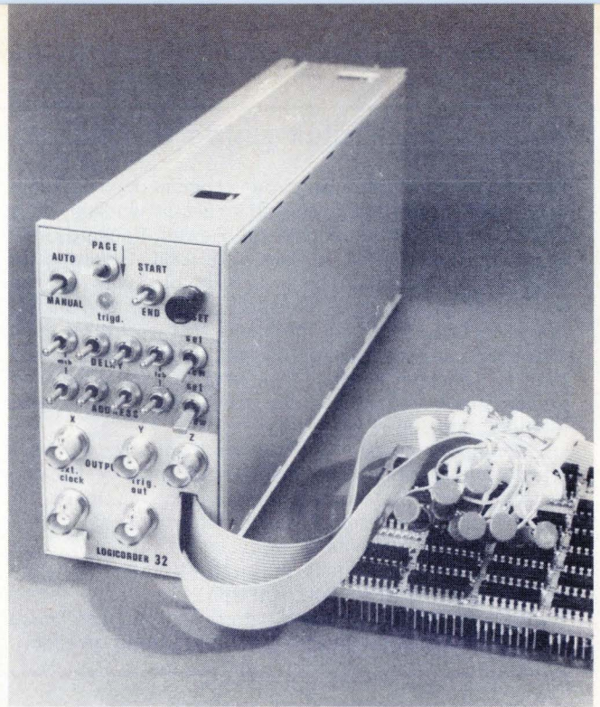
5. Cost-cutting. The Logicorder 32 microprocessor analyzer from Scanoptik is an inexpensive instrument that monitors up to 32 signal lines. It can capture and display data on an external oscilloscope screen in hexadecimal notation.
